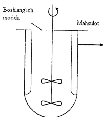
1.3 rasm. Ideal aralashtirish modelini amalga oshiruvchi apparat sxemasi
