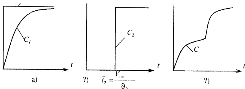
2.32-rasm. Ideal aralashtirish va ideal siqib chiqarish sohalarining parallel ulanishidan tuzilgan tizimning pog'onali g'alayonga javobi: a - ideal aralashtirish sohasining javobi; b - ideal siqib chiqarish sohasining javobi; v - tizimning javobi.
