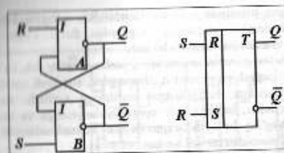
8.2-rasm. Triggerning ish sxemasi.
