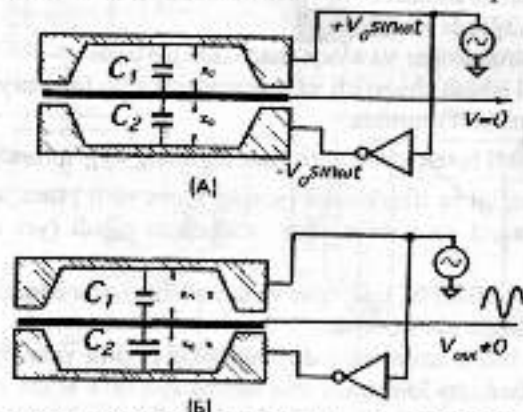
2.30-rasm. Tekis plastinkali sig'im datchigini ish prinsipi:
