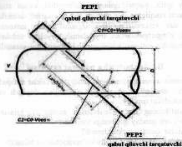
2.43-rasm. Ultratovushli o'zgartirgichning prinsipial sxemasi.
