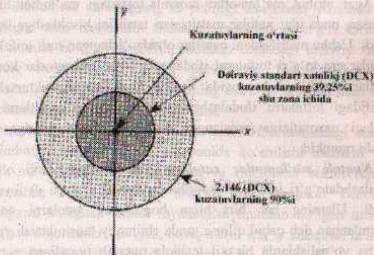
7.1-rasm. Dairaviy standart xatolik
