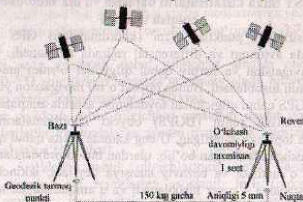
3.8-rasm. Statika usuli
