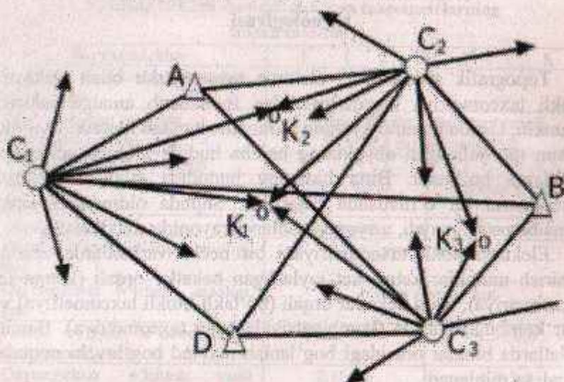
2.8-rasm. Ozod bekatlar taxeometriyasini bajarish sxemasi
