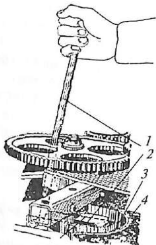
27-rasm. Shpindellarni teskariga aylantiruvchi kolodkani barabandan ajratib olish:
