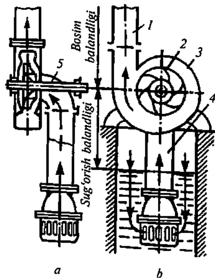
58-rasm. Markazdan qochma nasos:
