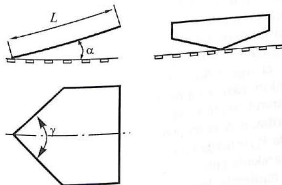
46- rasm. Yassi uchburchak lemex.
