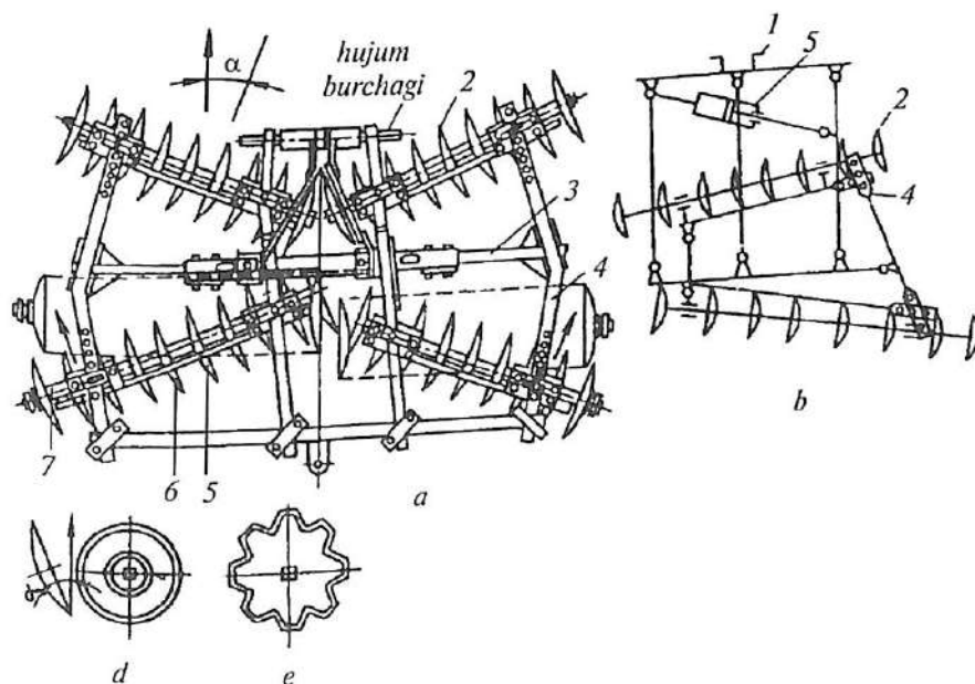
9- rasm. Disksimon borona.
