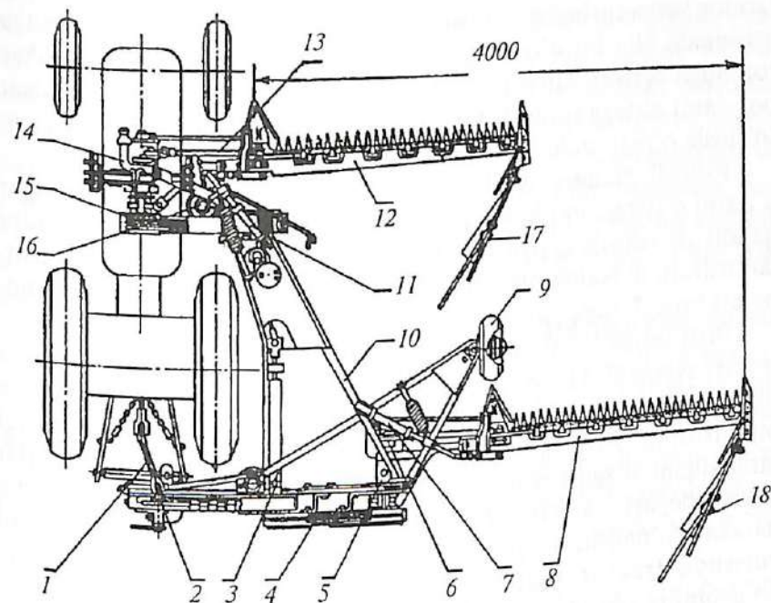
37- rasm. Qo‘sh brusli yarim osma pichano‘rgich.
