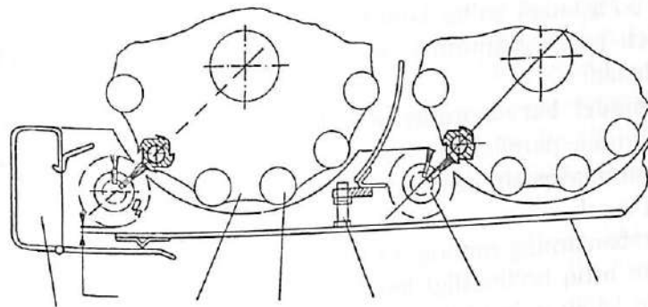
24- rasm. Ajratgich va apparat eshigi xolatini rostdash.
