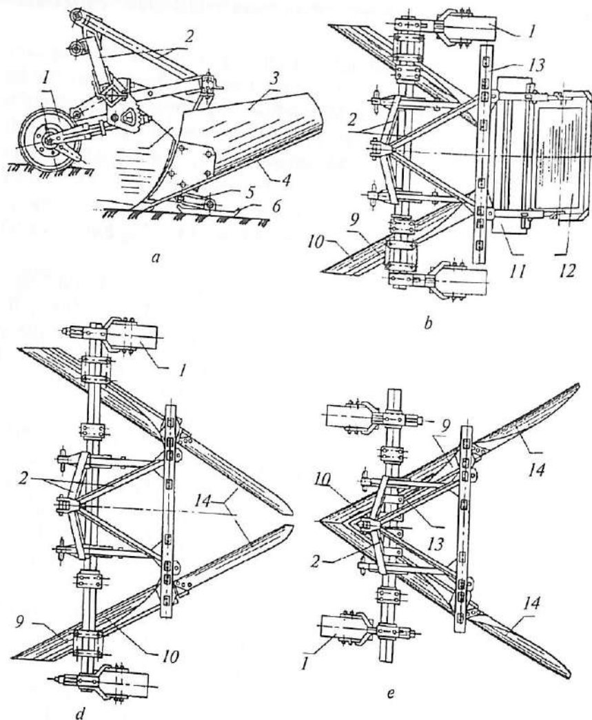
54-rasm. Universal ariq qazgich-tekislagich.
