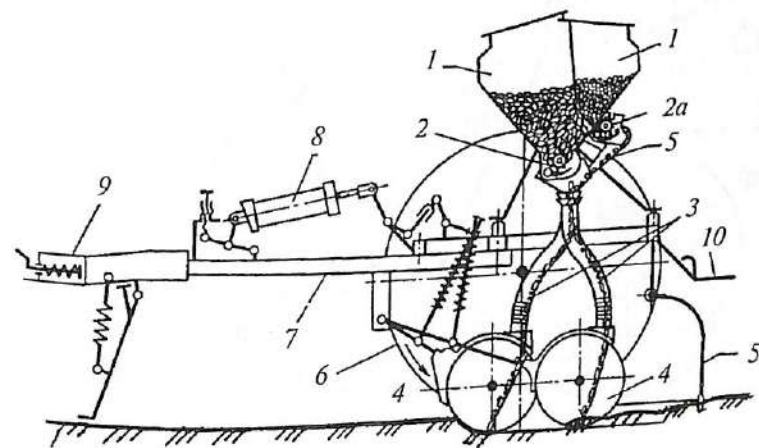
15-rasm. Universal seyalka.
