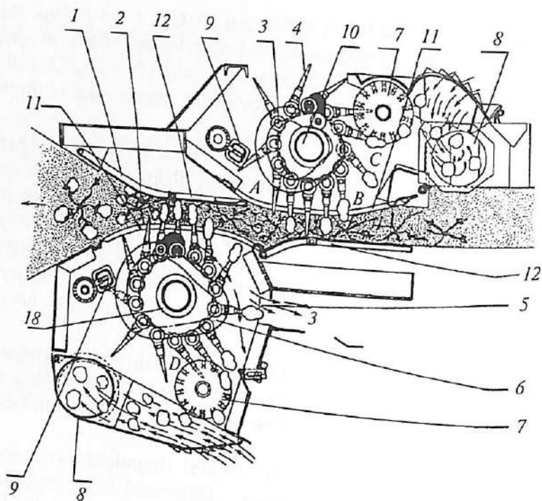
21- rasm. Gorizontal shpindelli paxta terish apparatining texnologik ish jarayoni:
