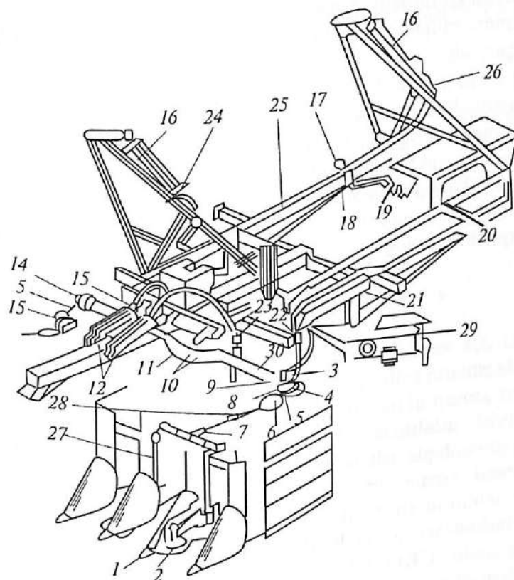
28-rasm. Bunker va terish apparatini ko'tarish sistemasi:
