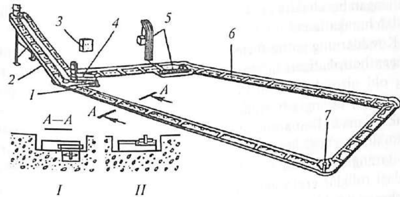
62-rasm. THC-2,0 go'ng yig'ish transportyor:
