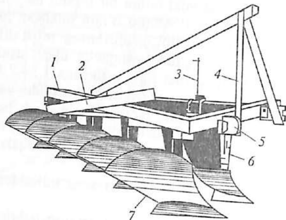
5-rasm. O'rnatma plug:
