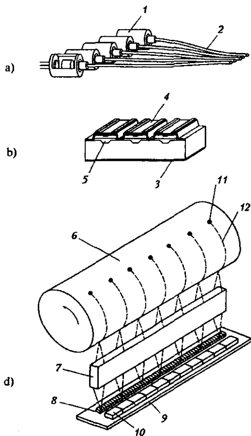
8.12-rasm. LED linekasidan foydalanuvchi printerning sxemasi:
