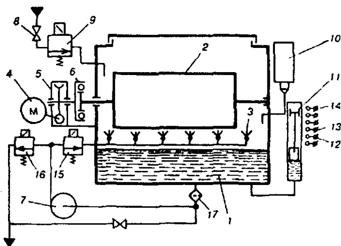
6.9-rasm. Oldindan bukilgan FBQni yuvish uchun protsessor.
