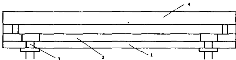
5.3-rasm. Nusxa ko'chiruvchi ramaning vakuumlash sistemasi: 1 – stol, 2 – rezina material; 3 – shtuser; 4 – kvarts shisha.
