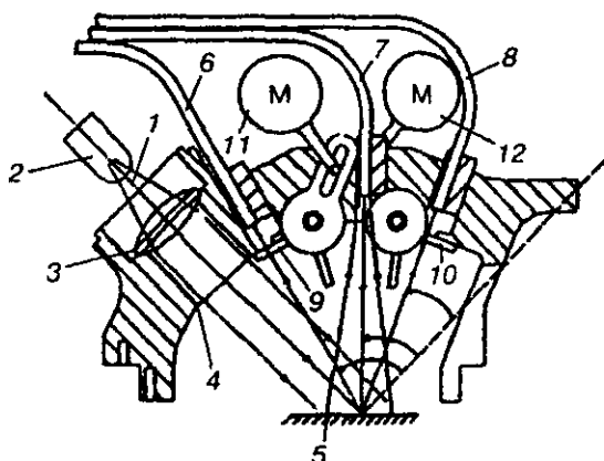
8.44-rasm. Spektrofotometming o'quvchi kallagi.
