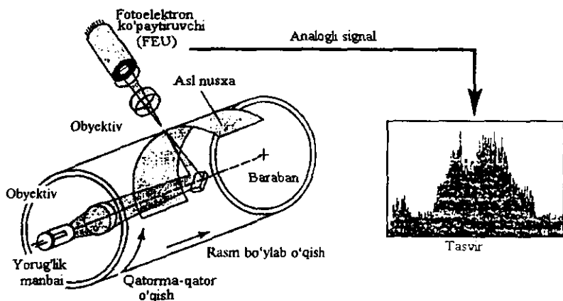
1.2-rasm. Baraban turdagi skanerda FEU ishlash sxemasi.
