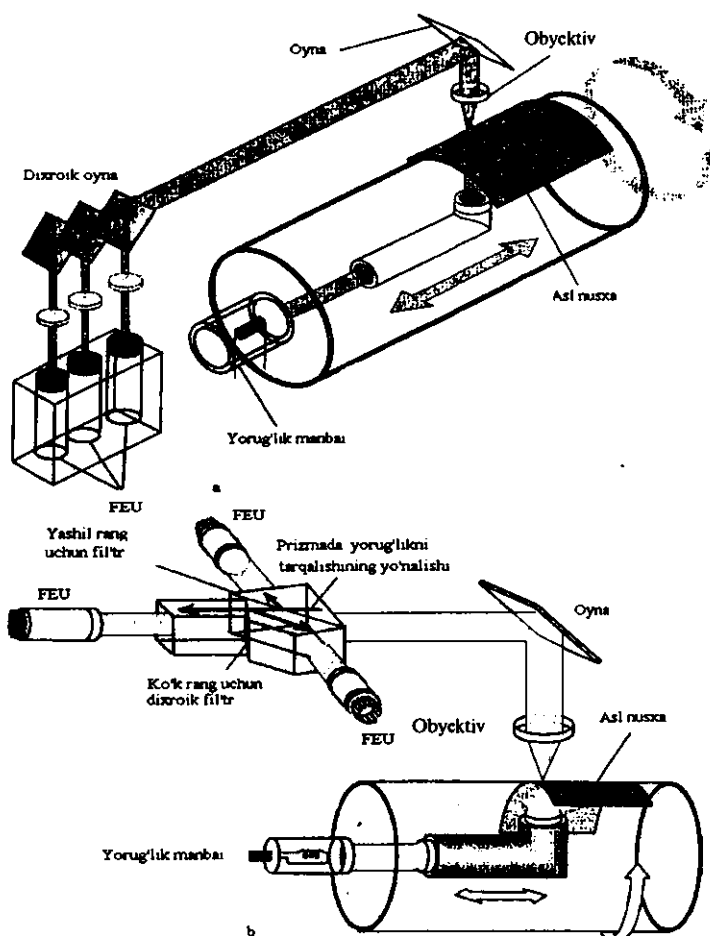
1.8-rasm. Baraban turdagi skaner: a – dixroik oynali; b – rangga ajratuvchi prizmalı Fujifilm FineScan 2750.
