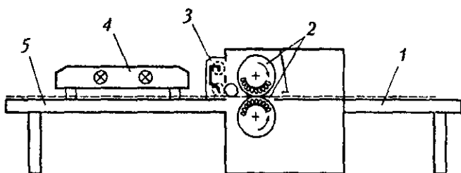
8.38-rasm. Yoritgichli laminatorning prinsipial sxemasi:
