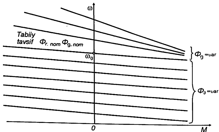
3.2- rasm. Generator-dvigatel tizimining mexanik tavsiflari.
