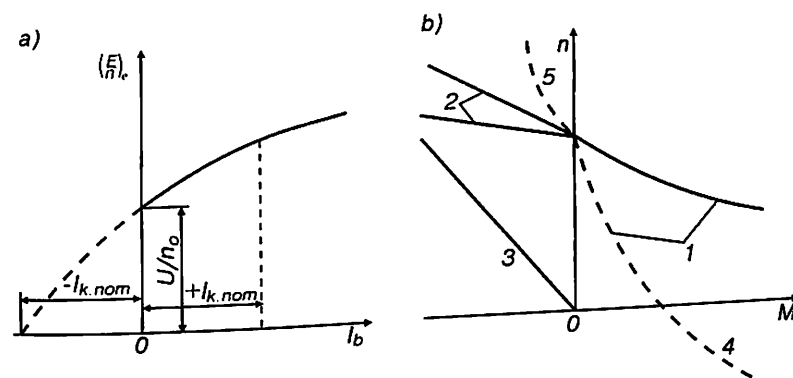
2.27- rasm. Aralash qo'zg'atishli dvigatel tavsiflari: a — o'tish tavsifi ( I_{q,nom} — ketma-ket qo'zg'atish chulg'amidagi nominal tok); b — mexanik tavsif.
