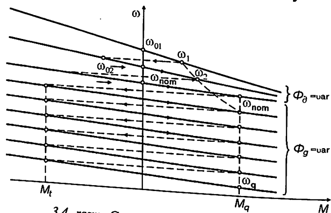
3.4- rasm. Generator-dvigatel tizimini tormozlashdagi mexanik tavsiflar.
