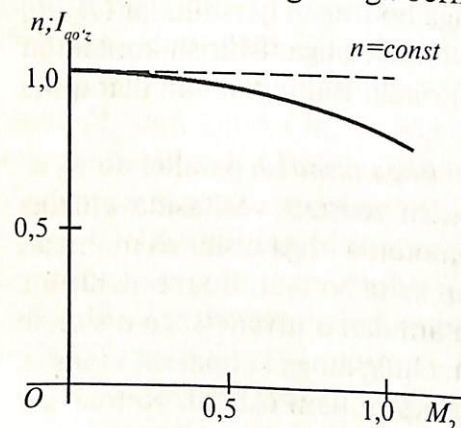
4.8- rasm. Parallel qo'zg'atishli motorning n = n_N = \text{const} va U = U_N = \text{const} bo'lgandagi rostlash xarakteristikasi — I_{qo'z} = f(M_2) .
