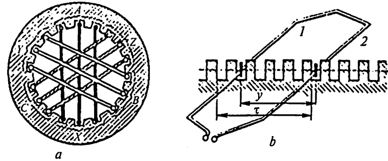
11.1-rasm. Stator chulg'amining o'rami (a) va g'altagi (b).
