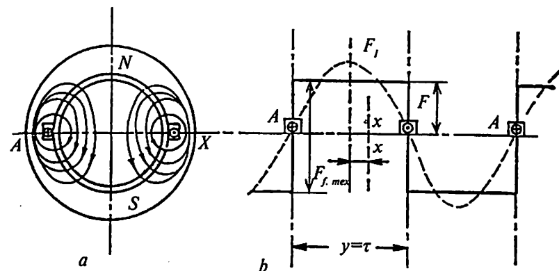
11.6- rasm. Yig'ilgan chulg'amning MYK.
