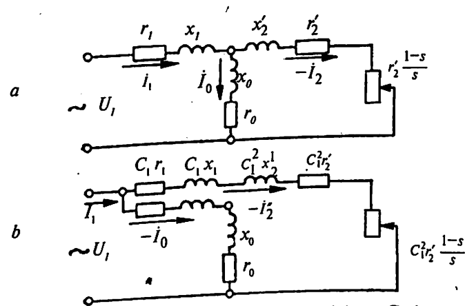
12.4- rasm. Asinxron motorning T simon (a) va G simon (b) almashtirish sxemalari.
