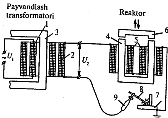
9.3-rasm. Payvandlash transformatori (reaktor ajratib ko'rsatilgan):
