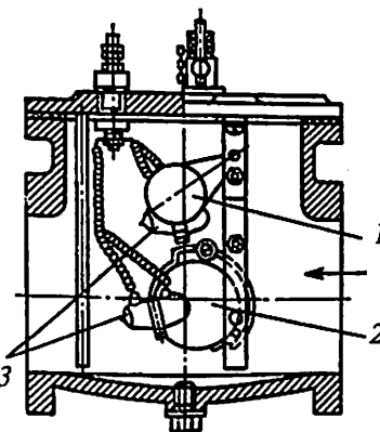
10.2-rasm. Transformatorning gaz relesi:
