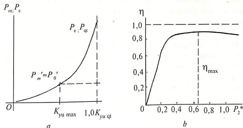
21.1- rasm. Elektr mashinalarida o'zgarmas va o'zgaruvchan isroflar (a); FIK ning yuklamaga nisbatan o'zgarishi (b).
