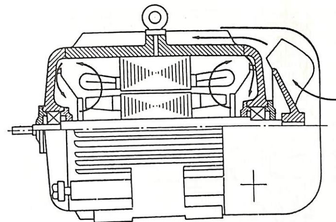
21.4- rasm. IP44 himoyalalanish darajali asinxron motorda sovitish muhitining harakatlanishi.
