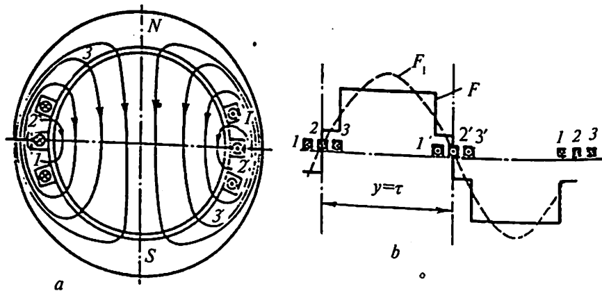
11.7- rasm. Ikki qutbli mashina tarqalgan chulg'amining MYK.
