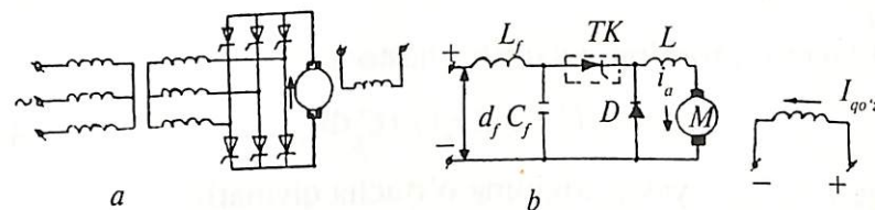
4.11- rasm. Boshqariladigan to'g'rilagichdan ta'minlanadigan mustaqil qo'zg'atishli motorning aylanish chastotasini rostlash (a), o'zgaras tok motorini impulsli rostlash (b): d_f C_f —kirish filtri; TK—tiristorli kalit; D —teskari diod; L_f —induktivlik.
