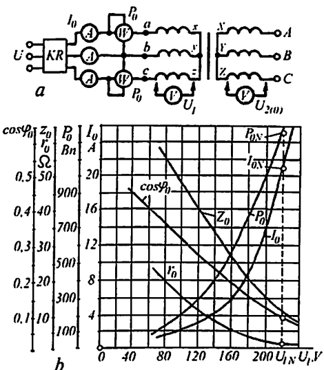
7.2-rasm. Uch fazali ikki chulg'amli transformatorning salt ishlash tajribasini o'tkazish sxemasi (a) va salt ishlash xarakteristikalar (b); KR — kuchlanishni rostlagich
