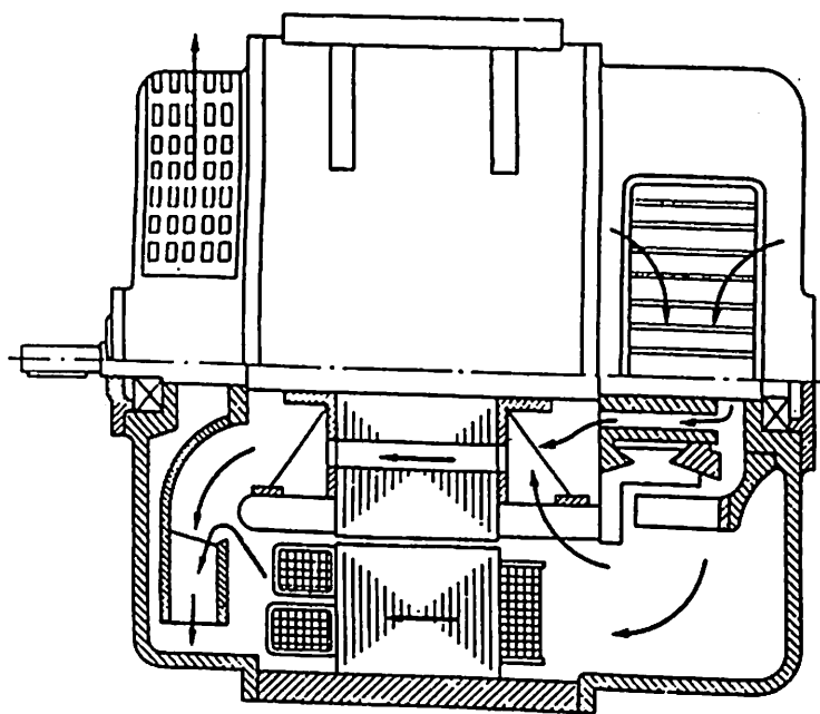
21.6- rasm. Ventilatsiyaning aksial sistemasida IP23 himoyalanish darajali o'zgarmas tok motorida sovitish muhitining harakatlanishi.
