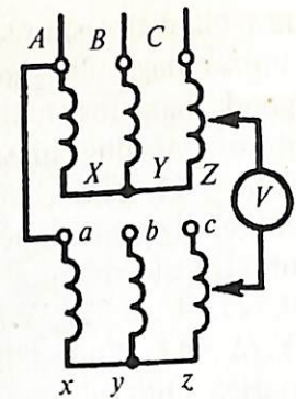
8.3- rasm. Transformatorning ulanish guruhini tajriba yo'li bilan voltmeter usulida aniqlash.
