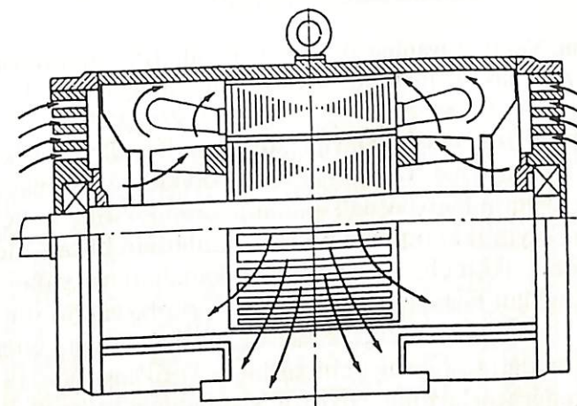
21.5- rasm. Ventilatsiyaning radial sistemasida IP23 himoyalalanish darajali asinxron motorda sovitish muhitining harakatlanishi.
