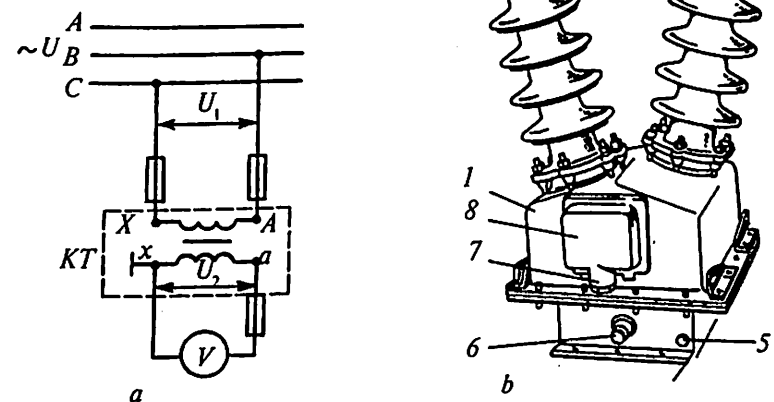
9.6- rasm. Kuchlanishi 35 kV bo'lgan NOM-35 kuchlanish transformatorini tarmoqqa ulash sxemasi (a) va uning tashqi ko'rinishi (b):
