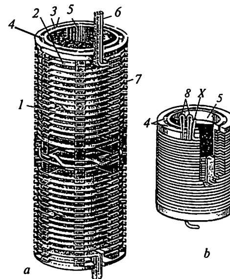
6.3- rasm. Transformator chulg'amlari: a—bir yo'lli vintsimon chulg'am; b—ko'p qatlamli silindrik chulg'am:
