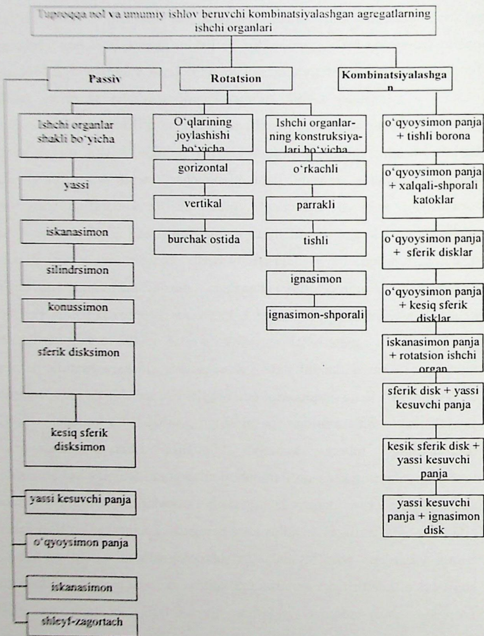
1.1-rasm. Ishchi organlarning tasnifi
