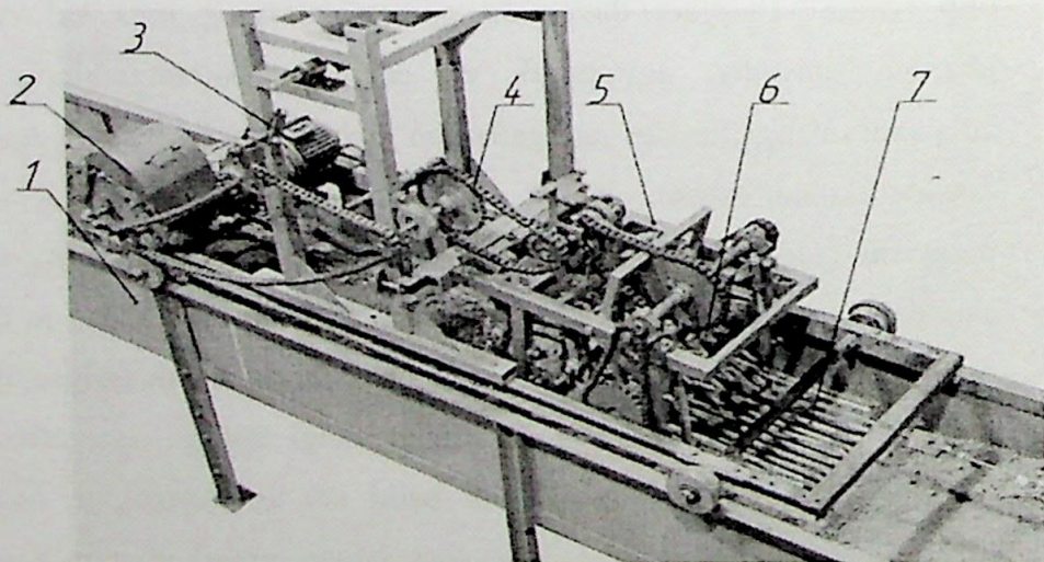
1.3.1-Rasm Tuproq kanalida eksperimental laboratoriya o'rnatish:
