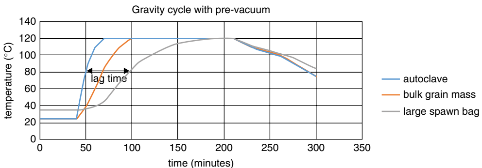
Figure 5.19 Gravity cycle – comparison of different spawn production systems.
