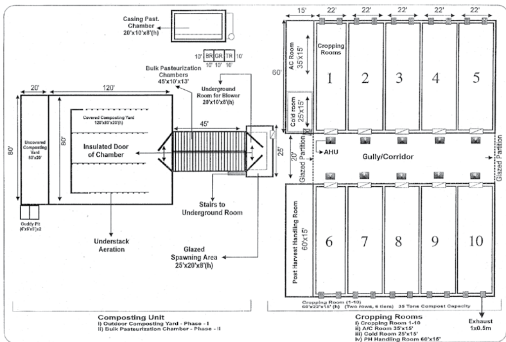
Figure 14.1 General layout of 250 TPA (tons per annum) mushroom farm.
