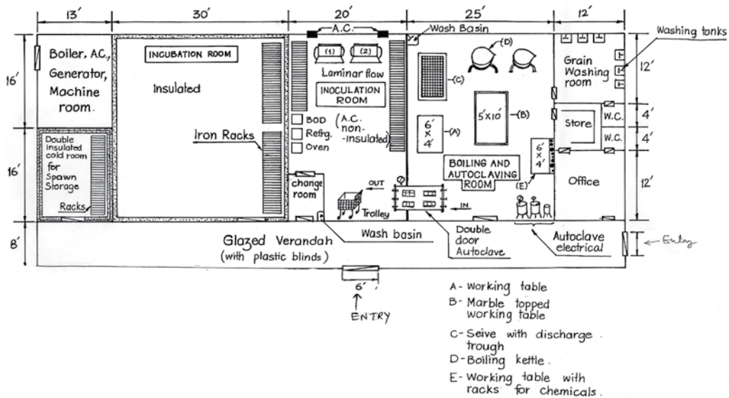
Figure 14.5 Layout plan of a spawn lab.
