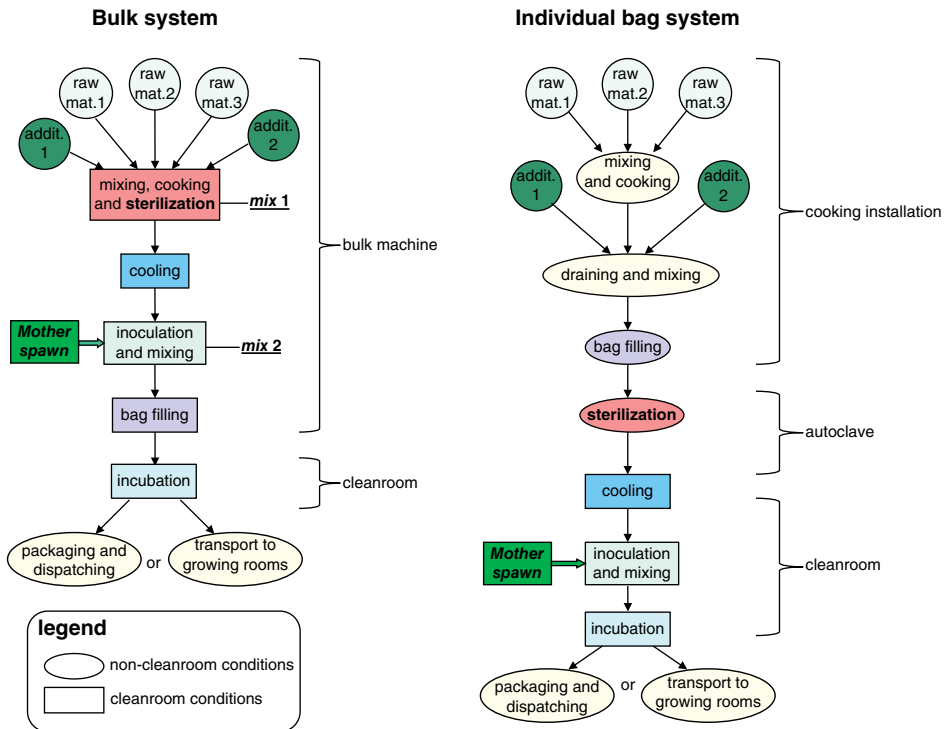
Figure 5.4 Comparison of product flow of two spawn production methods: sterilization in bulk or individual bags.
