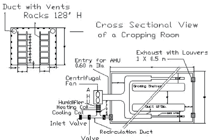
Figure 14.8 Internal layout of a cropping room (length 18 m/60'; width 7 m/22'; height 4.4 m/15').
