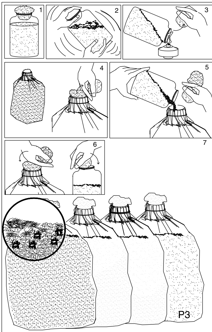
Figure 5.2 Example of inoculation practice of small grain bags without inbuilt filter.
