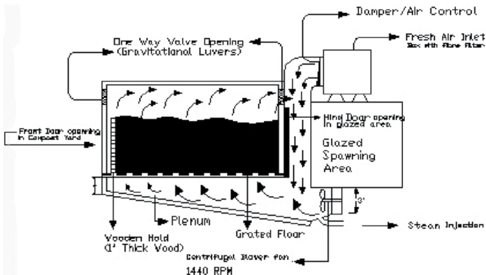
Figure 14.3 Cross section of a compost bulk pasteurization chamber (length 13 m/45', width 3 m/10', height 4 m/13').
