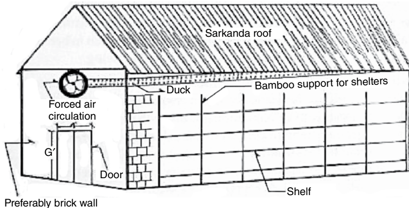
Figure 14.7 Low cost growing room.
