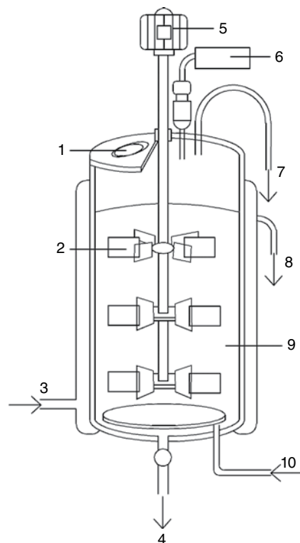
Figure 18.4 Schematic diagram of STRs. 1. Charging hole; 2. Mixer; 3. Cooling water inlet; 4. Clean hole; 5. Electric engine; 6. A device for measurement and control; 7. Blow vent; 8. Cooling water outlet; 9. Liquid-state medium; 10. Sterile air.
