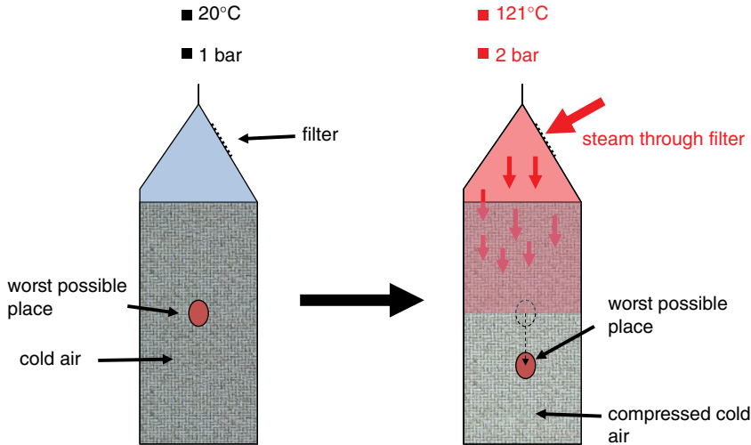
Figure 5.18 Compression of gases in bag during autoclaving.
