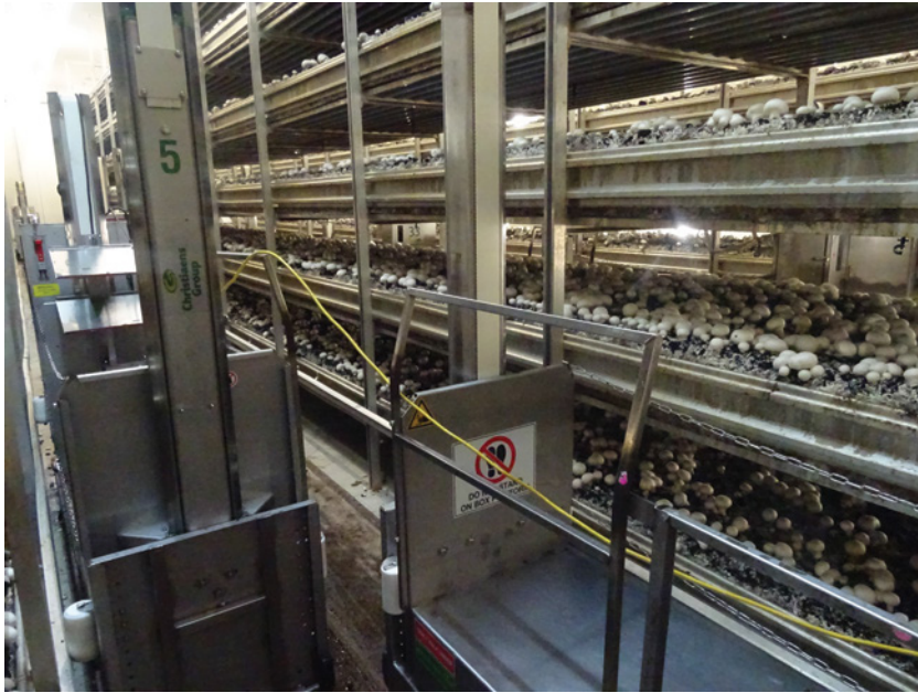
Figure 9.5 Automatic lorry: the yellow cable follows after picking to connect the batteries.
