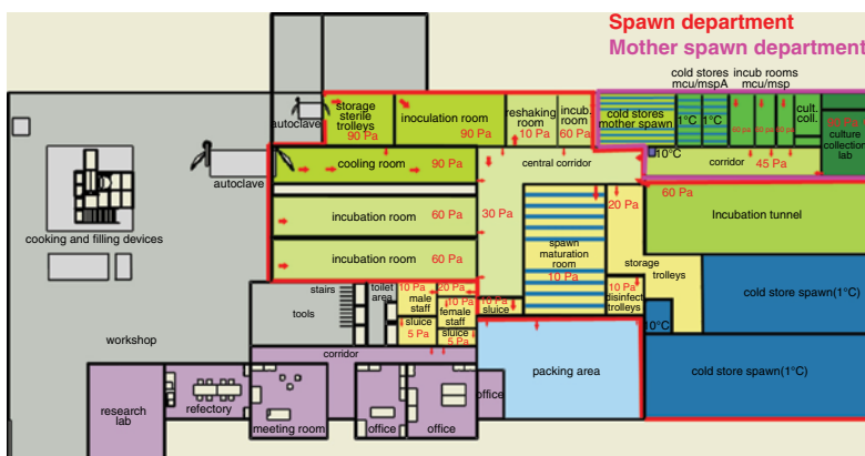
Figure 5.16 Floor plan of a grain spawn lab, depicting overpressure flow and pressure fall. Note the size of the mother spawn department compared to the spawn department.
