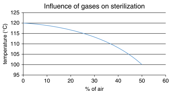
Figure 5.20 Influence of gases on sterilization temperature.
