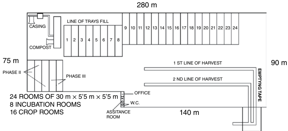
Figure 10.1 Plan view of a typical mushroom farm.
