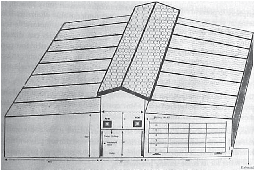
Figure 14.6 Front cross-sectional view of cropping rooms.
