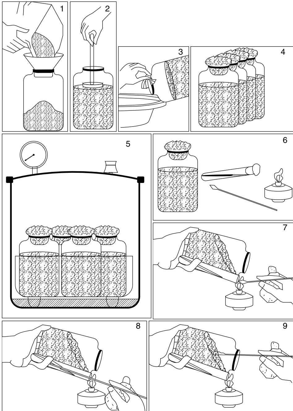
Figure 5.15 Making pre-culture spawn in cleanroom conditions.
