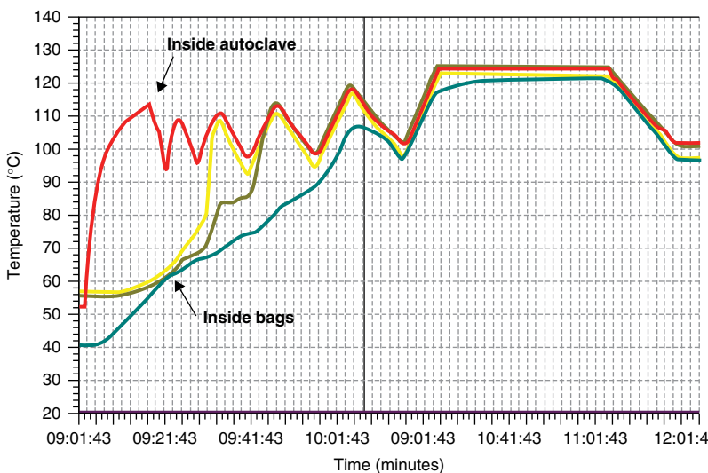
Figure 5.21 Vacuum sterilization cycle – sterilization of porous and bagged goods.
