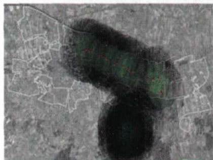
62-rasm. Havo ifloslanish modeli
