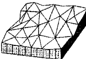
TIN model
