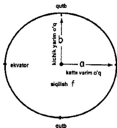
2.2-rasm. Ellipsoid (manba: Internet)
