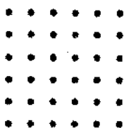
(1) Grid nuqtalar
