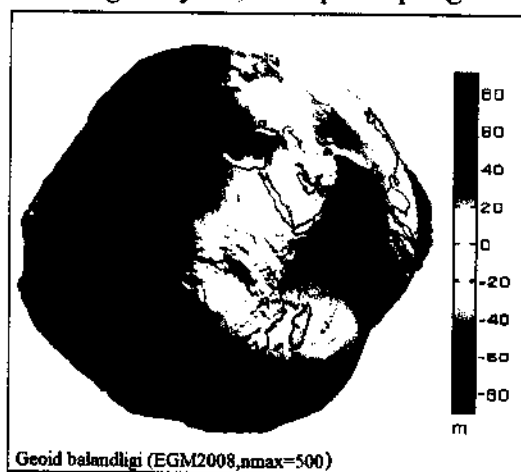
2.1-rasm. Geoid shakli (manba: Internet)
