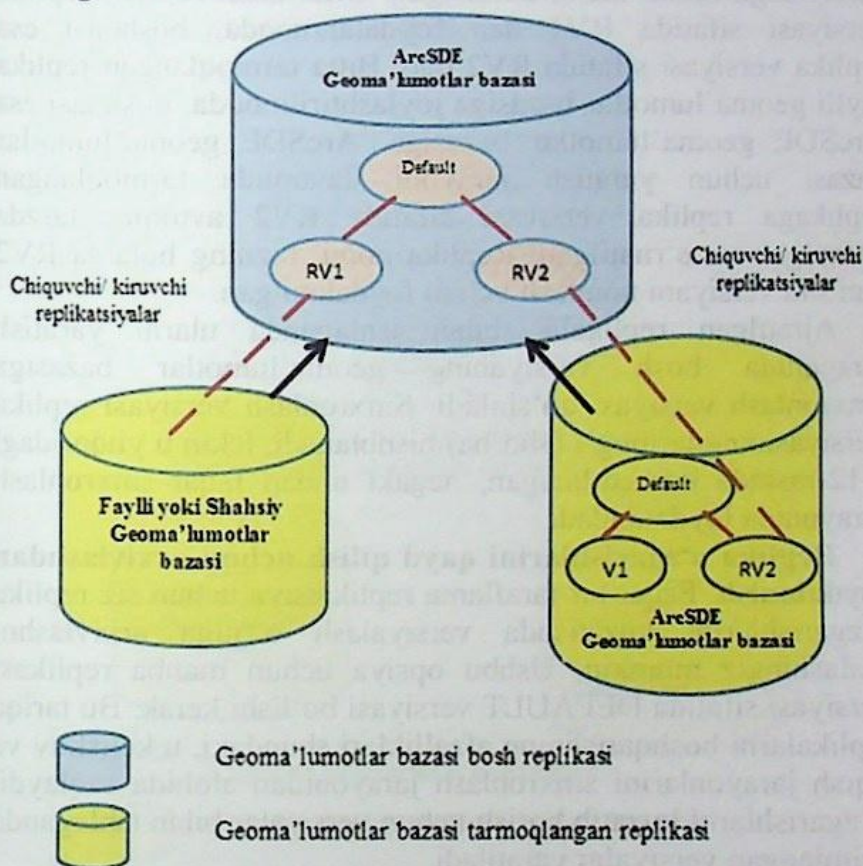
6.12-rasm. Ajratilgan replika va uning replika versiyasiga misol
