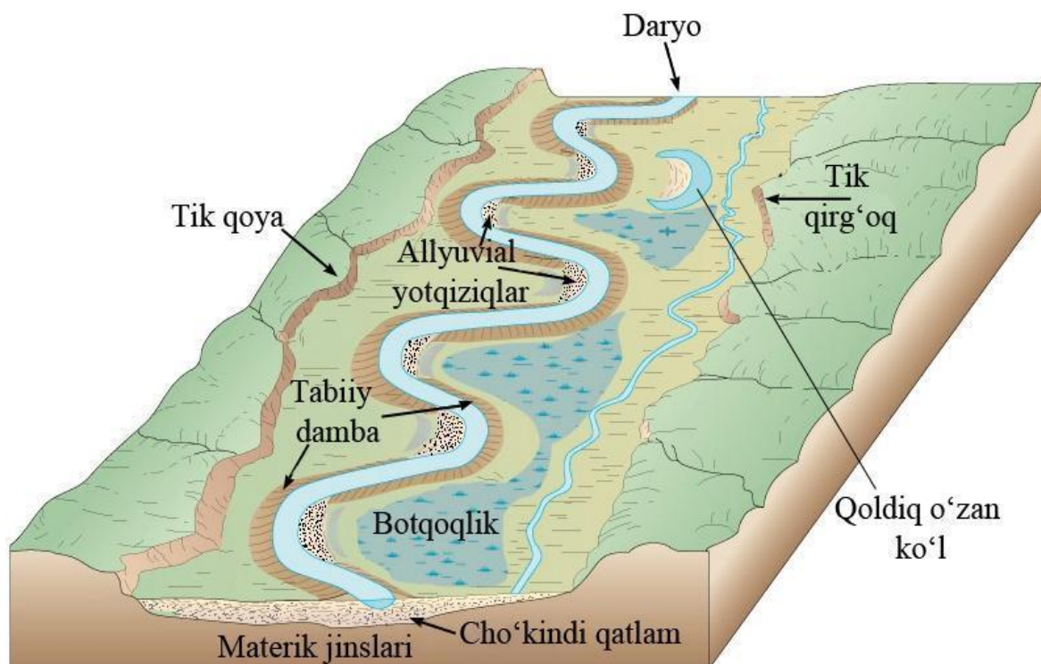
43-rasm. Daryoning meandra hosil qilish jarayoni
