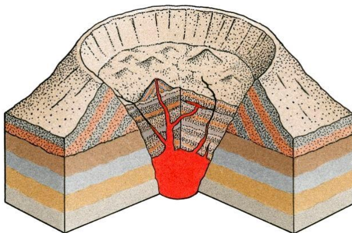
39-rasm. Kaldera
