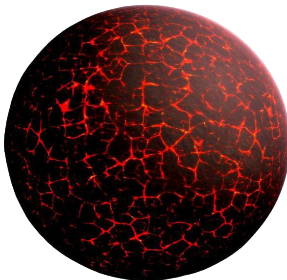
13-rasm. Xades eonida Yerning holati
