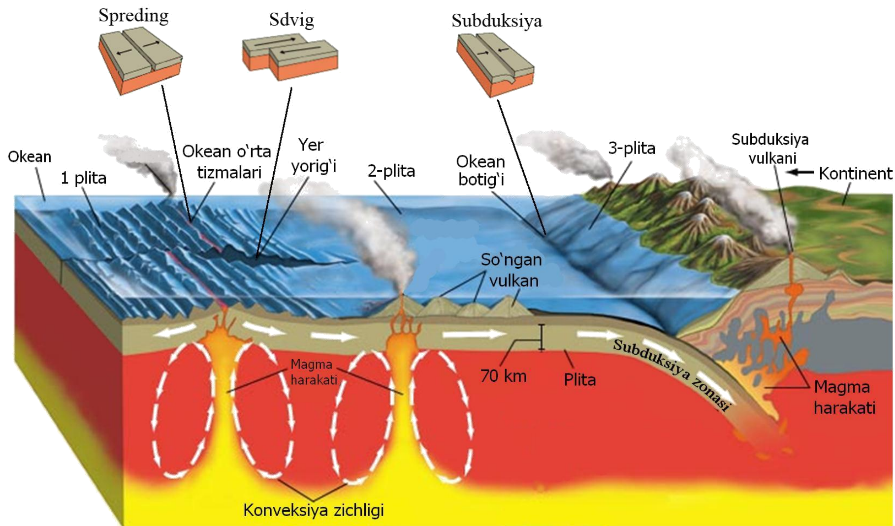
6-rasm. Litosfera plitalari harakati
