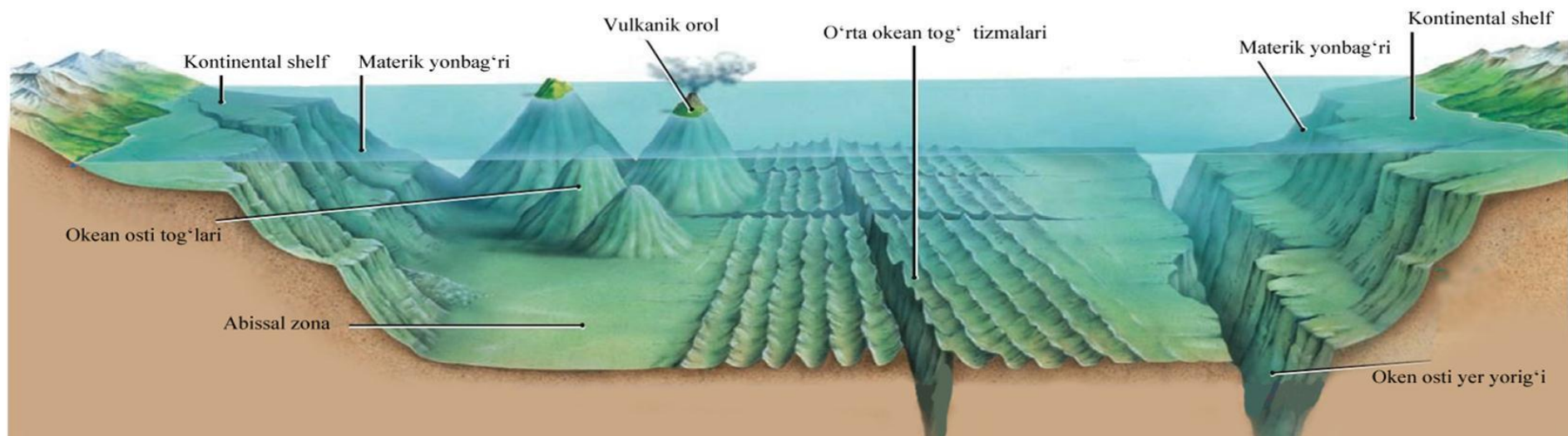
70-rasm. Okean osti relyef shakllari
