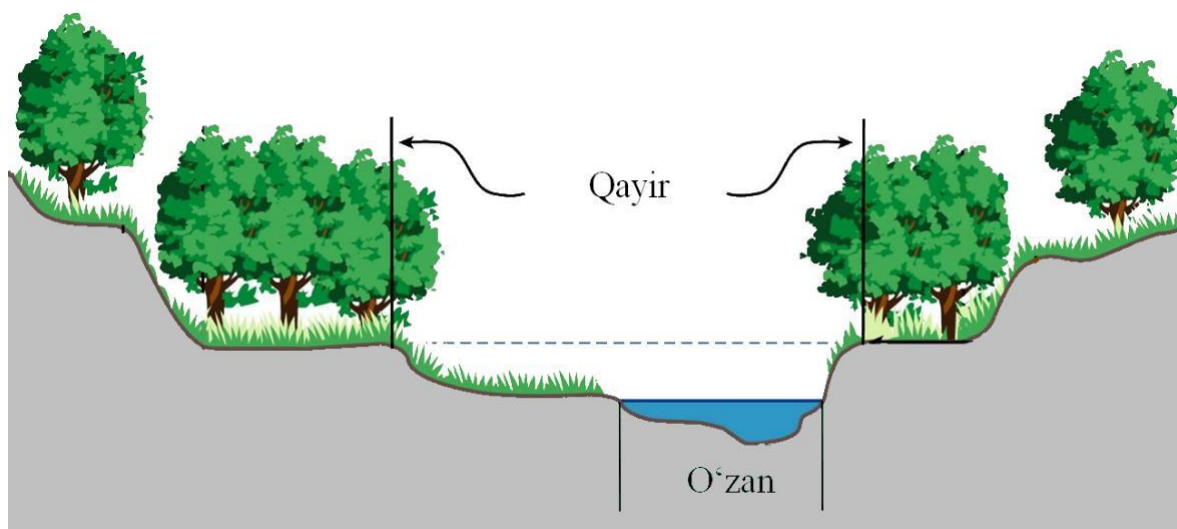
44-rasm. Daryo o'zani va qayir
