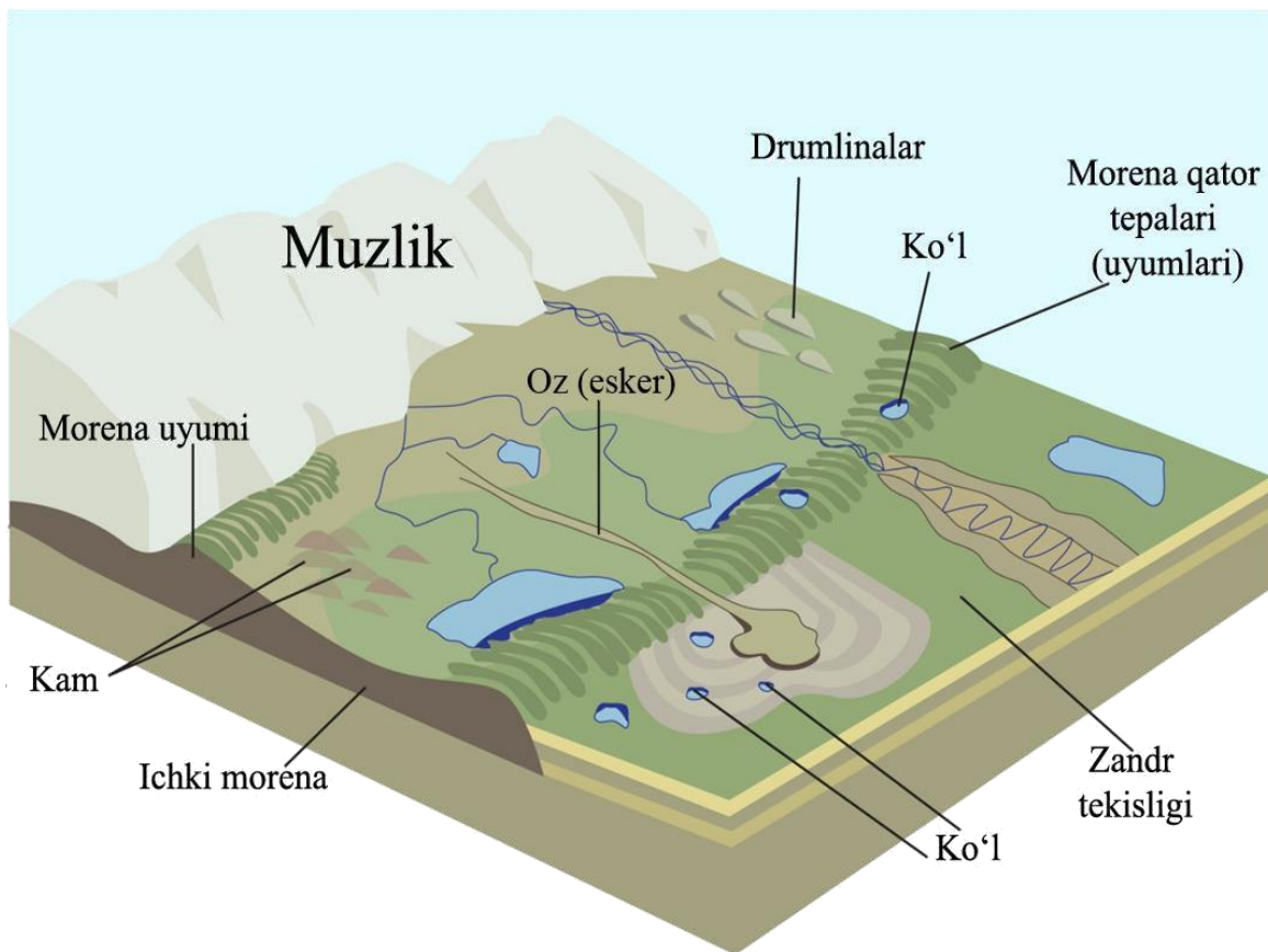
61-rasm. Glyatsial relyef shakllari
