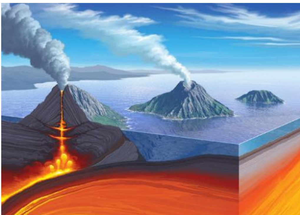
40-rasm. Vulkanik orollar
