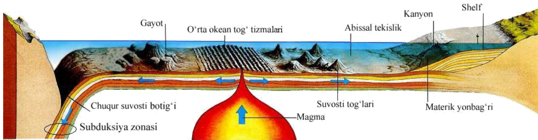
69-rasm. Okean osti relyef shakllari
