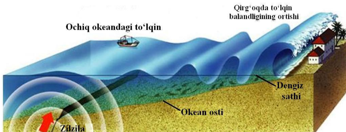
27-rasm. Zilzila va sunami
