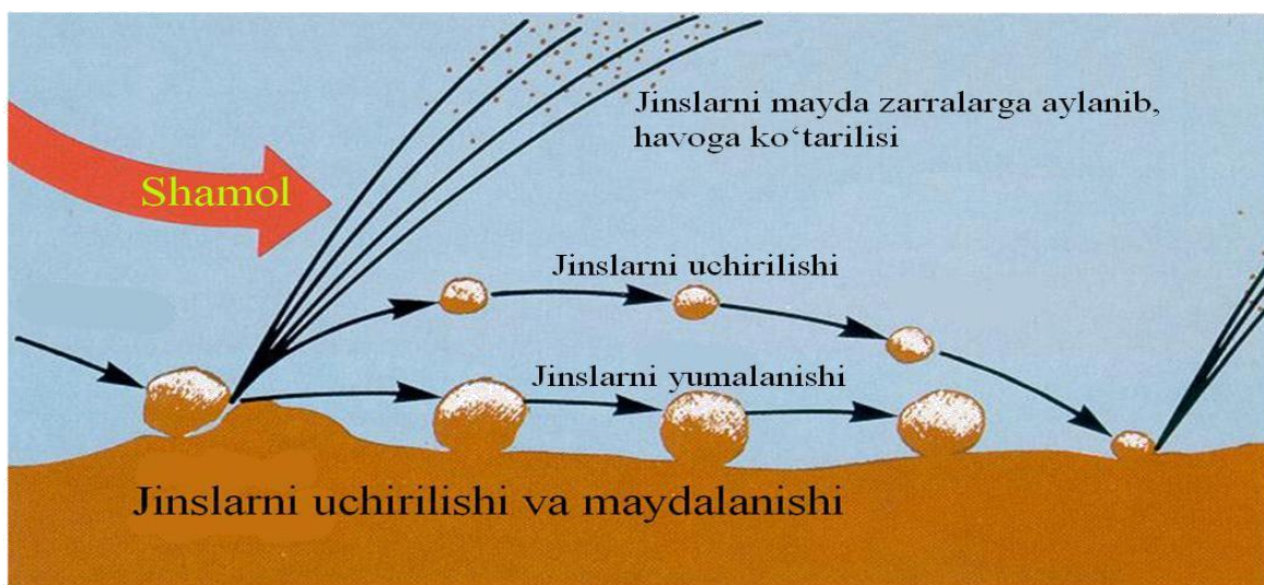
51-rasm. Deflyatsiya jarayoni
