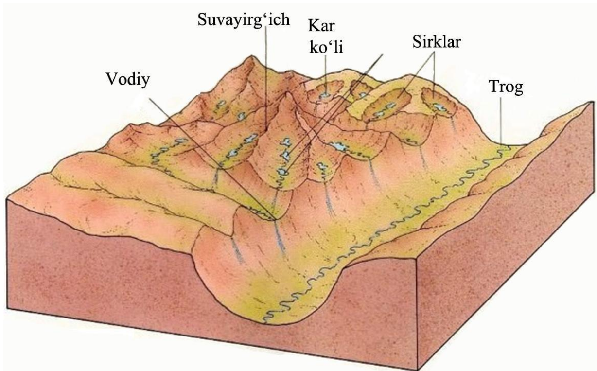
63-rasm. Trog vodiysi
