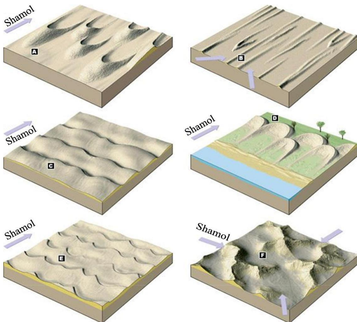
56-rasm. Eol relyef shakllari
