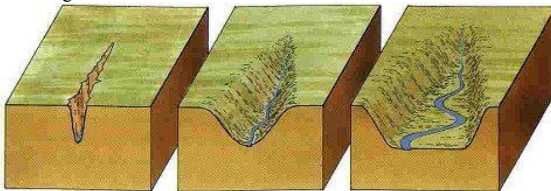
42-rasm. O'zan evolyutsiyasi
