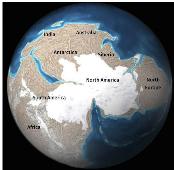
19-rasm. Rodiniya supermaterigi
