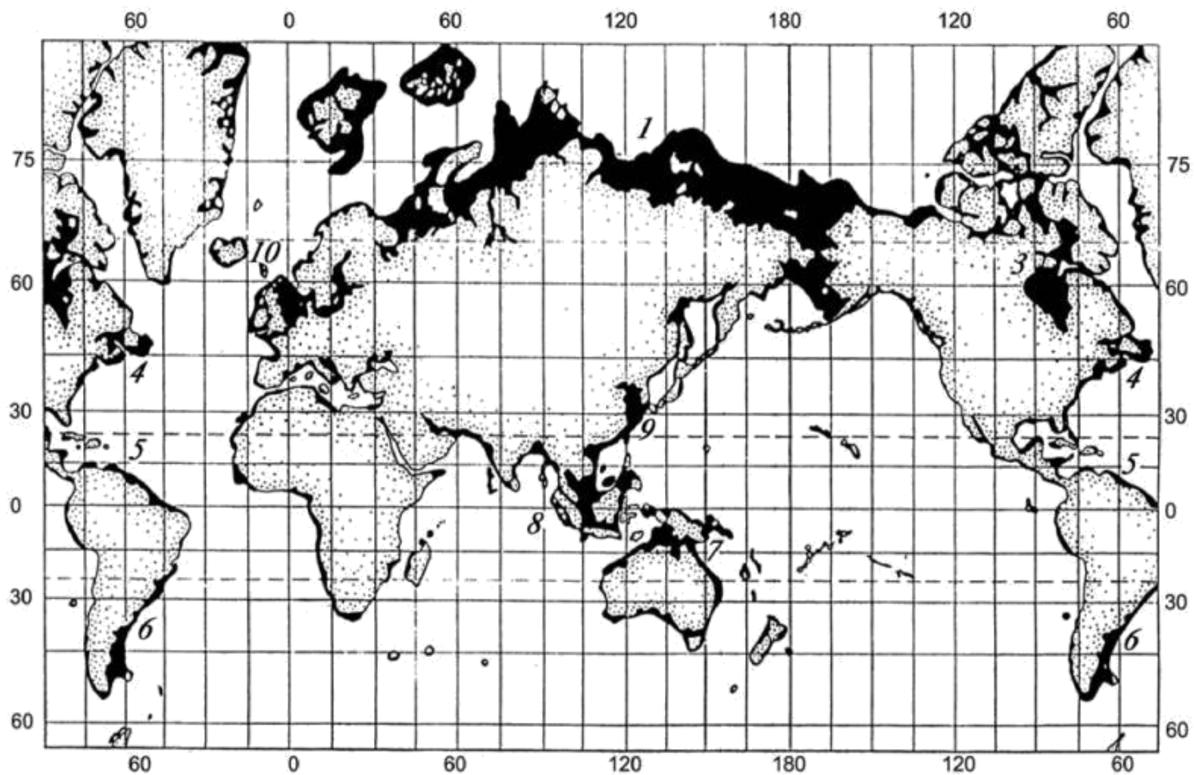
68-rasm. Yer sharida materik shelfining tarqalishi
