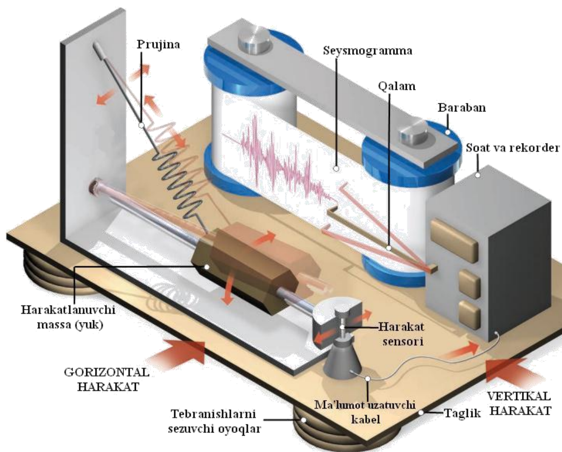
28-rasm. Zamonaviy seysmograf
