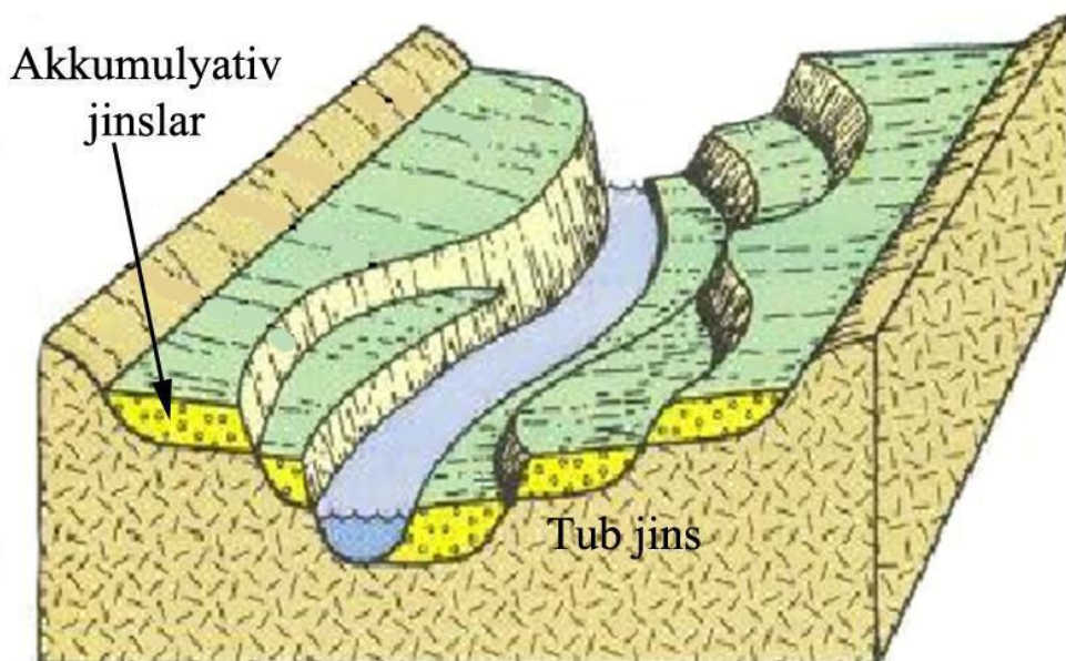
45-rasm. Erozion-akkumulyativ terrasa
