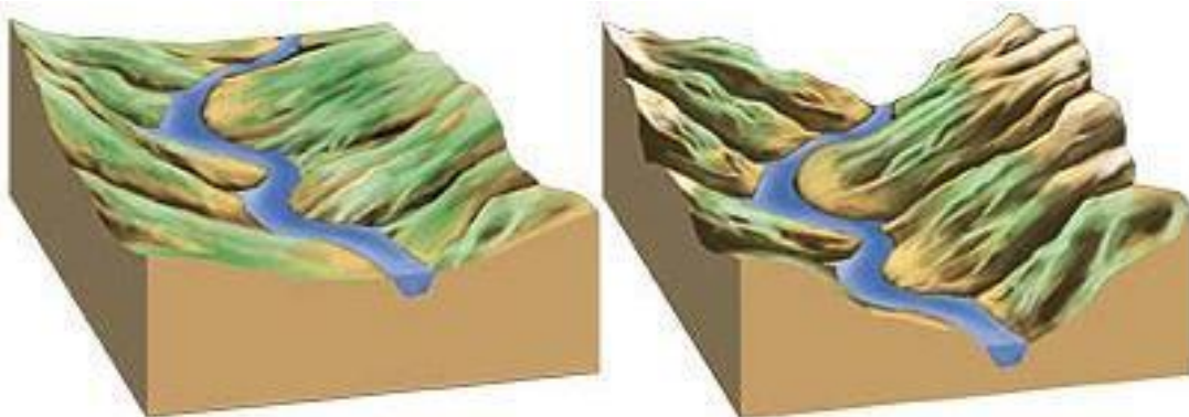
46-rasm. Daryo vodiysining rivojlanishi
