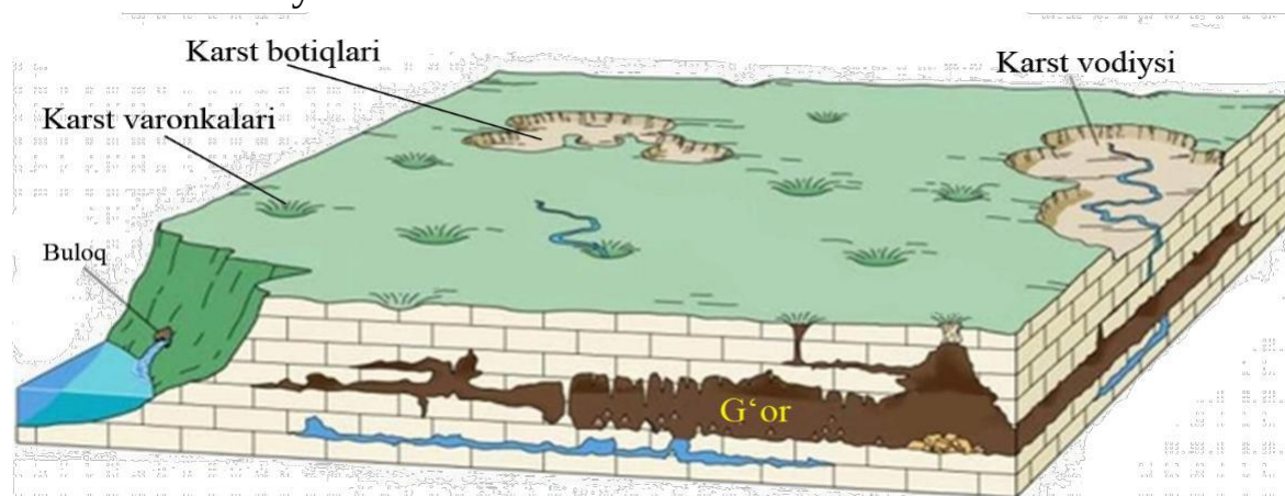
47-rasm. Karst jarayoni
