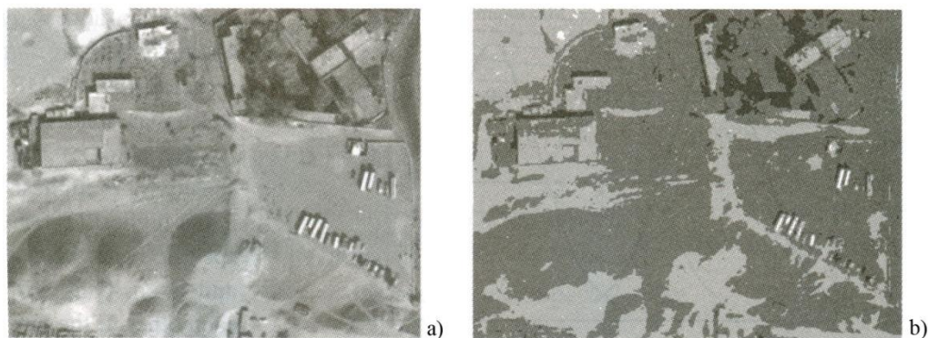
3.19-rasm. a) 8 bitli tasvir, b) 2 bitli tasvir.
