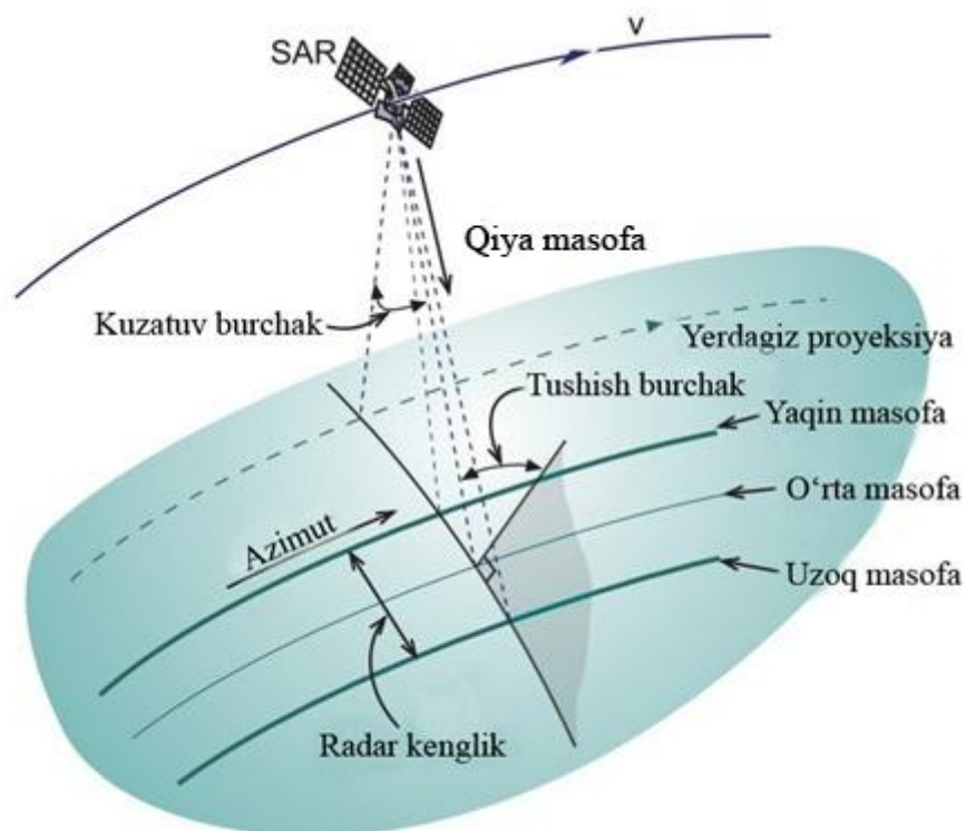
4.4-rasm. Radar masofadan zondlash geometriyasi.
