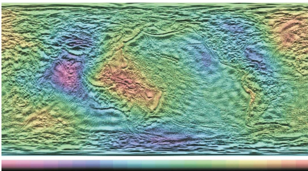
3.9-rasm. Radar altimetrda olingan tasvir.
