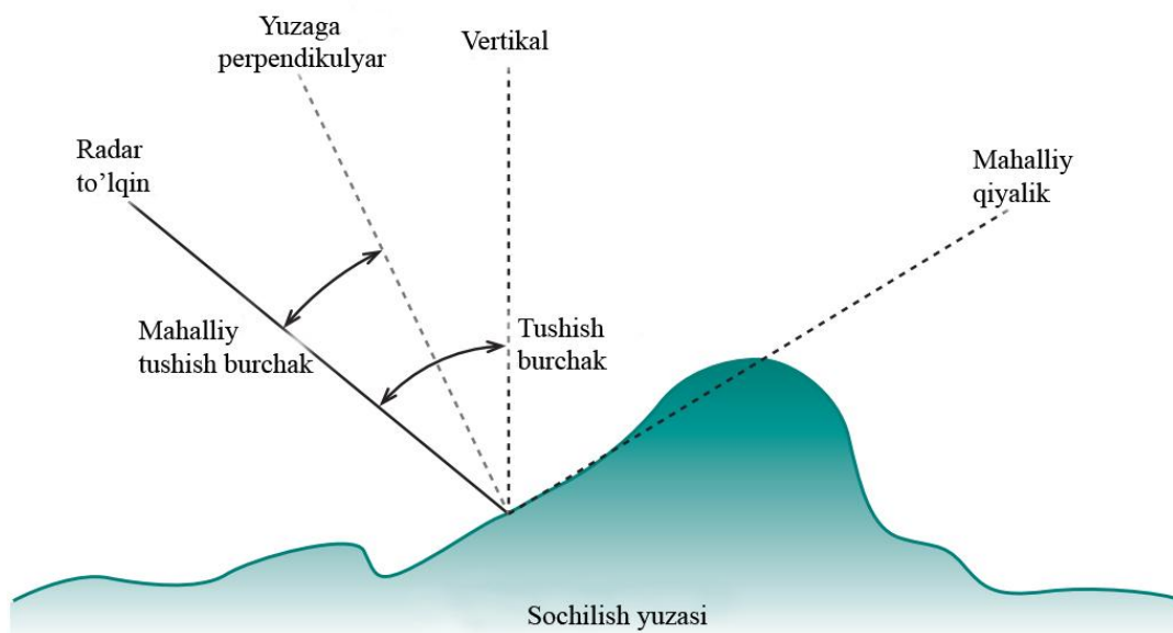
4.5-rasm. Radar va mahalliy tushish burchaklari.
