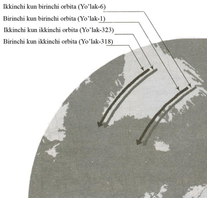
3.20-rasm. IRS Resourcesat-1 sun‘iy yo‘ldoshining orbitasi va yo‘lagi.
