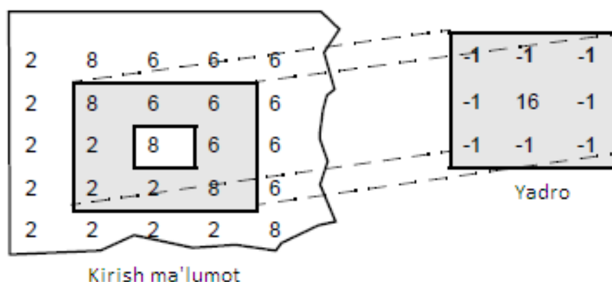
6.16-rasm. Namunaviy ma'lumotga 3 \times 3 o'rama yadro qo'llangan.
