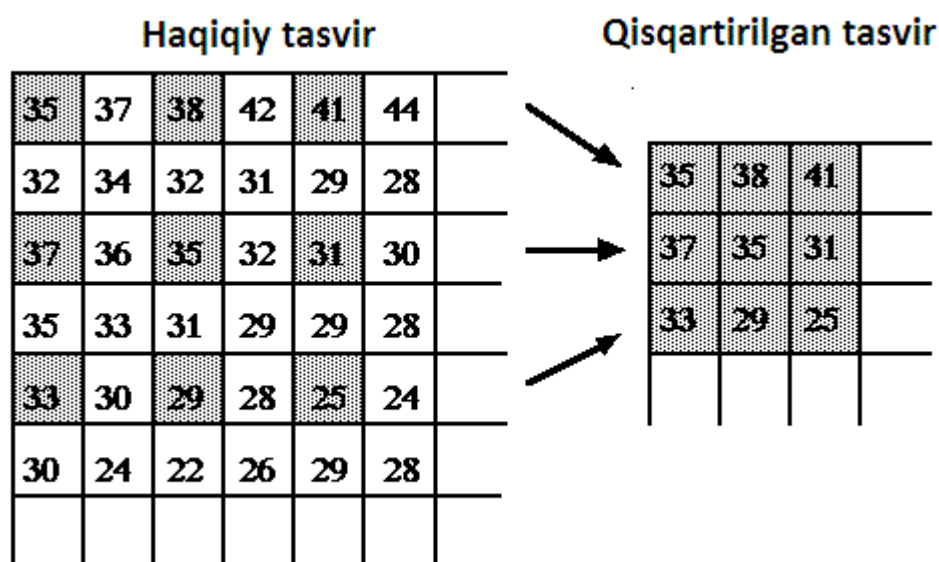
6.11-rasm. Tasvirni 2^x kichraytirish.
