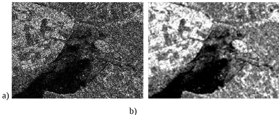
4.7-rasm. a) Asl va b) Donachali dog‘lardan filtrlangan radar tasvir.
