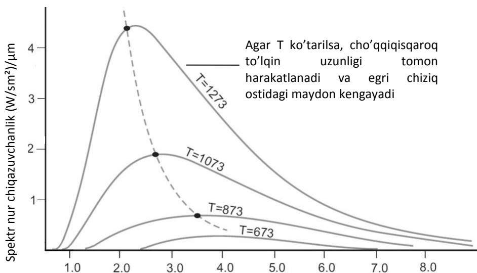
2.4-rasm. Stefan – Boltsman qonuniga asoslangan absolyut qora jism nurlanish egri chizig'i ( K haroratda).
