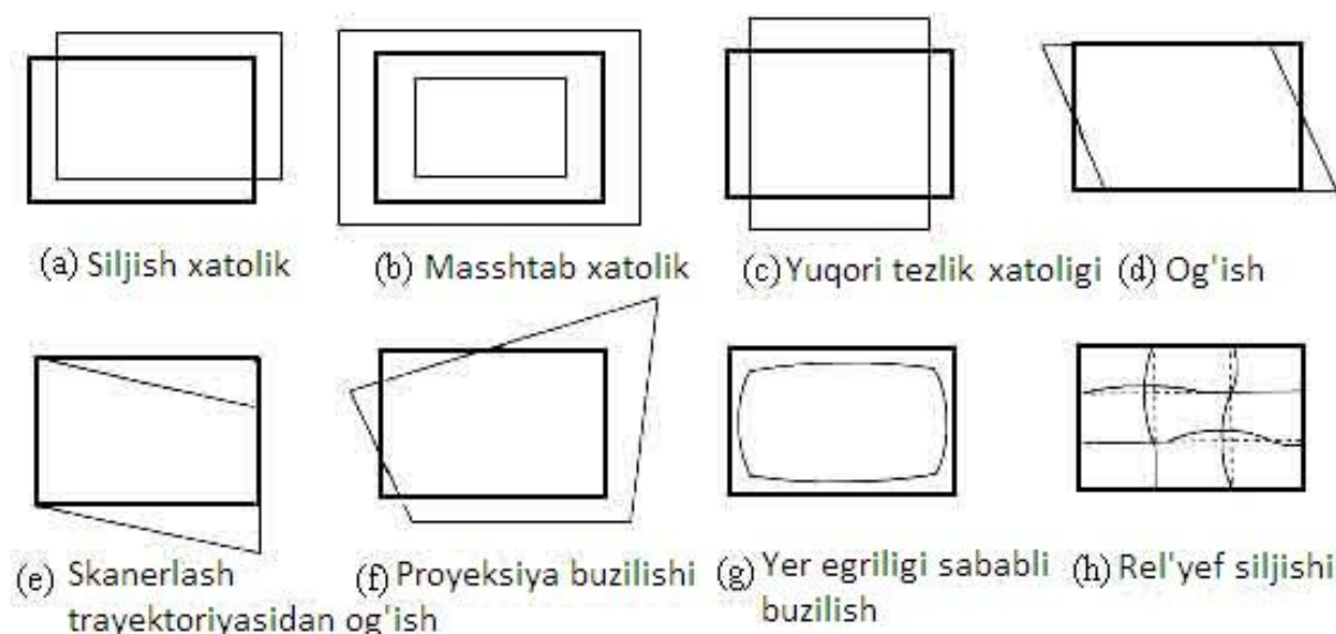
6.8-rasm. Tashqi buzilish.
