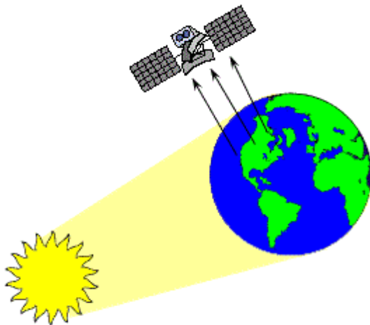
2.6-rasm. Passiv masofadan zondlash.
