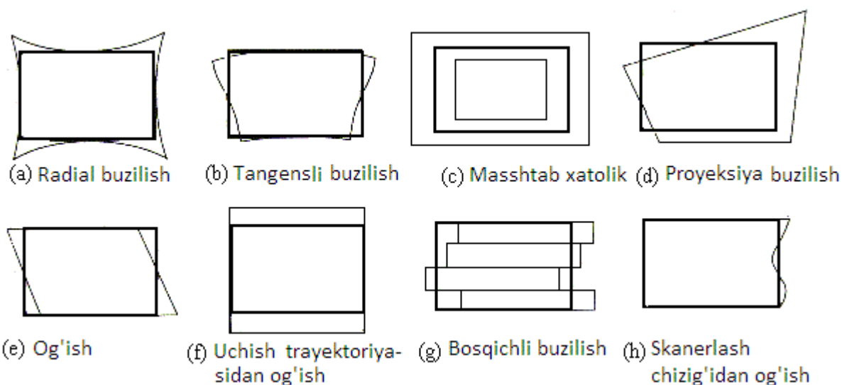
6.7-rasm. Ichki buzilish.
