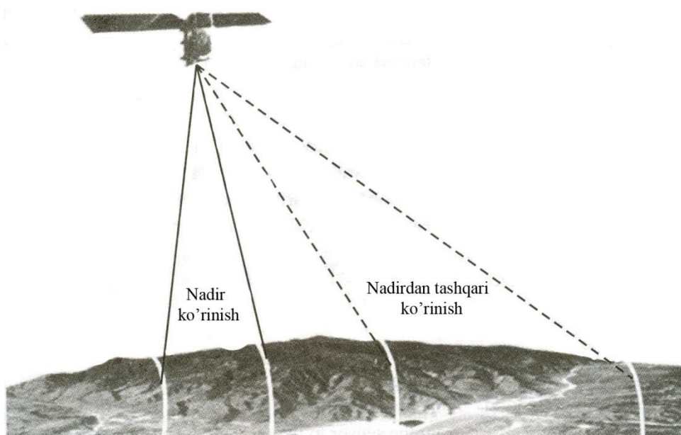
3.16-rasm. Nadir va nadirdan tashqari ko‘rinish.
