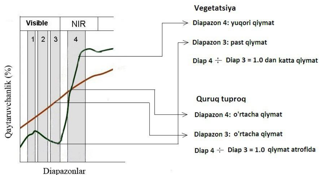
6.19-rasm. Yaqin infraqizildan qizilga koeffitsiyent.
