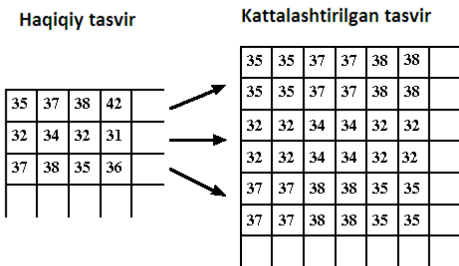
6.11-rasm. Tasvirni 2x kattalashtirish.
