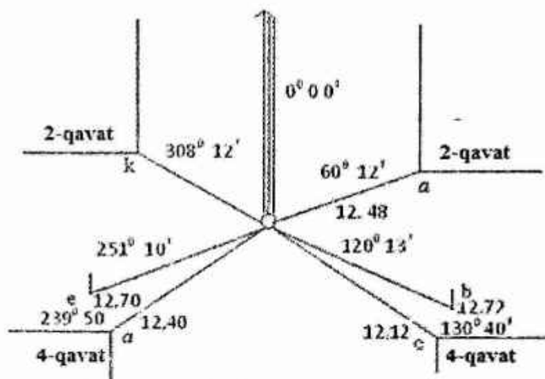
6.1-rasm. Quthiy usulda planga olish
