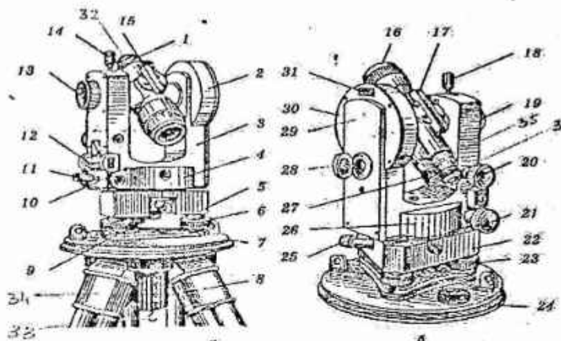
4.2-rasm. T30 teodolit tuzilishi
