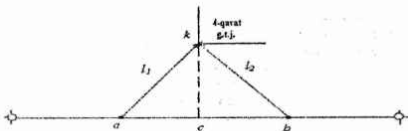
6.3-rasm. Chiziqli kestirma usuli
