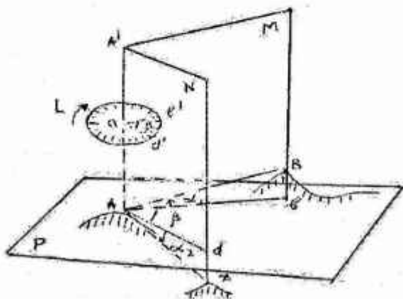
4.1-rasm. Gorizontol burchak o'lchash sxemasi
