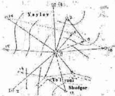
6.14-rasm. Taxeometrik syomka abrisi
