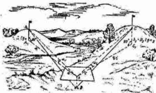
6.16-rasm. Grafik usulda plan olish
