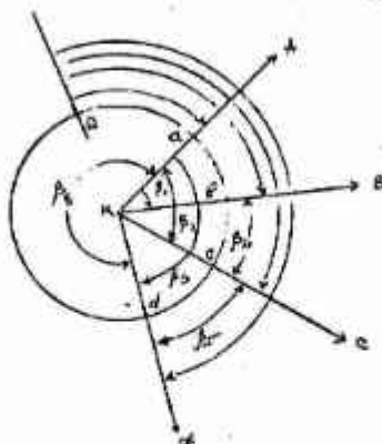
4.3-rasm. Doiraviy qabul usuli
