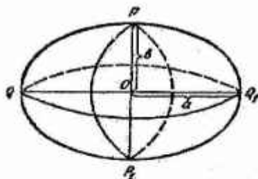
1.2-rasm. Ellipsoid.
