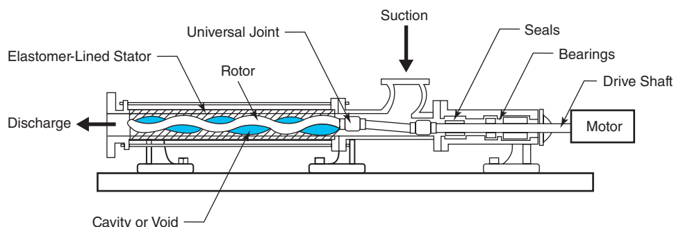
Figure 4.16 Progressive Cavity Pump Components
