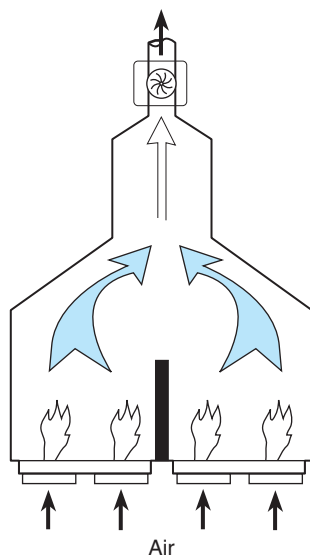
Figure 10.8 Induced-Draft Furnace
