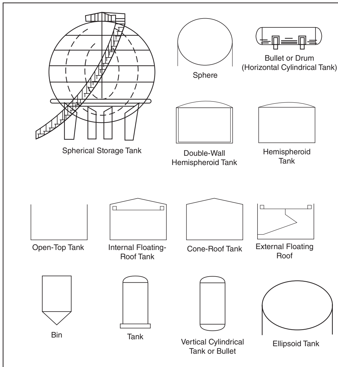
Figure 3.3 Tank Designs
