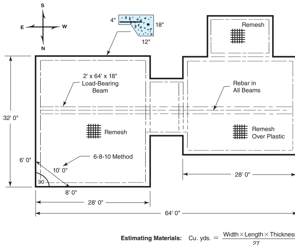
Figure 12.5 Foundation
