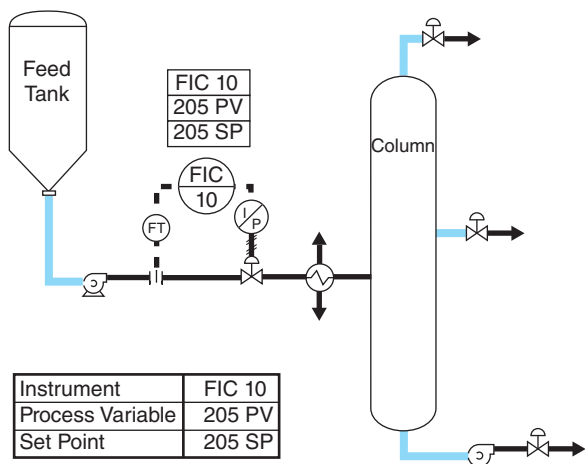
Figure 15.26 Troubleshooting: Problem 1
