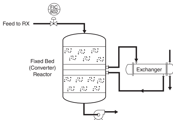
Figure 14.6 Converter (Fixed Bed) Reactor
