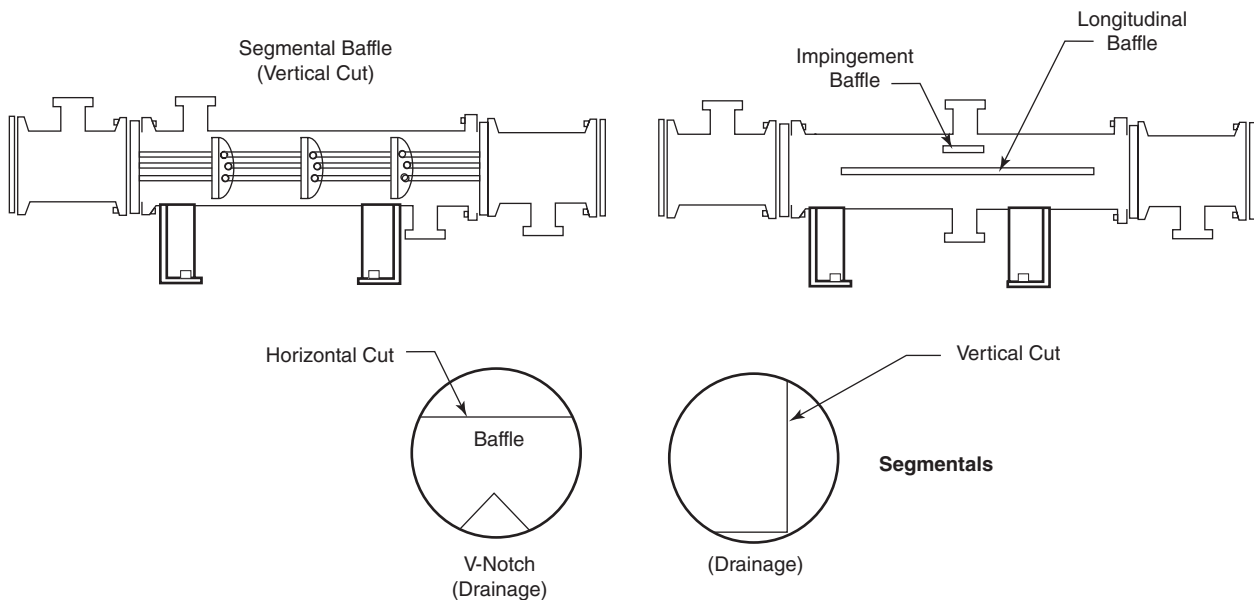
Figure 7.13 Baffle Arrangements
