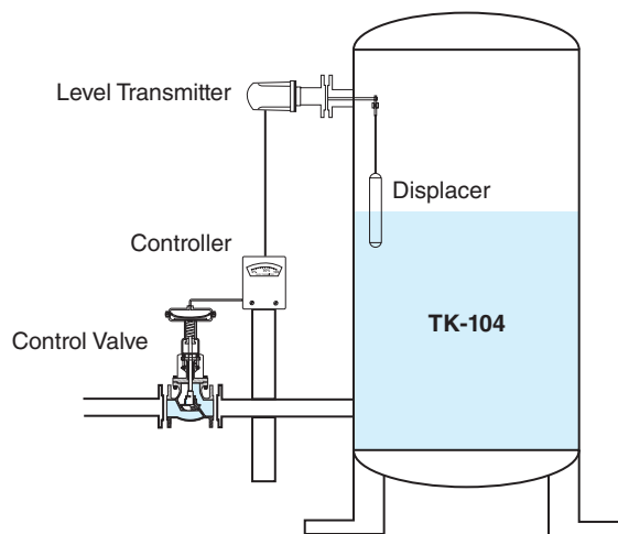
Figure 11.19 Level Control by Displacer
