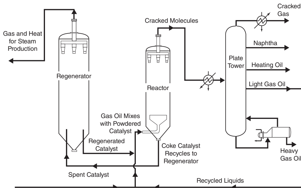
Figure 14.11 Fluid Catalytic Cracking
