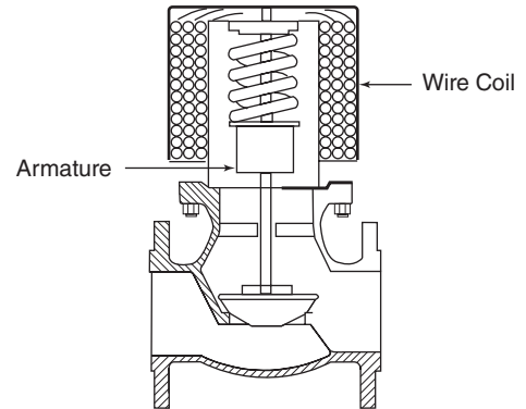
Figure 2.27 Solenoid Valve
