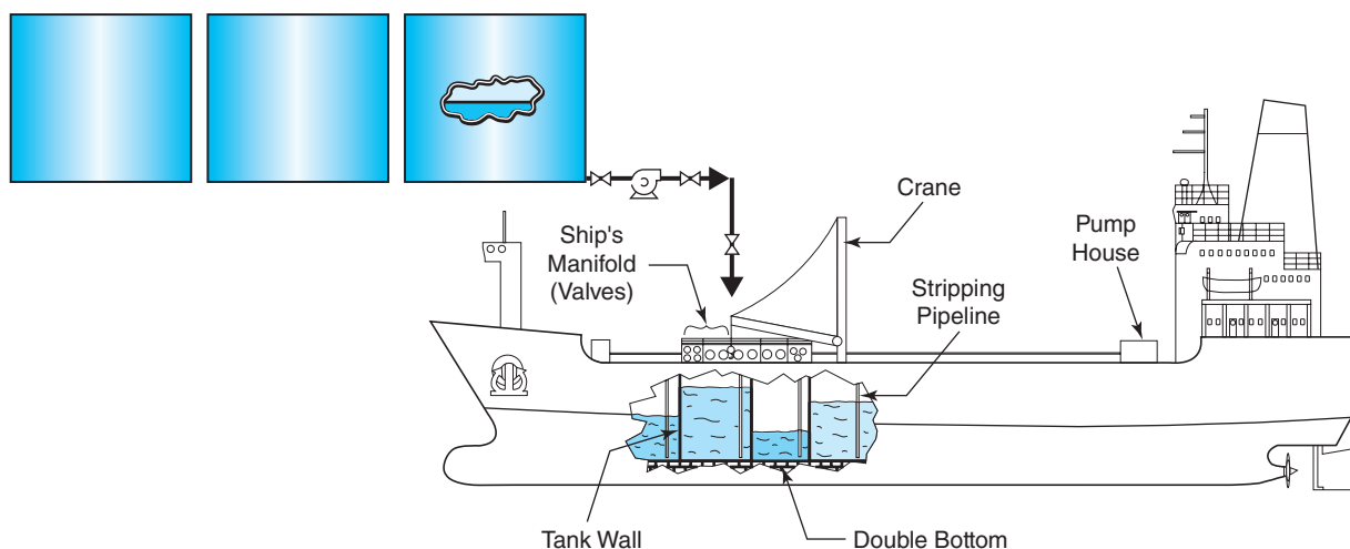
Figure 4.12 Tank-to-Ship Transfer
