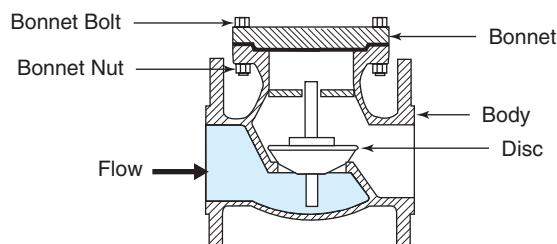
Figure 2.11 Lift Check Valve
