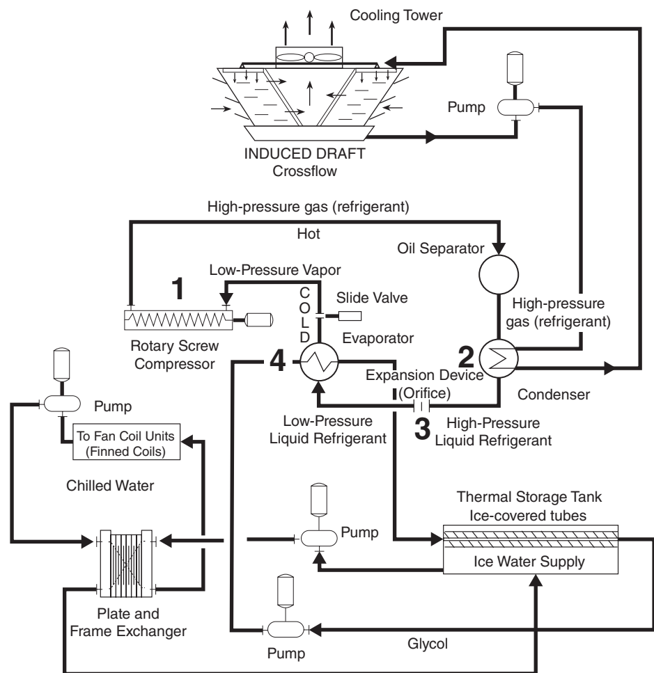
Figure 13.12 Refrigeration System
