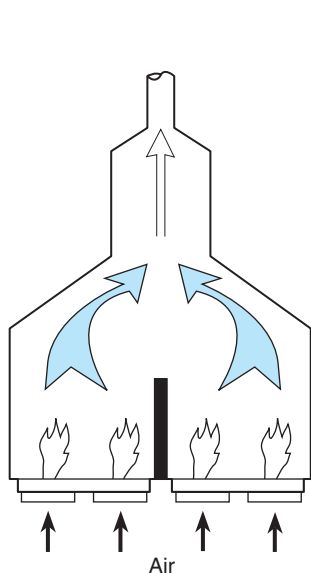
Figure 10.6 Natural-Draft Furnace
