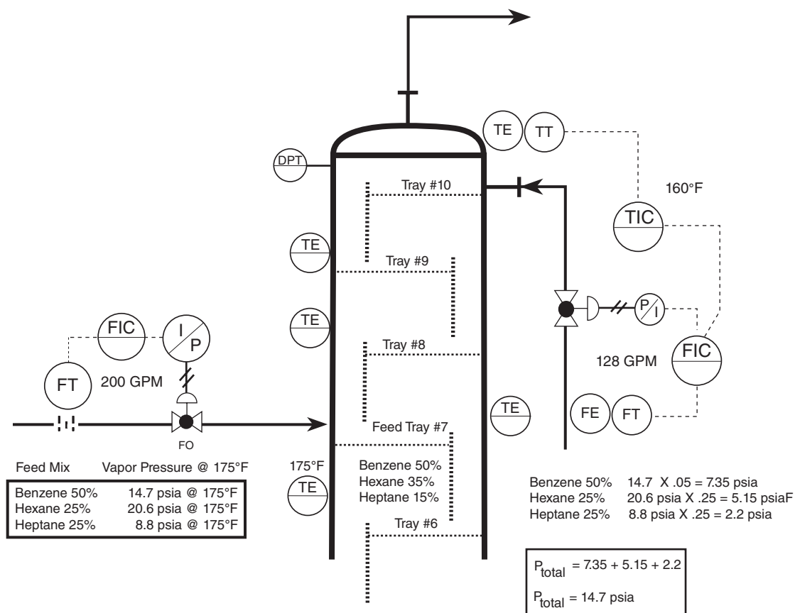
Figure 15.6 Dalton's Law of Partial Pressures
