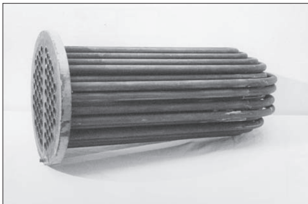
Figure 7.17 U-Tube
