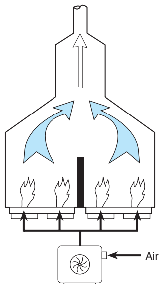
Figure 10.7 Forced-Draft Furnace
