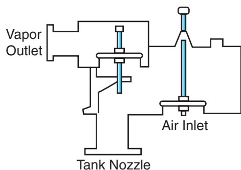
Figure 3.6 Conservation Vent
