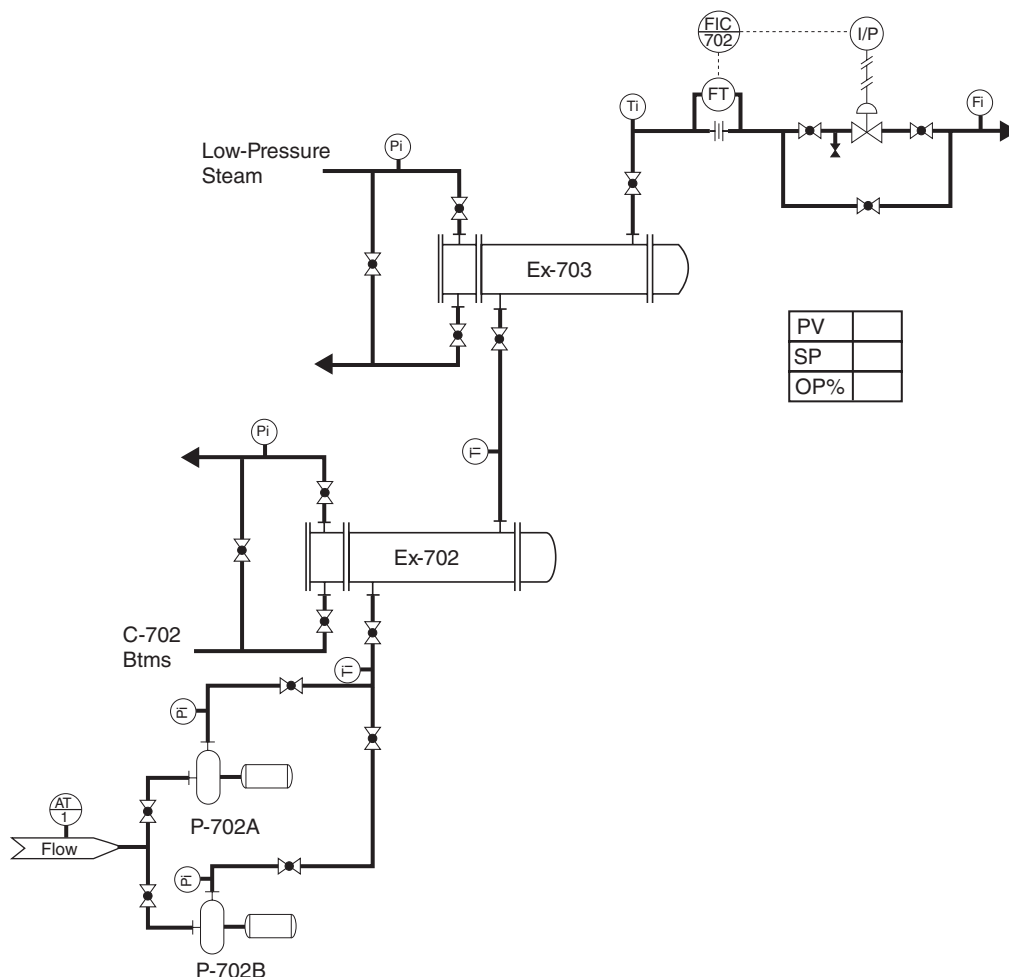
Figure 15.22 Preheat System
