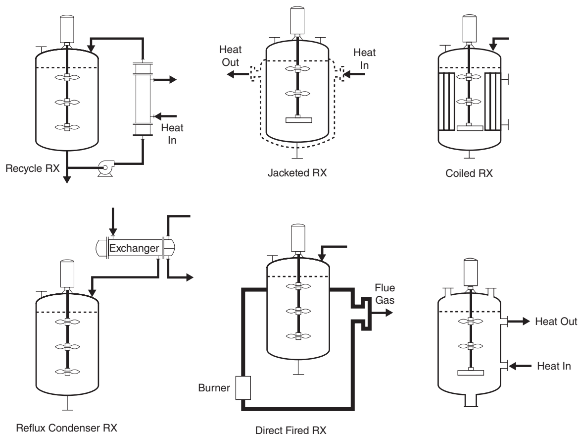
Figure 14.4 Batch Stirred Tank Reactors
