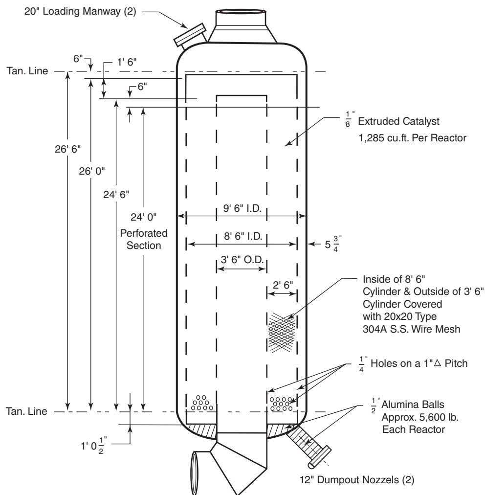
Figure 3.21 Radial Flow Reactor
