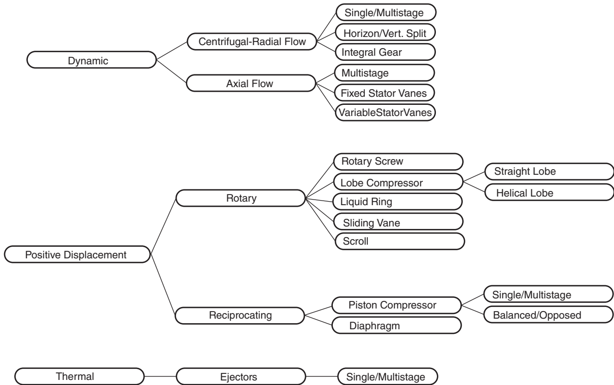
Figure 5.1 Compressor Family Tree
