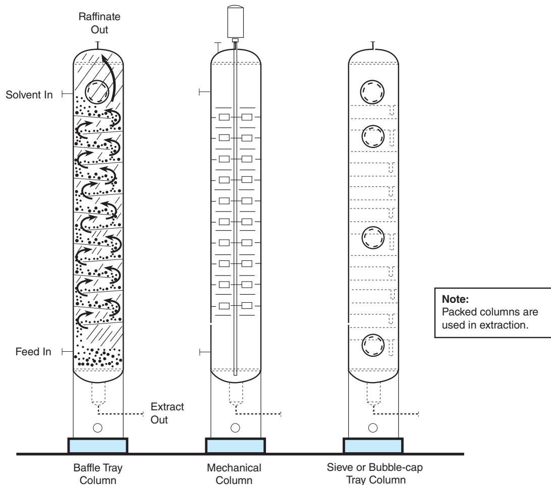
Figure 16.5 Extraction Columns
