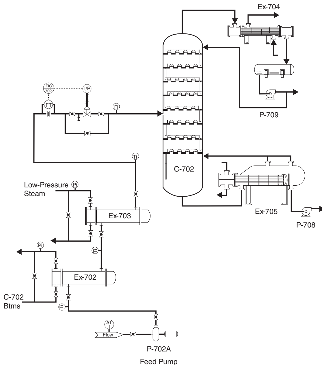
Figure 15.23 Distillation Process
