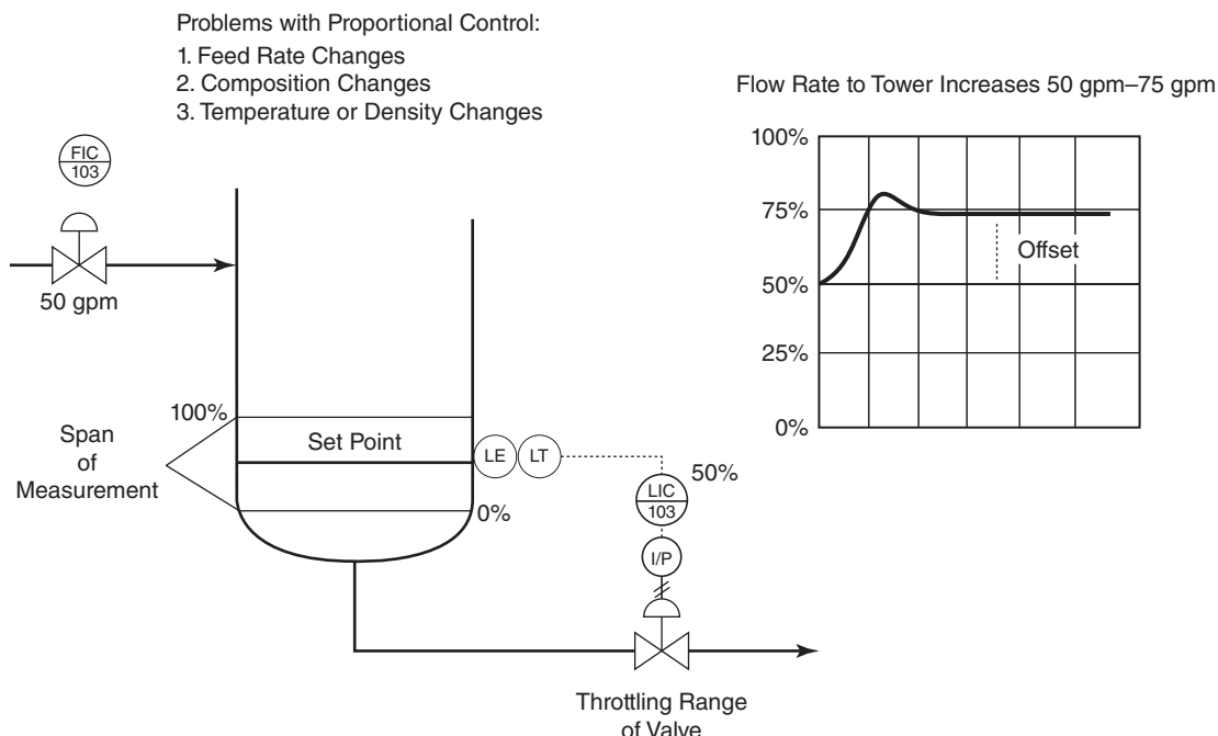
Figure 11.24 Proportional Control
