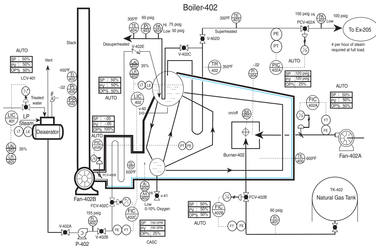
Figure 9.11 Steam Generation System: Boiler B-402
