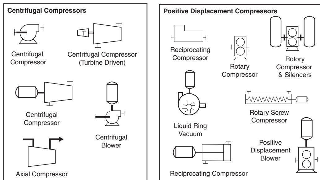
Figure 5.19 Compressor Symbols
