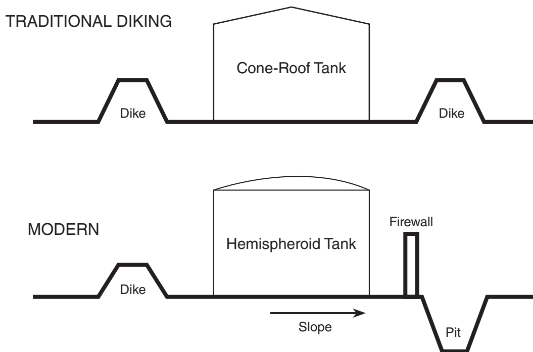
Figure 3.8 Traditional and Modern Diking Techniques
