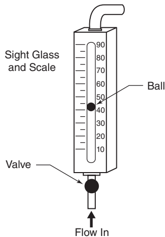
Figure 11.14 Rotameter
