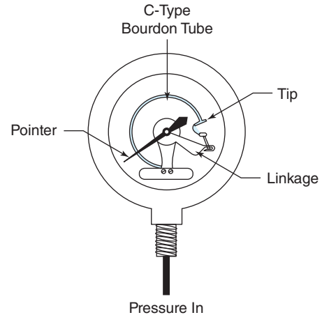
Figure 11.7 Bourdon Tube-type Pressure Elements
