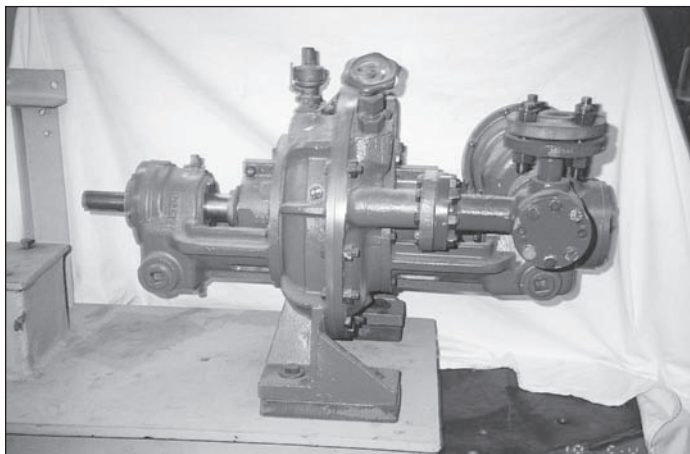
Figure 1.9 Steam Turbine
