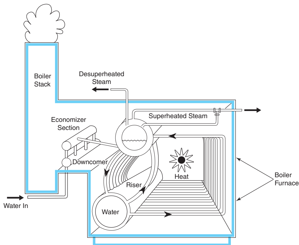
Figure 9.4 Water-Tube Boiler
