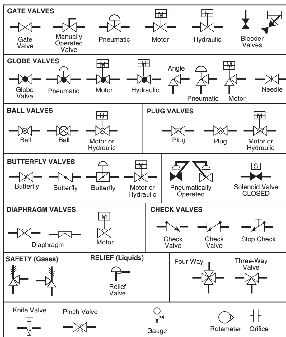
Figure 2.28 Valve Symbols
