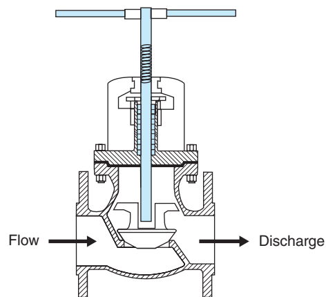
Figure 2.13 Stop Check Valve
