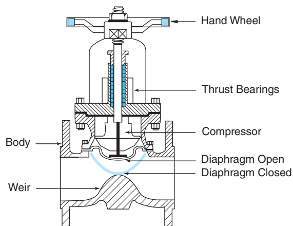
Figure 2.19 Diaphragm Valve Components
