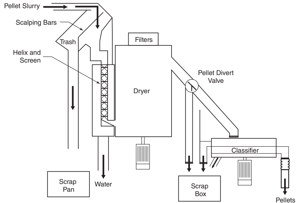
Figure 17.9 Dryer and Classifier System
