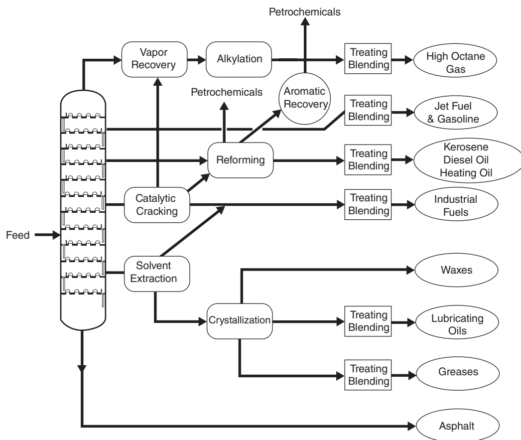
Figure 15.4 Modern Fractional Distillation
