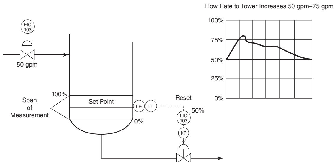
Figure 11.25 Reset
