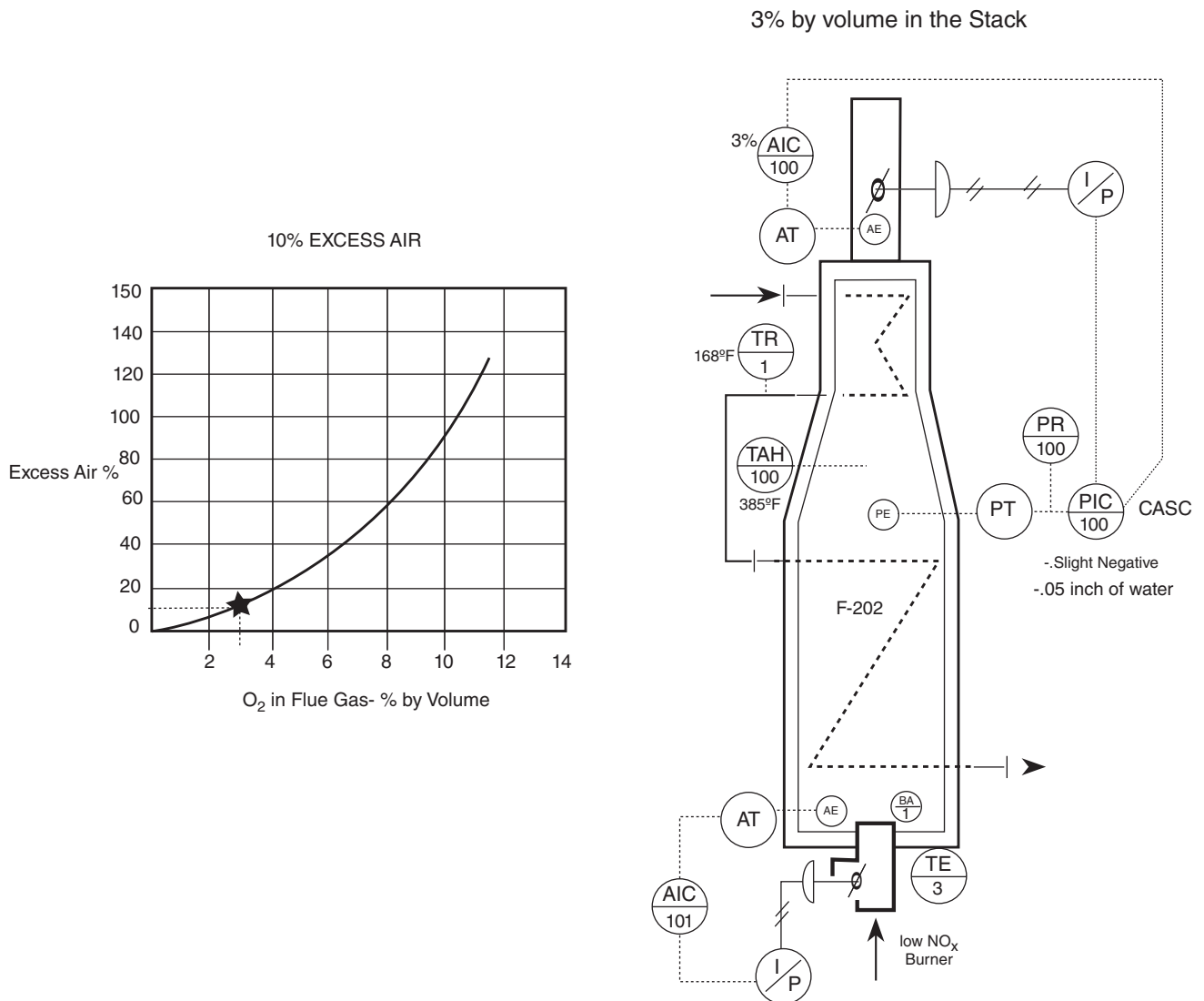
Figure 10.3 Air-to-Fuel Ratio Chart
