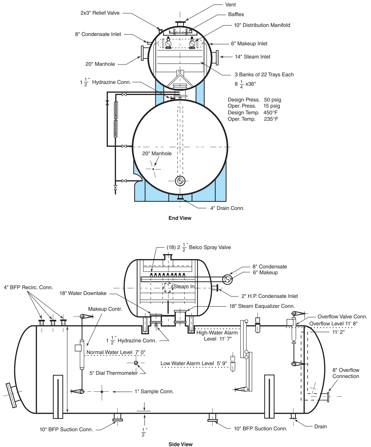
Figure 3.15 Deaerator in Boiler Feed-Water Plant
