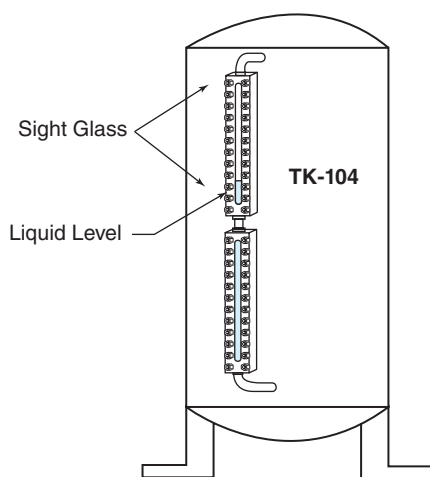
Figure 11.18 Sight Glass
