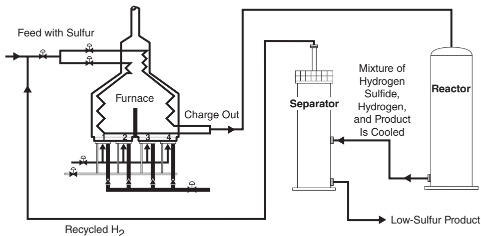
Figure 14.8 Hydrodesulfurization
