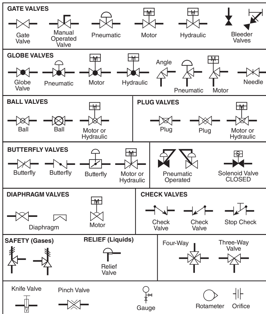
Figure 12.10 Valves
