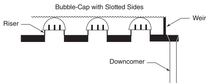
Figure 15.12 Bubble-Cap Tray
