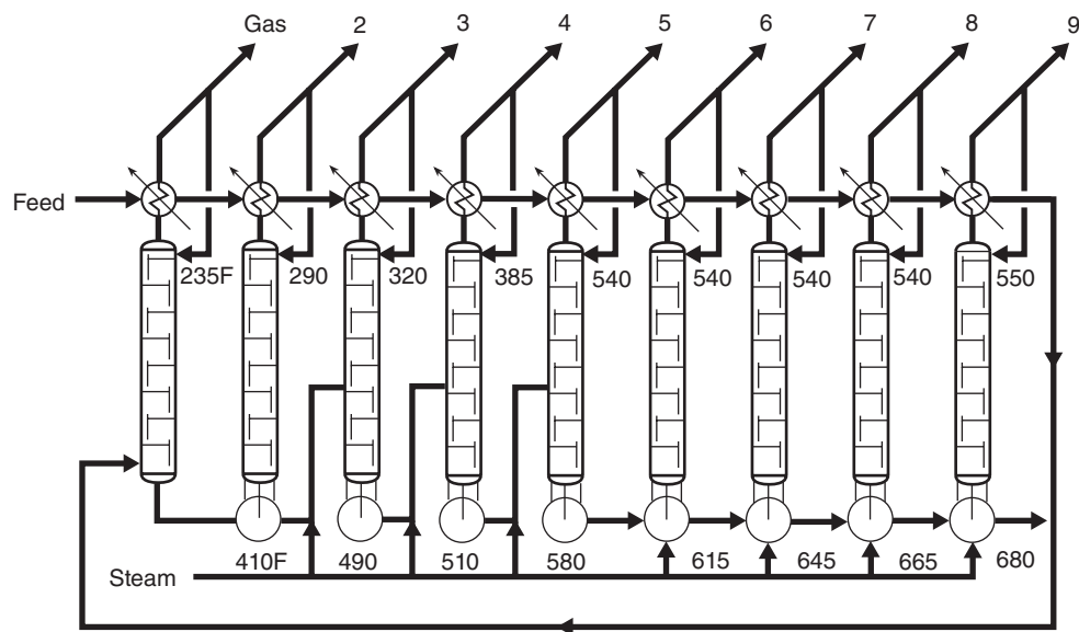
Figure 15.3 Continuous Batch Distillation
