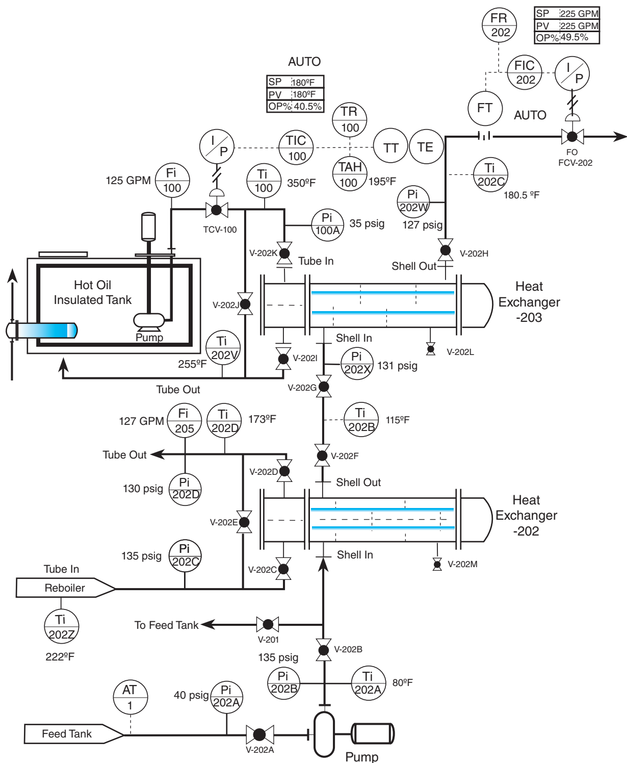
Figure 7.24 Heat Exchanger System
