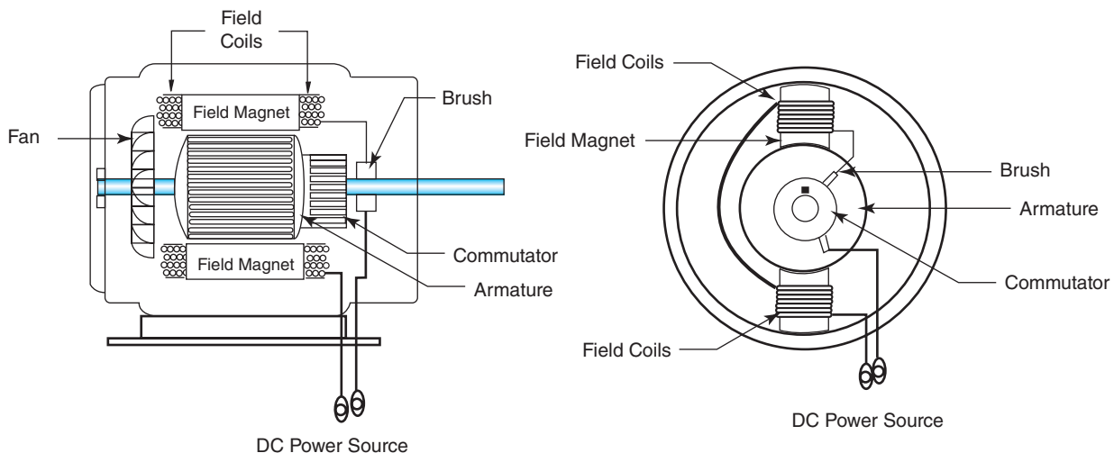
Figure 6.10 DC Motor
