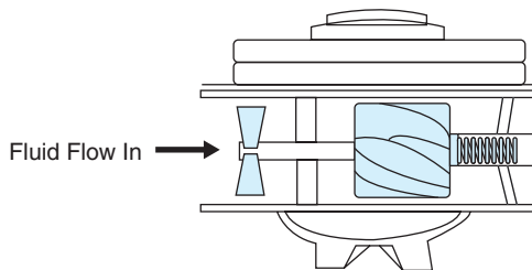
Figure 11.15 Turbine Flow Meter
