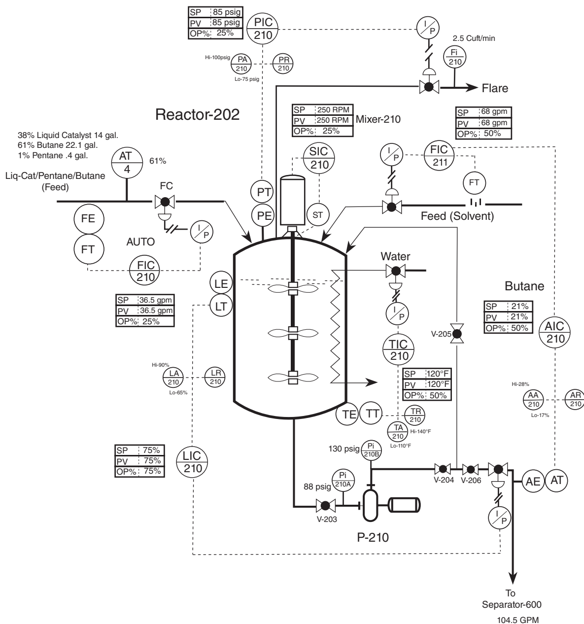
Figure 14.16 Stirred Reactor System
