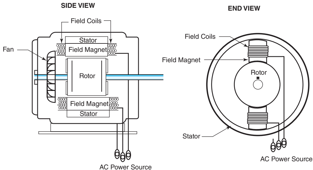
Figure 1.5 AC Motor
