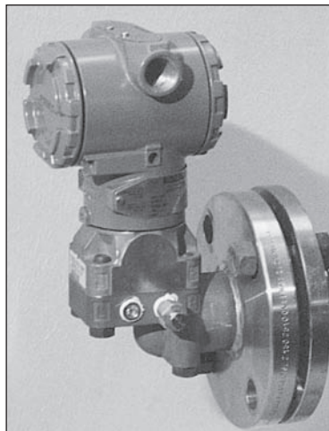
Figure 11.22 \Delta P Cell Transmitter
