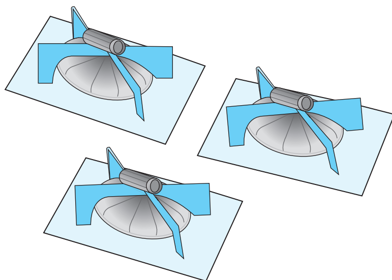
Figure 15.12 Bubble-Cap Tray
