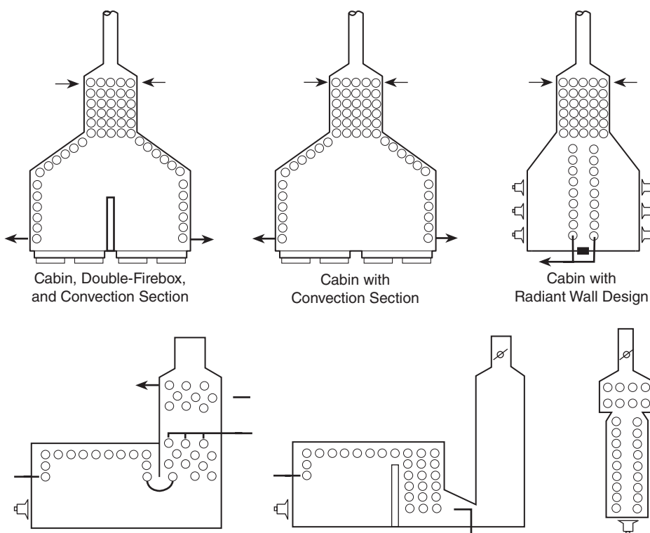
Figure 10.14 Furnace Designs
