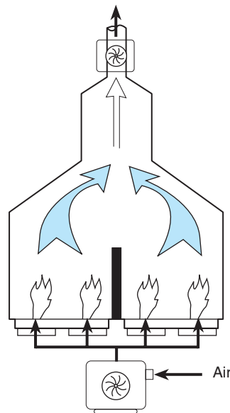
Figure 10.9 Balanced-Draft Furnace
