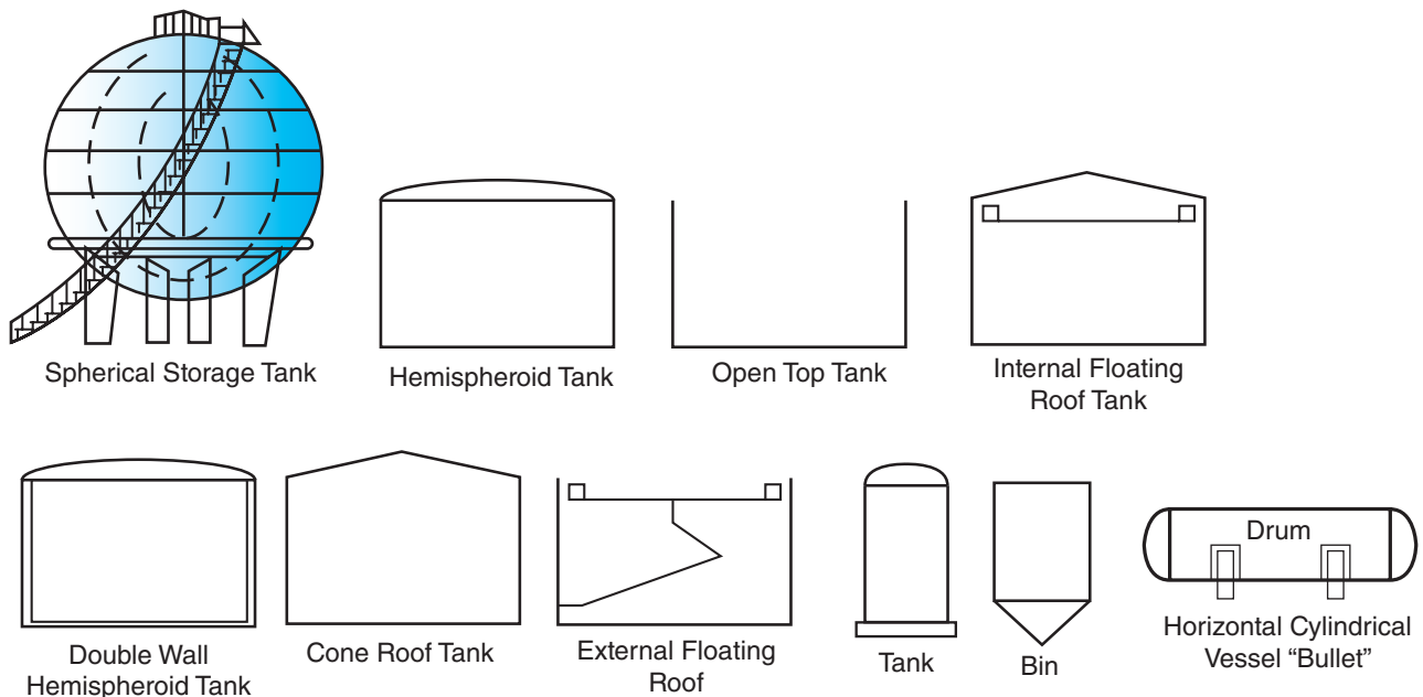
Figure 1.13 Tank Designs
