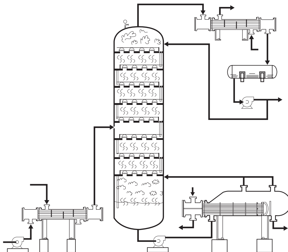
Figure 1.21 Distillation Column
