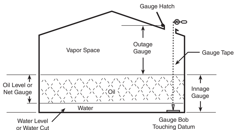
Figure 3.7 Tank Terminology
