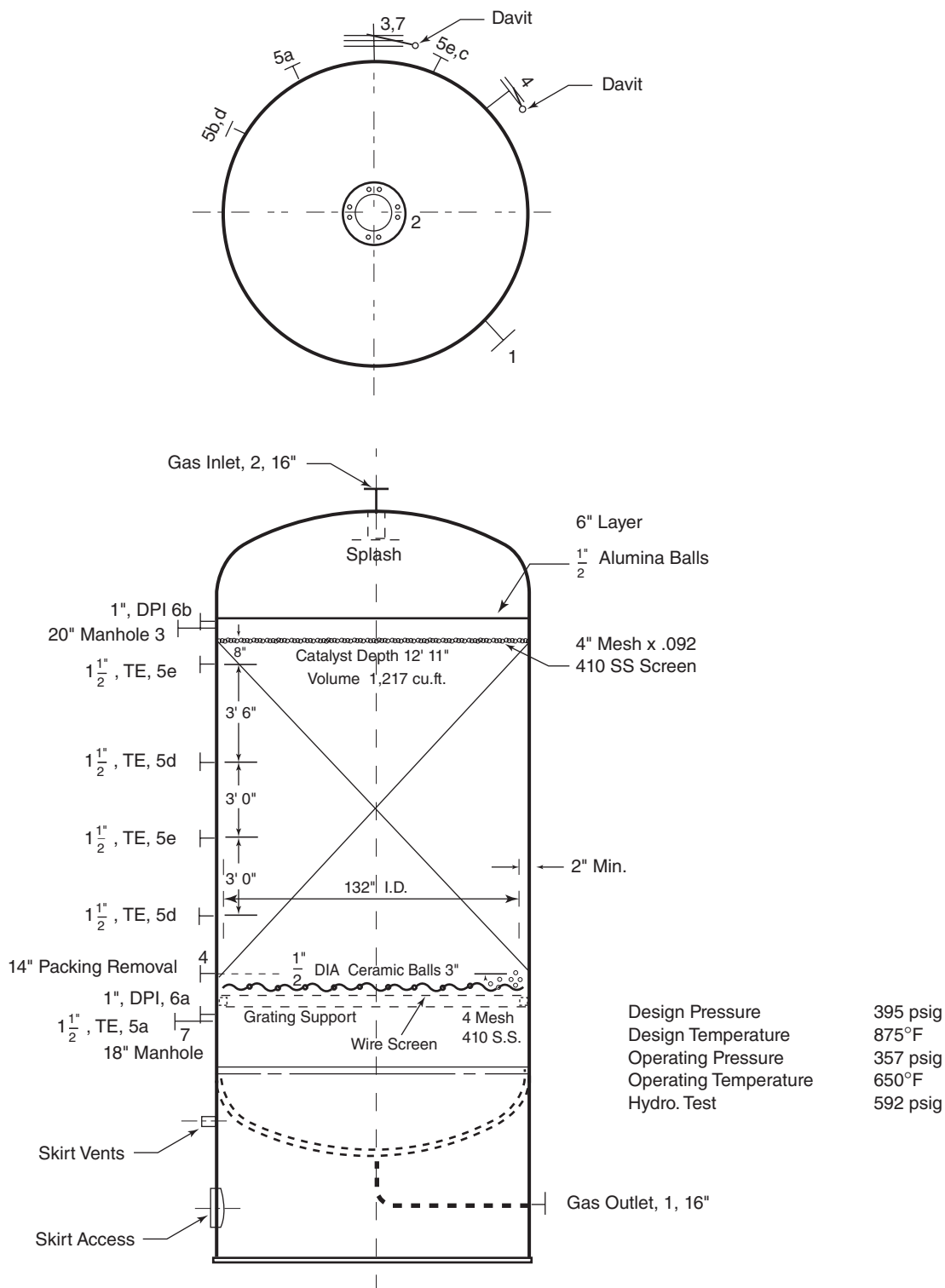
Figure 3.20 Fixed Bed Reactor
