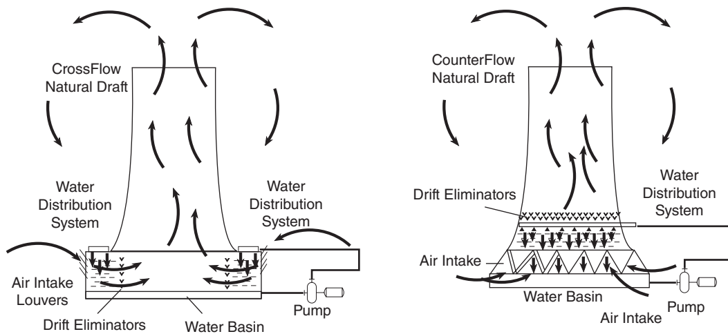
Figure 8.4 Natural-Draft Cooling Tower
