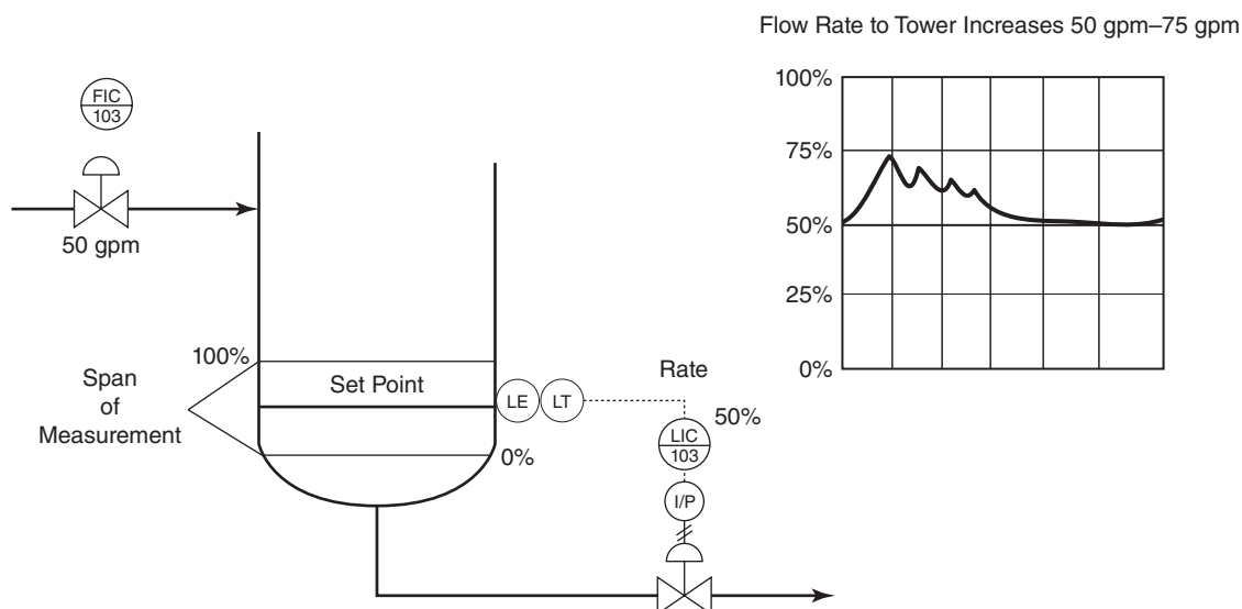
Figure 11.26 Rate
