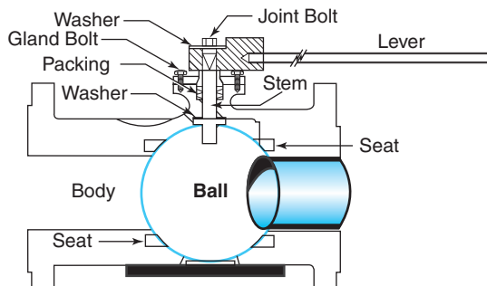
Figure 2.8 Ball Valve Components
