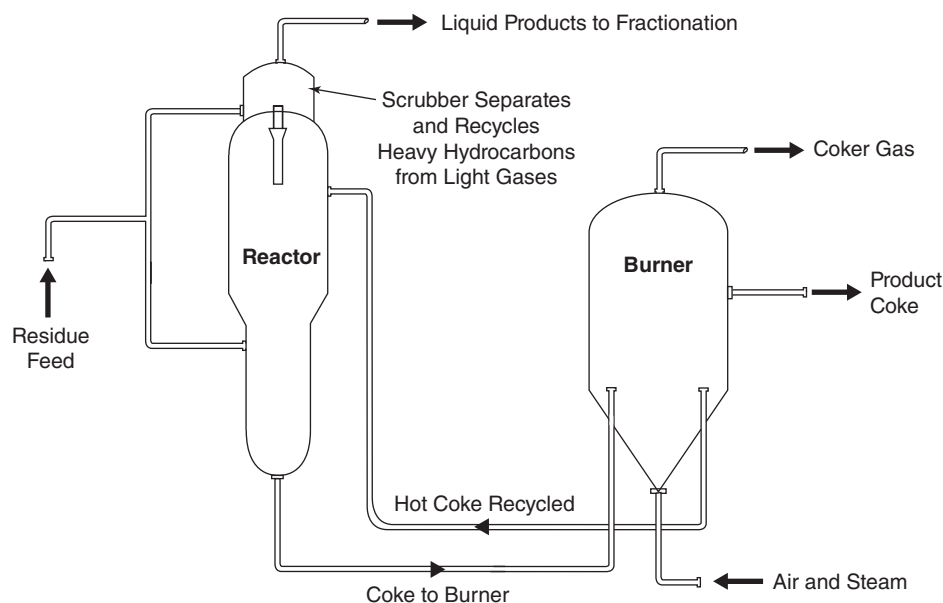
Figure 14.12 Fluid Coking
