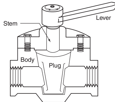
Figure 2.17 Plug Valve Components
