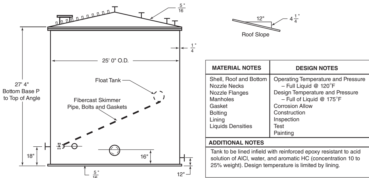
Figure 3.13 Storage Tank with Internal Skimmer
