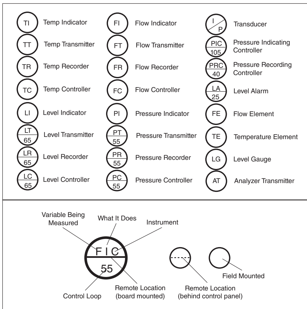
Figure 12.1 Process and Instrument Symbols (continued)
