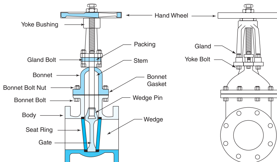
Figure 2.2 Gate Valve Components
