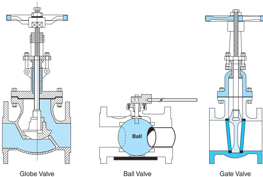
Figure 1.14 Valves
