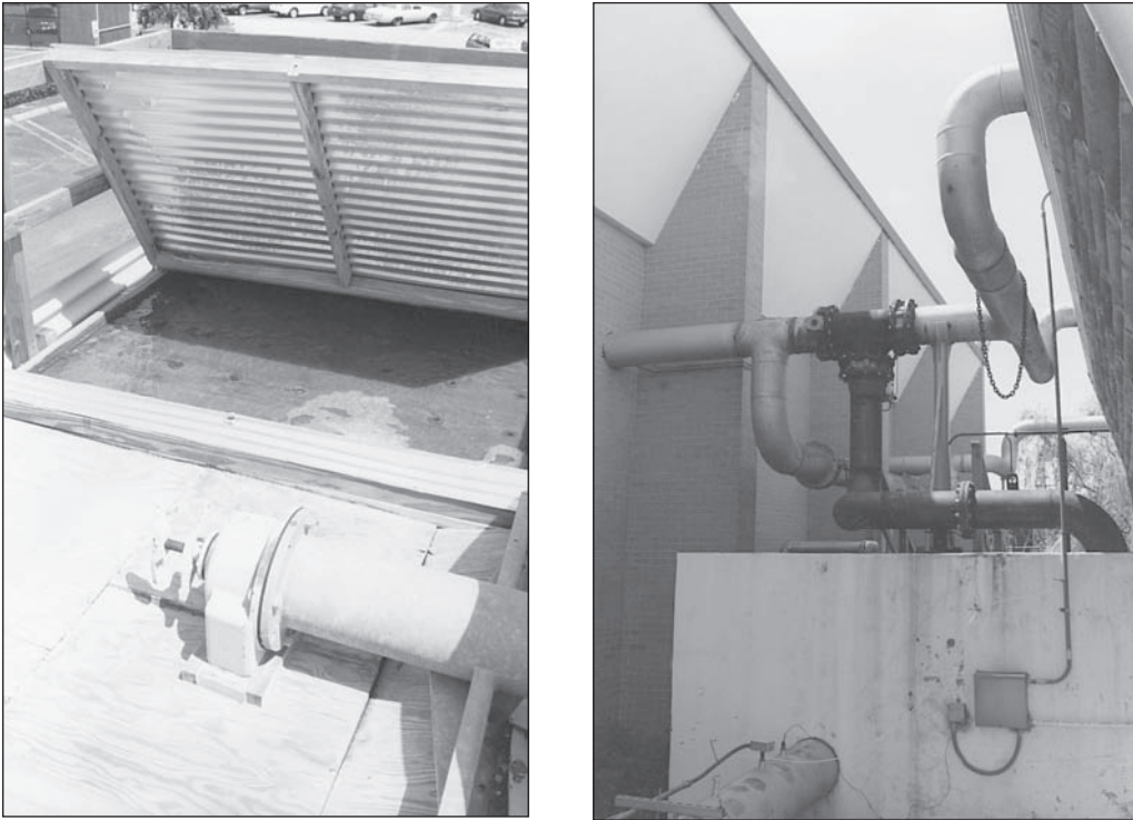
Figure 8.2 Water Distribution System
