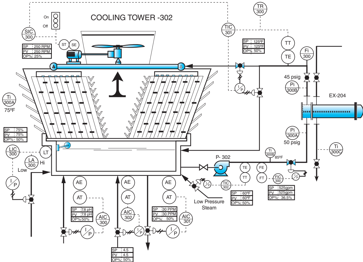
Figure 8.10 Cooling Tower System: CTW-302
