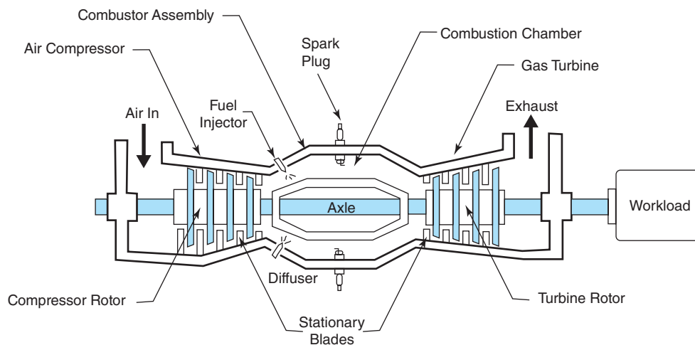
Figure 6.8 Gas Turbine Components
