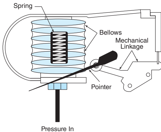
Figure 11.6 Bellows Pressure Elements
