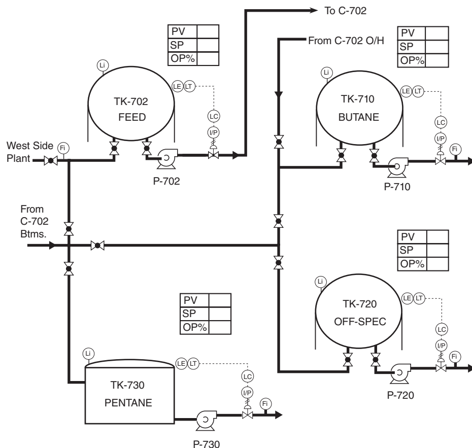
Figure 15.21 Feed System
