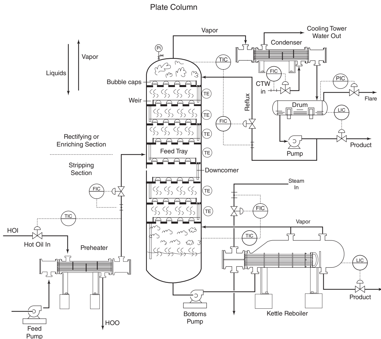
Figure 15.9 Plate or Tray Column
