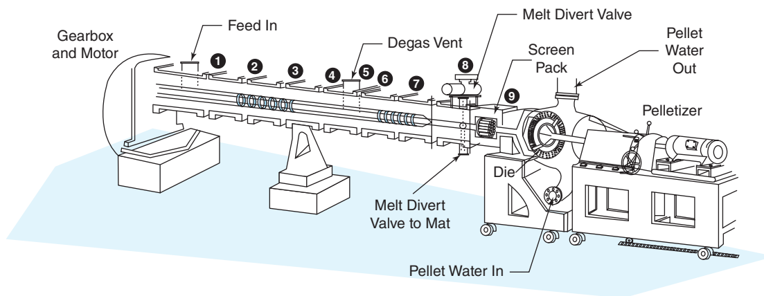
Figure 17.4 Extruder
