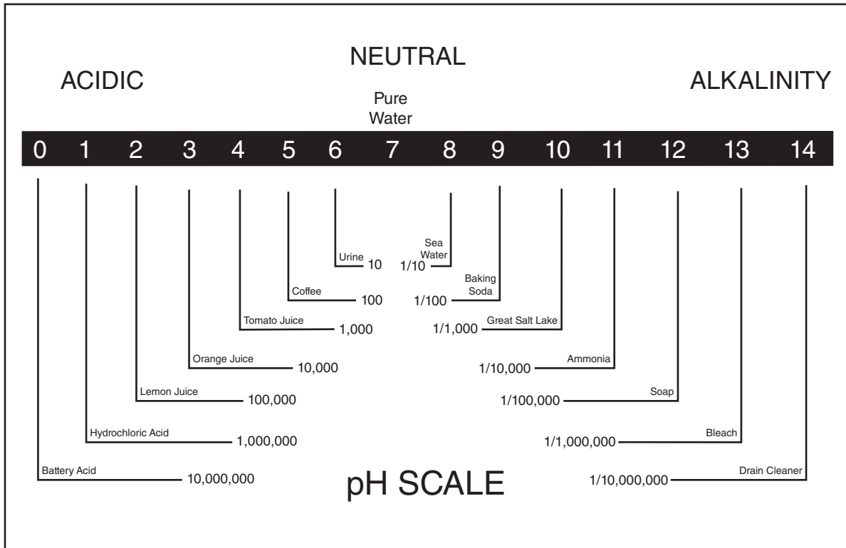
Figure 8.12 pH Scale
