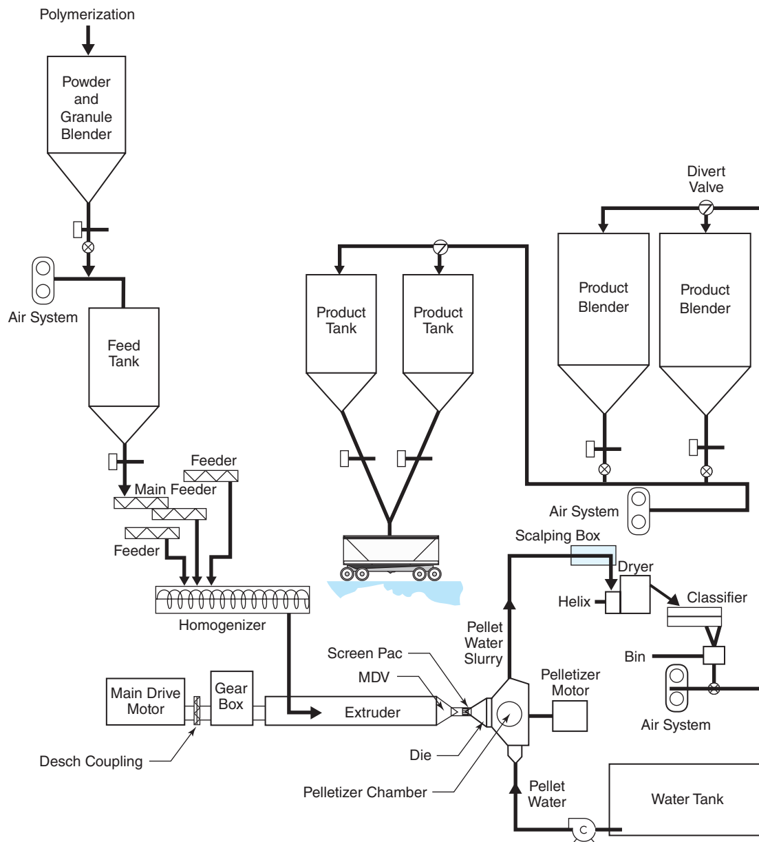
Figure 17.2 Finishing Section
