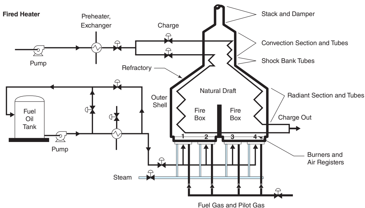
Figure 10.10 Cabin Furnace
