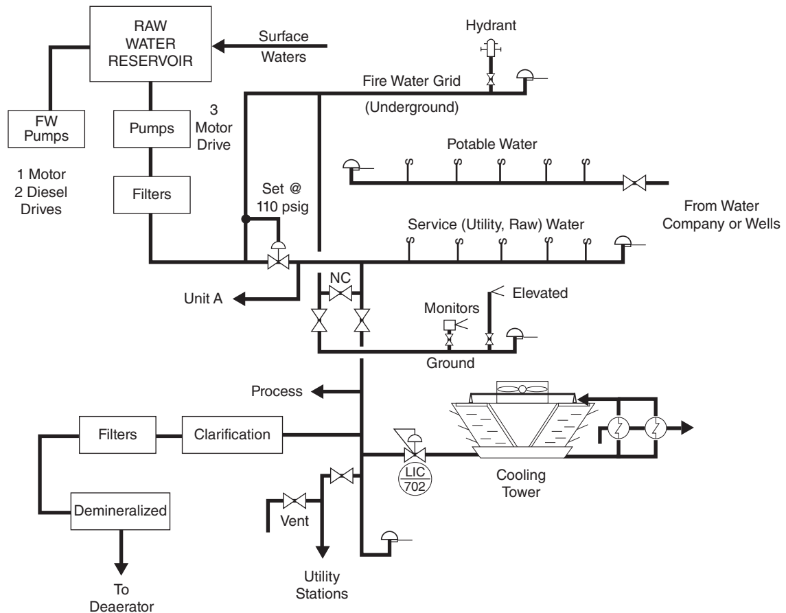
Figure 13.2 Water Systems
