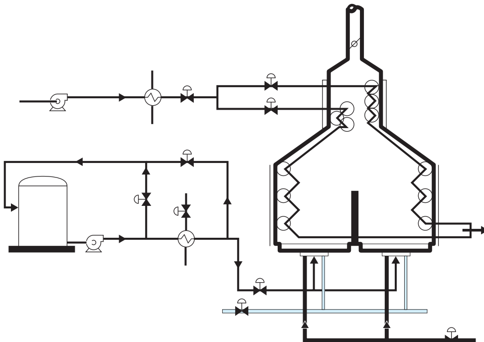
Figure 1.19 Fixed Heaters
