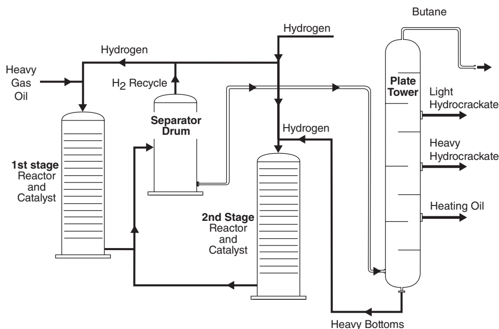
Figure 14.9 Hydrocracking
