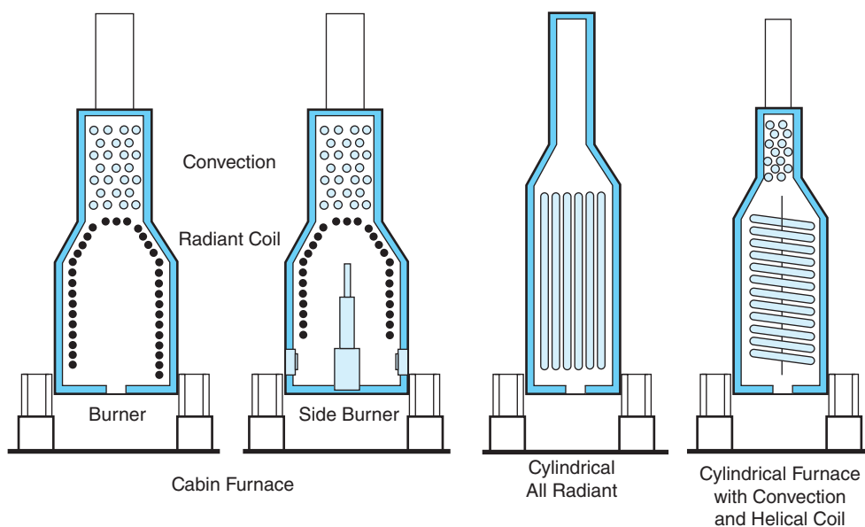
Figure 10.12 Cylindrical Furnace Designs
