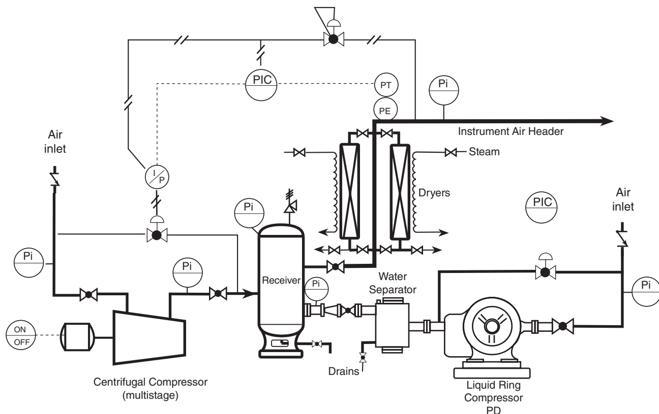
Figure 5.18 Compressor System
