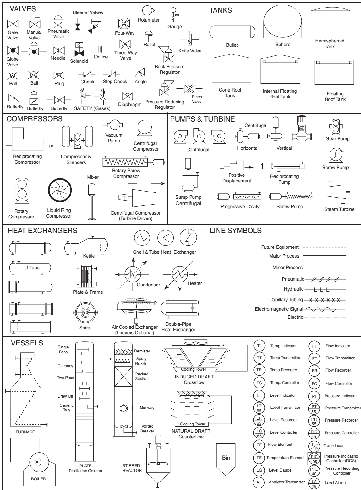
Figure 12.1 Process and Instrument Symbols
