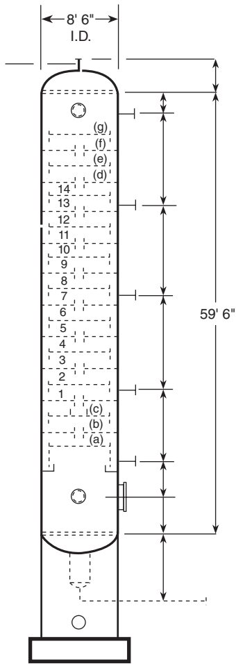
Figure 3.17 Distillation Column
