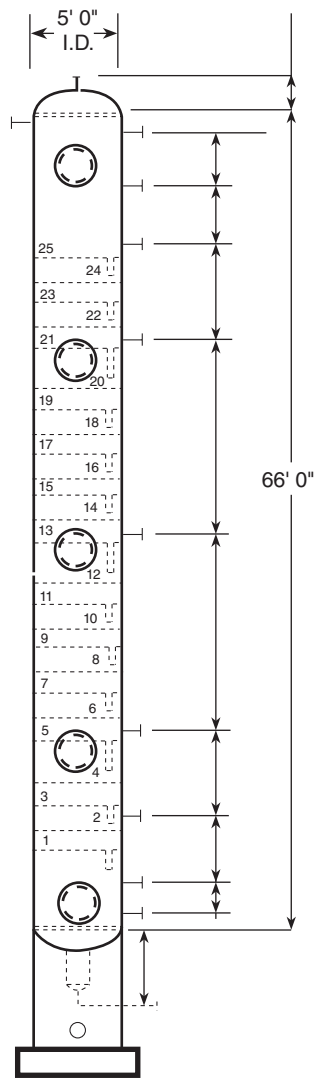
Figure 3.18 Extraction Column
