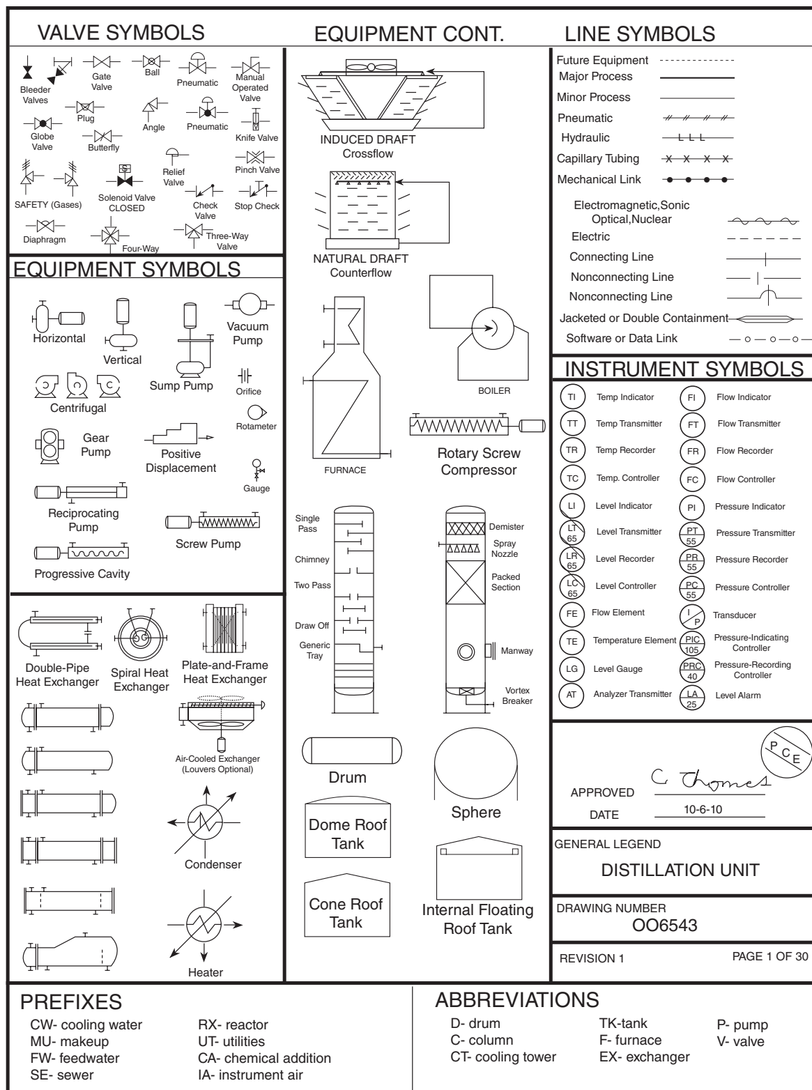
Figure 12.4 Process Legend
