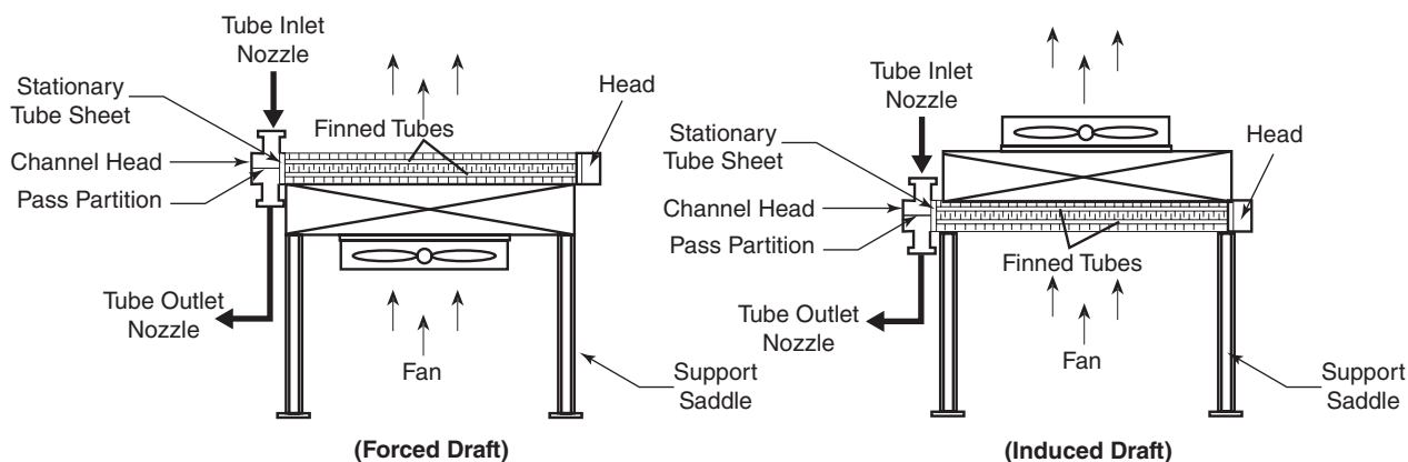
Figure 7.23 Air-Cooled Heat Exchanger
