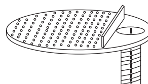
Figure 15.13 Sieve Tray and Downcomer
