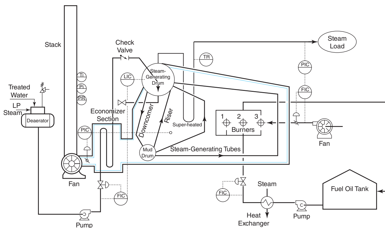
Figure 9.7 Steam System
