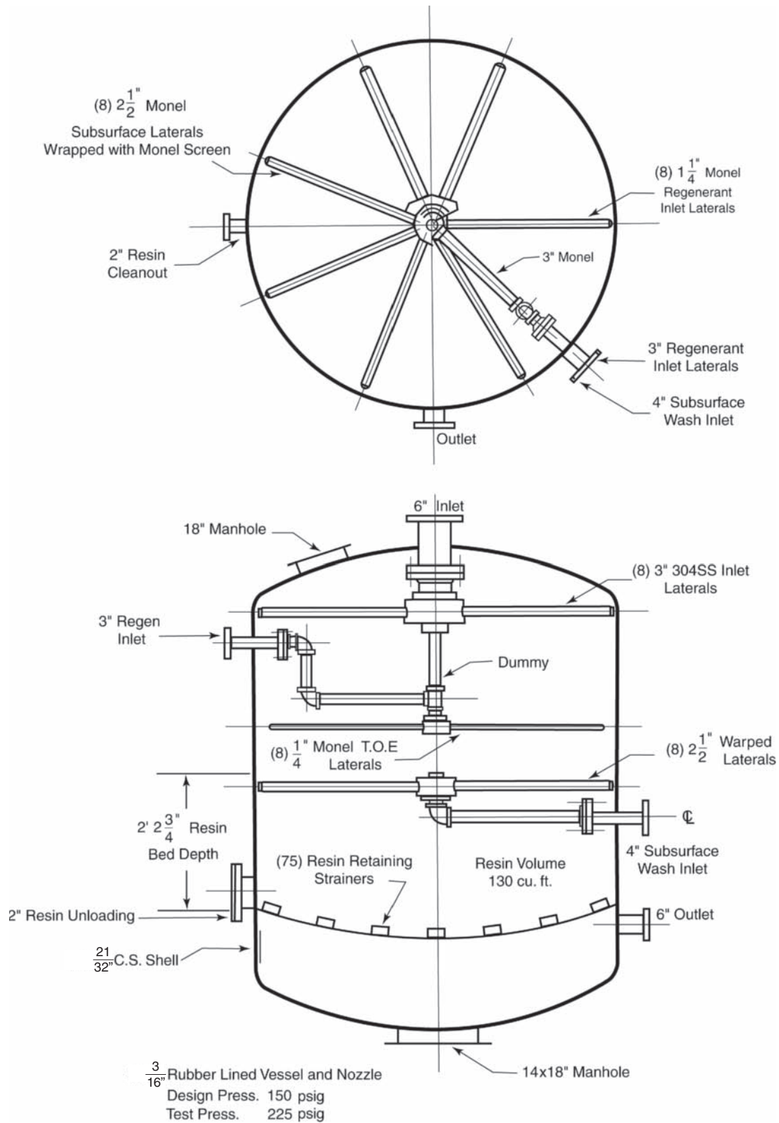
Figure 3.14 Storage Tank
