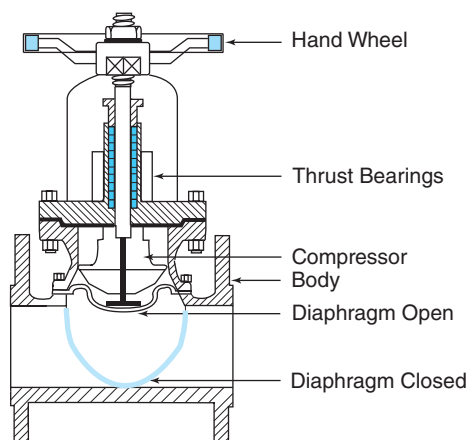
Figure 2.20 Straight-Through Diaphragm Valve
