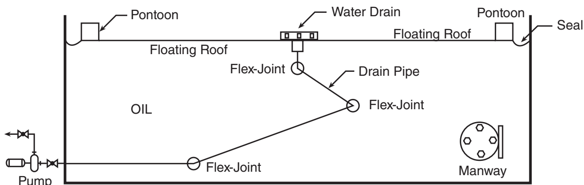
Figure 3.4 Floating-Roof Tank Components
