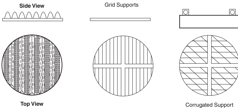
Figure 15.18 Packing Supports
