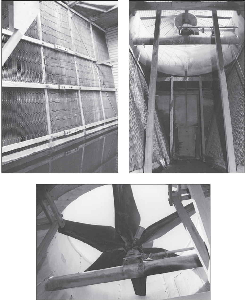
Figure 8.8 Internal View of Induced-Draft, Crossflow Cooling Tower
