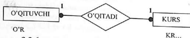
2.2.6-rasm. ER-tur diagrammasiga misol.
