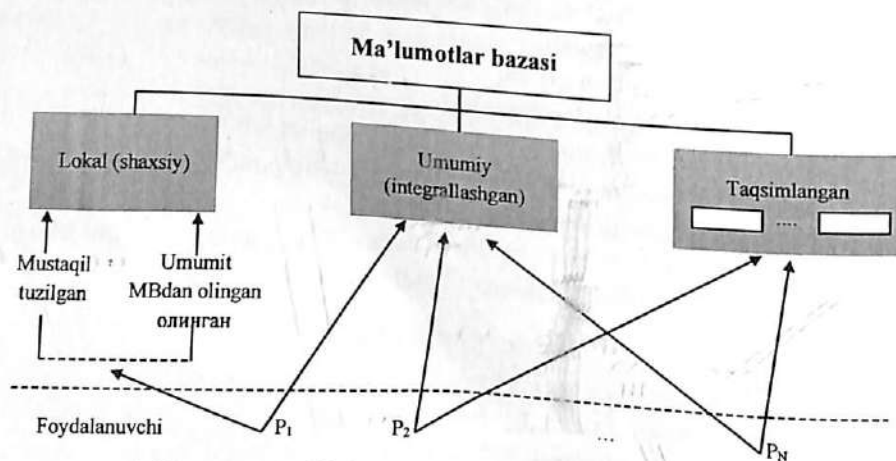
1.10-rasm. Tashkiliy jihatdan MBning turkumlanishi
