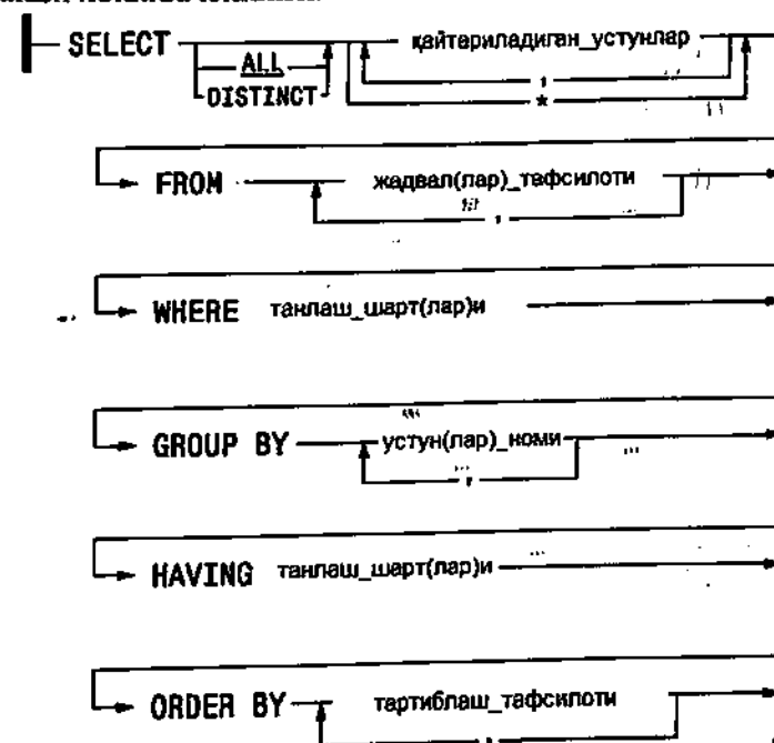
4.3.2-rasm. SELECT operatorining sintaksis diagrammasi
