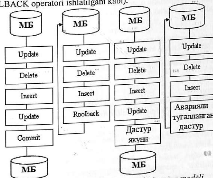
6.1.1-rasm. ANSI/ISO tranzaktsiyaning modeli
