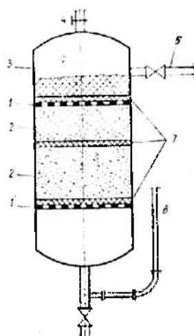
3.16-rasm. Qumli filtr.
