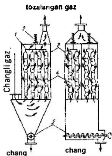
3.32-rasm. Yengli filtr.
