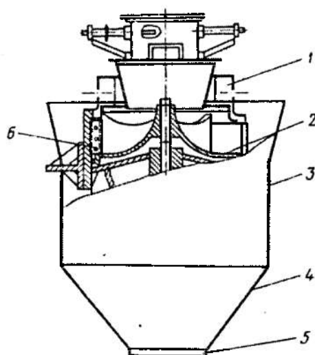
7.12-rasm. Markazdan qochma, romli kesgich.
