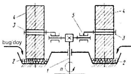
7.10-rasm. Yuguruvchi tegirmon.
