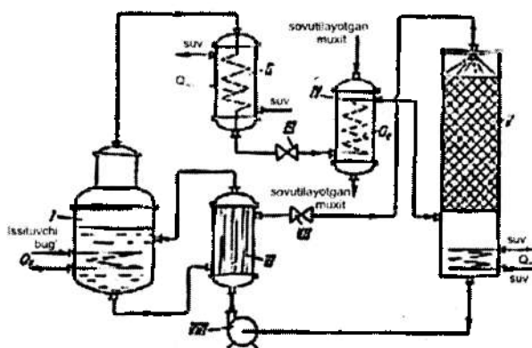
10.9-rasm. Suv-ammiak absorbsion sovitish mashinasining sxemasi: I - qaynatkich; II - kondensator; III, VII - rostlovchi ventillar; IV - bug'latkich; V - absorber; VI - isitkich; VIII - nasos.
