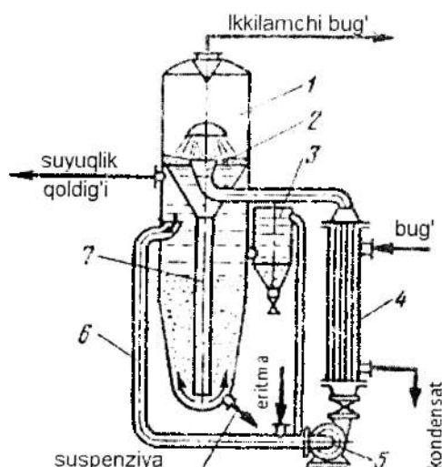
5.154-rasm. Mavhum qaynash qatlamli kristallizator.
