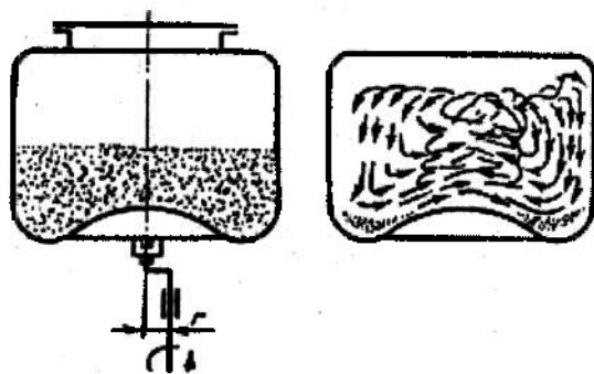
8.16-rasm. Drajje yasash granulatorida zarrachalarning harakat sxemasi.
