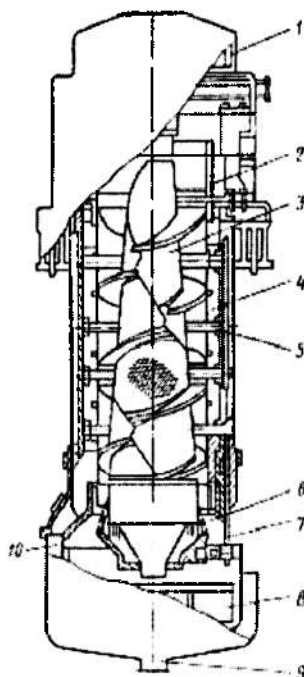
8.2-rasm. Vertikal shnekli press.
