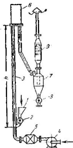
5.140-rasm. Pnevmatik quritkich. 1-bunker; 2-ta'minlagich; 3-truba; 4-ventilator; 5-kalorifer; 6-yig'gich-amortizator; 7-siklon; 8-to'kish moslamasi; 9-filtr.
