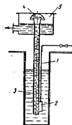
2.57-rasm. Havoli ko'targich.
