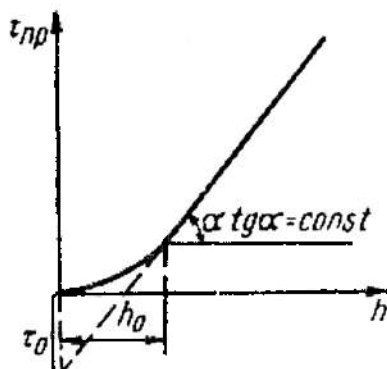
5.96-rasm. Himoyalovchi ta'sir davomiy-ligining adsorbent qatlami balandligiga bog'liqligi.
