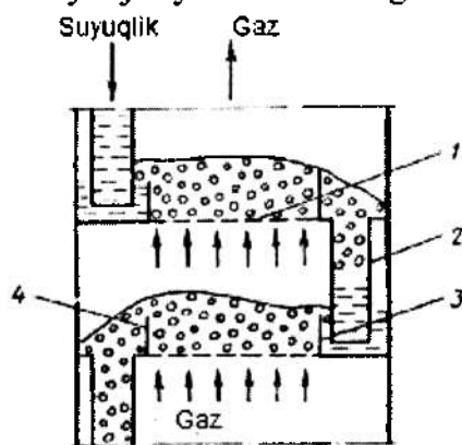
5.23-rasm. Elaksimon tarelkali kolonna.
