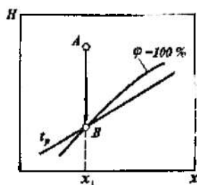
5.115b-rasm. I-x diagrammada shudring nuqtasini aniqlash.
