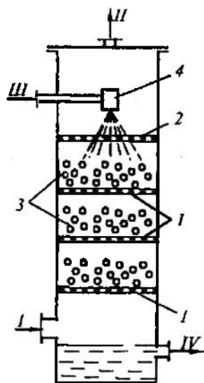
5.38-rasm. Sharsimon nasadkali mavhum qaynash qatlamli absorber.
