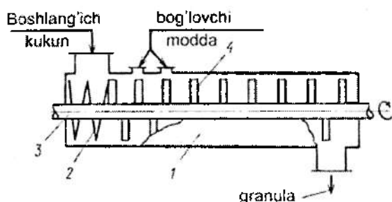
8.15-rasm. Turboparrakli tezkor granulyator. 1-qobiq; 2-shneck; 3-rotor o'qi; 4-rotor sterjenlari.
