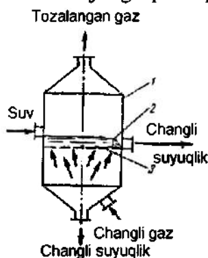
3.35-rasm. Ko'pikli skrubber.
