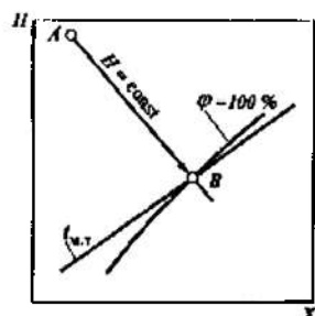
5.115d-rasm. I-x diagrammada ho‘l termometr temperaturasi aniqlash.
