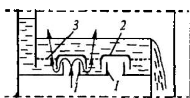
5.37-rasm. Elaksimon-qalpoqchali tarelka.
