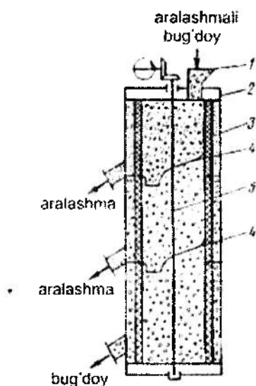
7.17-rasm. Barabanli g'alvir 1-yuklash shtutseri; 2-qibiq; 3-baraban; 4-kanalli to'siq; 5-o'q.
