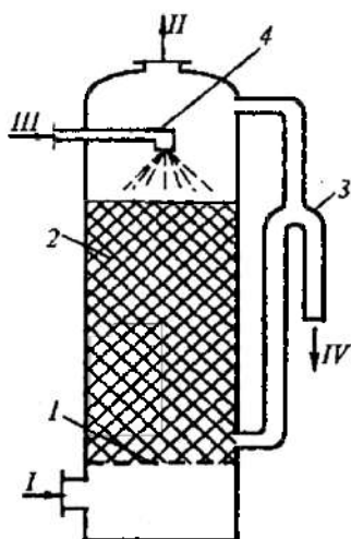
5.39-rasm. Nasadkali emulgatsion absorber.
