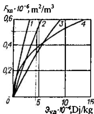
7.26-rasm. Solishtirma yuza F_{ud} o'sishining material solishtirma energiyasi E_{uk} sarfiga bog'liqligi. 1-apatit, gips, ohaktosh; 2-ohaktosh, mergel; 3-granit; 4-toshko'mir.
