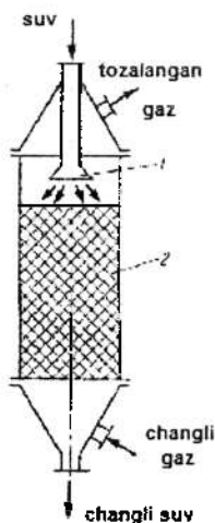
3.34a-rasm. Nasadkali scrubber.
