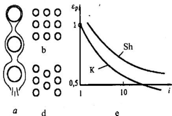
4.18-rasm. Truba o'rami trubasining tashqi yuzasida kondensatsiyalanish.
