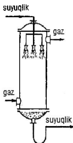
5.40-rasm. Purkovchi absorber.
