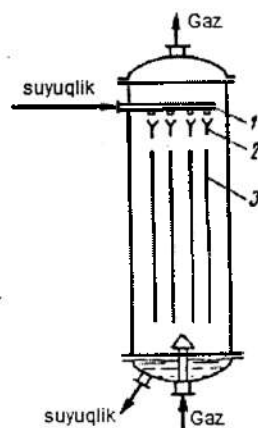
5.18-rasm. Yupqa qatlamli tekis parallel nasadkali absorber.
