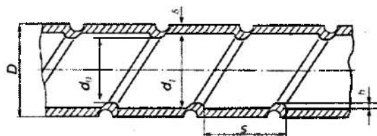
5.33-rasm. Spiralsimon turbulizatorli truba.
