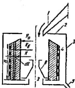
3.9-rasm. Filtrlovchi sentrifuga. 1-suspensiya berish trubasi; 2-cho'kma tushiradigan teshik; 3-qobiq; 4-rotor; 5-fugat chiqarish shtuseri; 6-konus.
