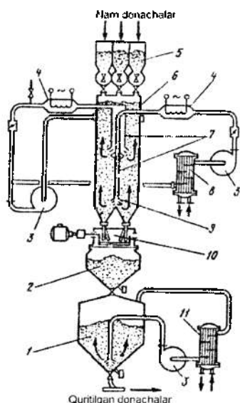
5.132-rasm. Sochiluvchan, donador materiallarni quritish uchun shaxtali quritkich.
