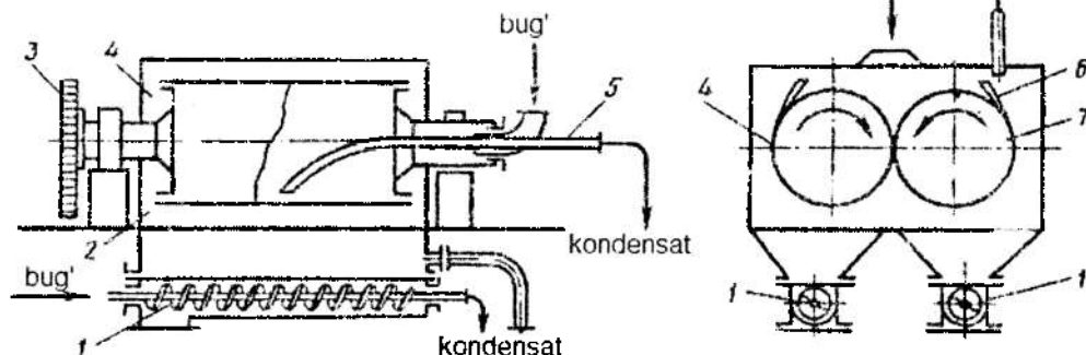
5.141-rasm. Juvali quritkich.
