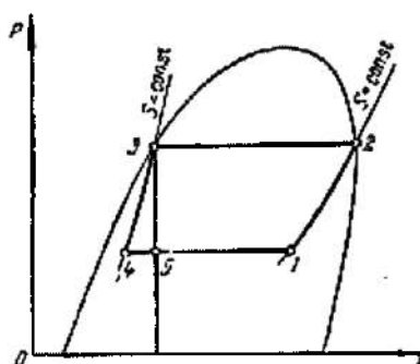
10.5-rasm. p-i diagrammadagi kompressor sovitish mashina sikli.
