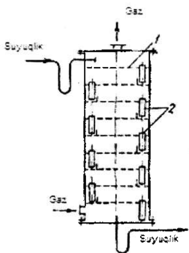
5.22-rasm. Quyilish moslamali, tarelkali absorber.
