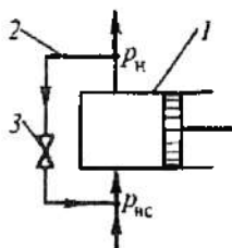
2.47-rasm. Porshenli nasoslar unumdorligini baypas shahobchasida ventil yordamida rostdlash.
