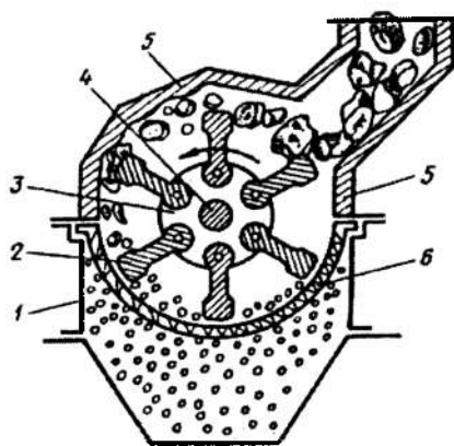
7.6-rasm. Bolg'ali maydalagich.
