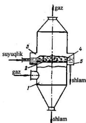
3.35a-rasm. Elaxsimon (a) va quyilish (b) tarelkali ko'pikli skrubber. a) 1-qobiq; 2-purkash moslamasi; 3-tarelka.
