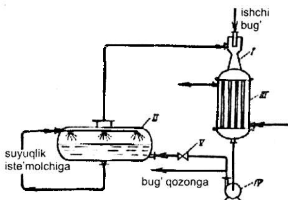
10.10-rasm. Suv-bug' injektor sovitish mashinasining sxemasi: I – injektor; II – bug'latkich; III – kondensator; IV – nasos; V – rostlovchi ventily.
