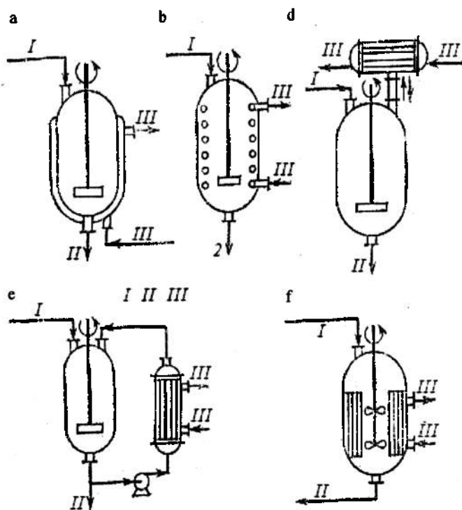
9.14-rasm. Aralashish reaktorining issiqlik almashinish moslamalari.
