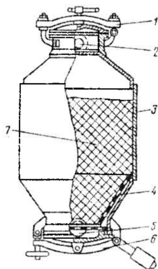
5.85-rasm. Perkolator.
