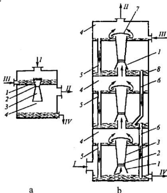
5.41-rasm. Venturi absorberi.
