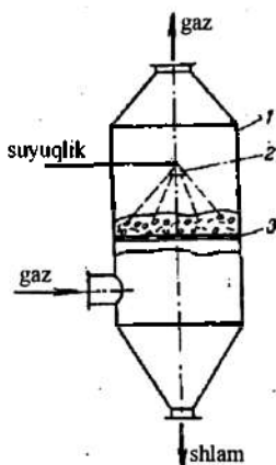
3.35a-rasm. Elaxsimon (a) va quyilish (b) tarelkali ko'pikli skrubber. a) 1-qobiq; 2-purkash moslamasi; 3-tarelka.
