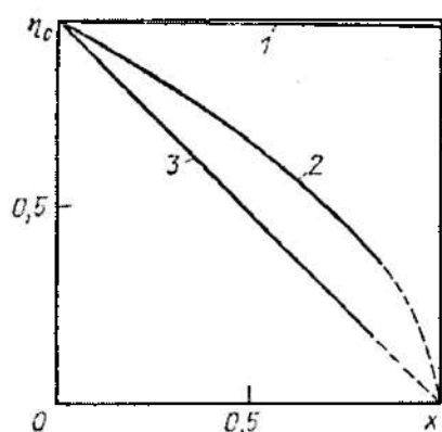
9.2-rasm. Ideal aralashtirish qurilma f.i.k. \eta_c ning reaksiyalar aylanish darajasiga bog'liqligi. 1-nol darajali; 2-birinchi darajali; 3-ikkinchi darajali.
