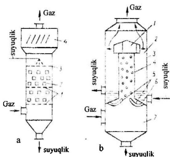
5.43-rasm. Harakatchan nasadkali (a) va tezkor (b) absorberlar.
