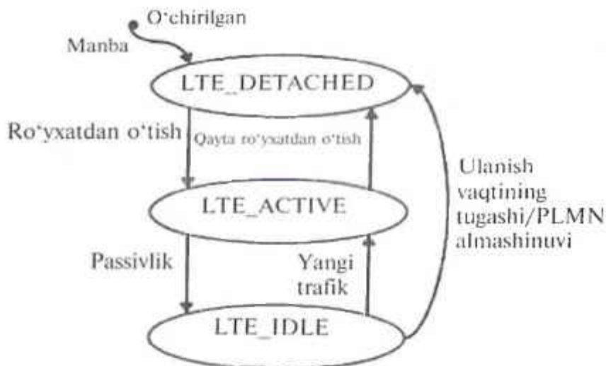
16.1-rasm. LTE tizimida AUning mobillik holatlari.
