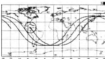
1.34-rasm. Orbitaning og'ish burchagi i=51^{\circ}
