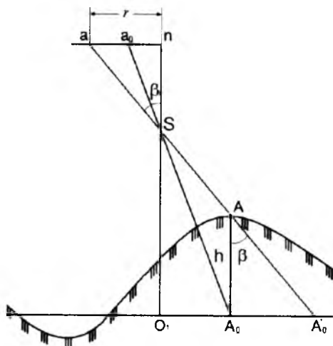
2.9-rasm. Tasvirdagi relyef taʼsirida nuqtaning siljishi
