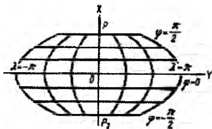
42-rasm. Pseudosilindrik proyeksiyalar koordinatalari tizimi
