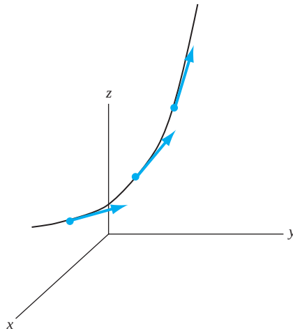
FIGURE 11.4 Curvature as a rate of change of the tangent vector.
