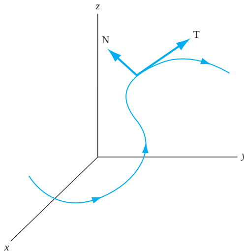
FIGURE 11.6 Unit tangent and normal vectors to a curve.
