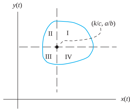
FIGURE 10.25 Typical predator/prey trajectory.
