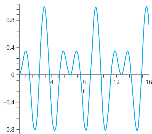
FIGURE 2.11 Beats.
