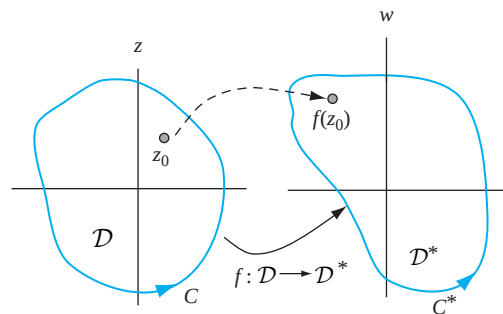
FIGURE 23.19 f : D \rightarrow D^* if f(z_0) is in D^* .
