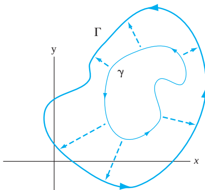
FIGURE 20.7 The deformation theorem.
