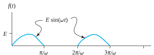
FIGURE 3.3 Function for Problem 19, Section 3.1.
