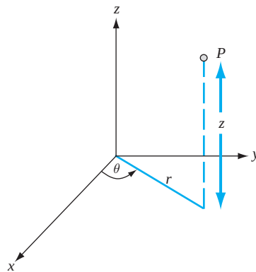
FIGURE 12.27 Cylindrical coordinates of Example 12.28.
