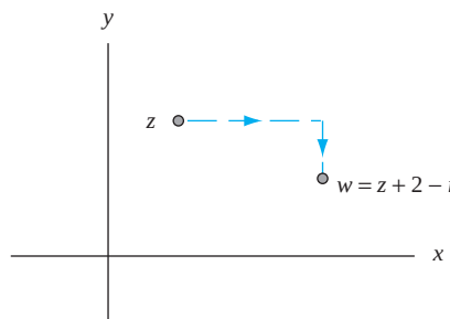
FIGURE 23.12 A translation.
