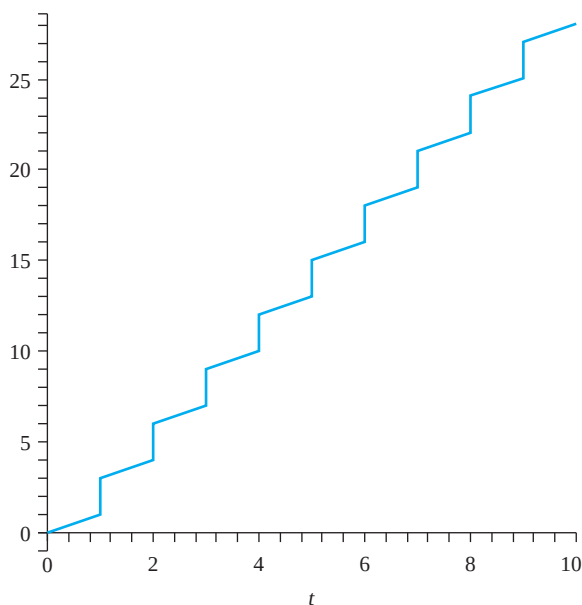
FIGURE 3.21 Replacement function.
