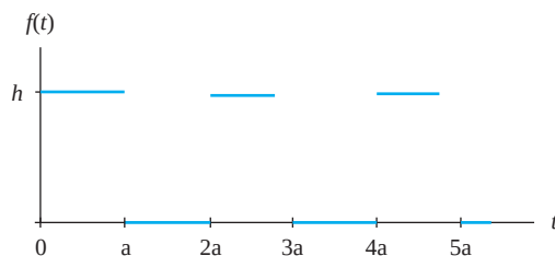
FIGURE 3.5 Function for Problem 21, Section 3.1.
