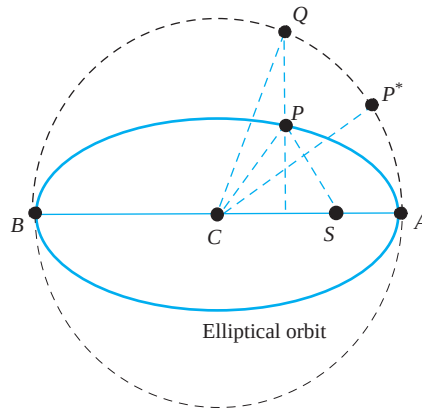
FIGURE 15.12 Kepler's problem.
