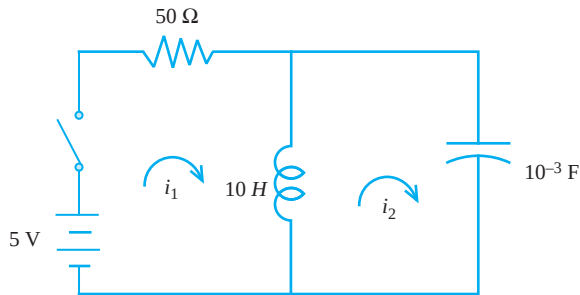
FIGURE 10.11 Circuit for Problem 9, Section 10.5.
