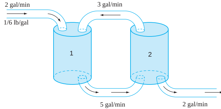
FIGURE 3.33 System of tanks in Problem 20, Section 3.6.
