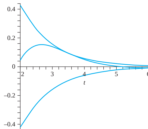
FIGURE 2.6 Underdamped, unforced motion in Example 2.20.
