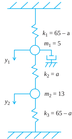
FIGURE 10.13 Mass/spring system for Problem 11, Section 10.5.
