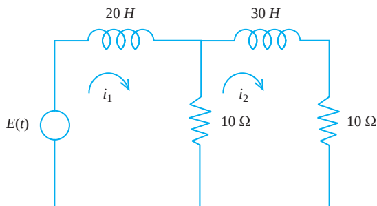
FIGURE 3.32 Circuit of Problem 18, Section 3.6.
