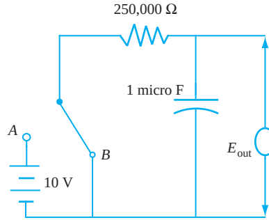
FIGURE 3.18 The circuit of Example 3.13.
