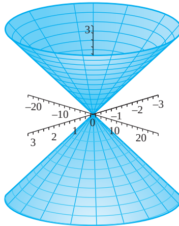
FIGURE 12.13 Elliptical cone z = au \cos(v) , y = bu \sin(v) , z = u .
