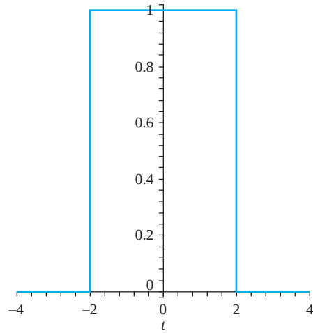
FIGURE 14.3 Window function w(t) in Example 14.11.
