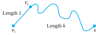
FIGURE 7.2 Constructing v_i - v_j walks of length k + 1 .
