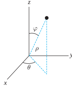
FIGURE 18.3 Spherical coordinates.
