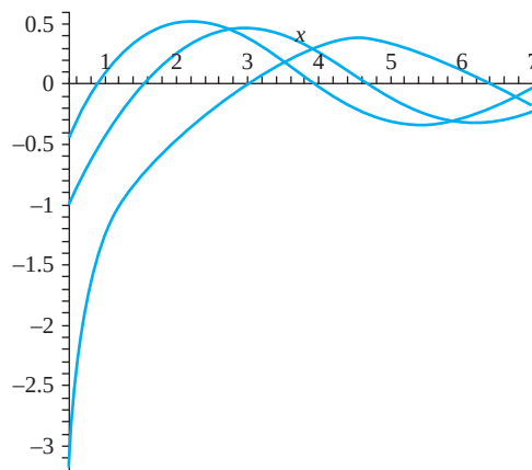
FIGURE 15.7 Y_\nu(x) for \nu = 0, 1/3, 1/2 .
