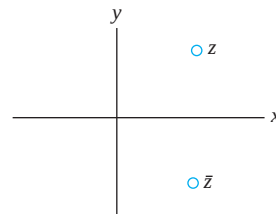
FIGURE 19.2 Complex conjugate.
