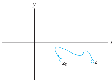
FIGURE 19.6 z \rightarrow z_0 along arbitrary paths.
