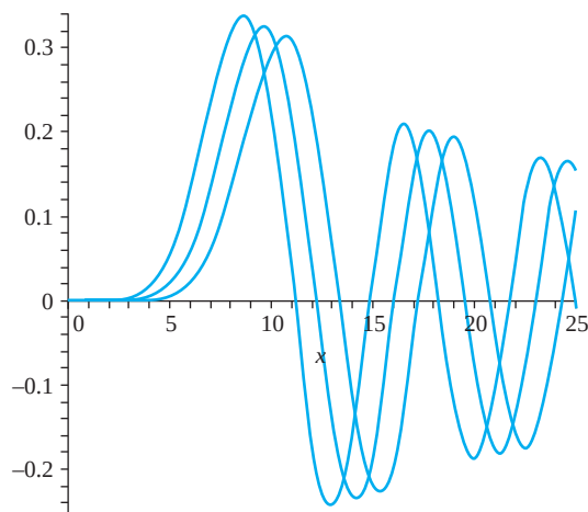
FIGURE 15.10 Interlacing lemma for J_7(x) , J_8(x) , and J_9(x) .
