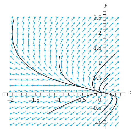
FIGURE 10.17 Phase portrait in Example 10.20.
