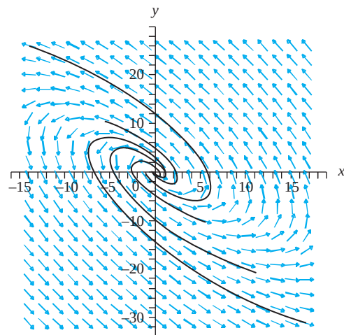
FIGURE 10.23 Spiral source in Example 10.23.
