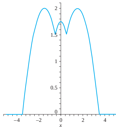
FIGURE 16.16 t = 1.5 .
