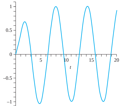
FIGURE 2.8 Critically damped, forced motion
