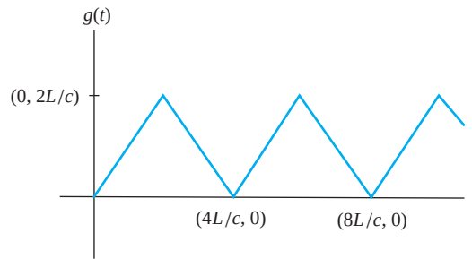
FIGURE 16.10 Sawtooth wave.
