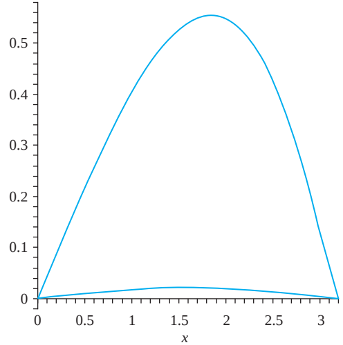
FIGURE 17.5 t = 1.3 .
