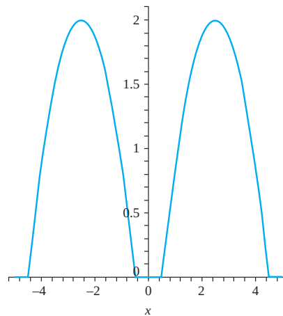
FIGURE 16.18 t = 2.5 .
