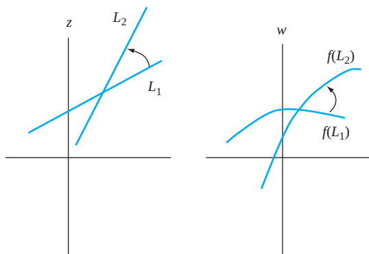
FIGURE 23.7 f preserves orientation.
