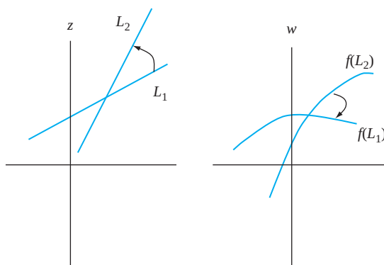
FIGURE 23.8 f fails to preserve orientation.
