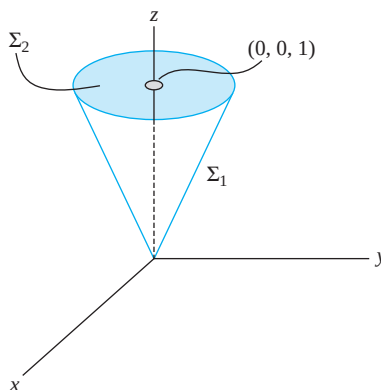
FIGURE 12.21 \Sigma in Example 12.24.
