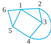
FIGURE 8.8 Graph of Problem 4, Section 8.6.
