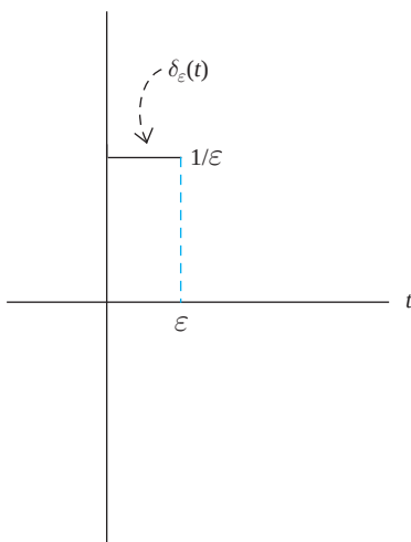
FIGURE 3.22 \delta_\epsilon(t)
