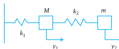
FIGURE 3.30 Mass/spring system in Problem 16, Section 3.6.
