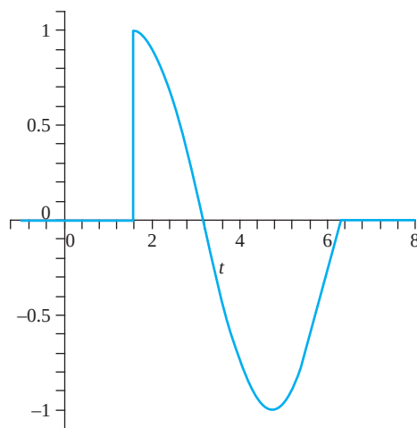
FIGURE 3.12 (H(t - \pi/2) - H(t - 2\pi)) \sin(t) .
