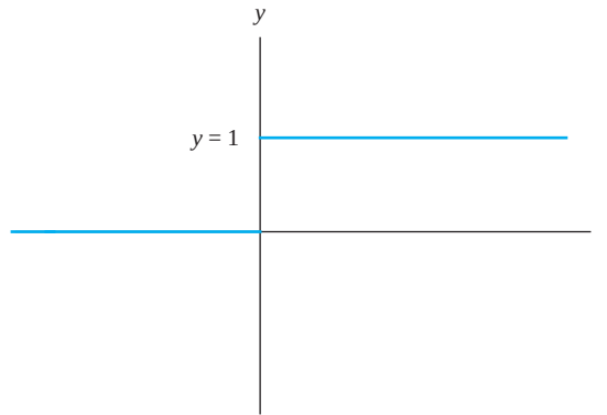
FIGURE 3.8 The Heaviside function.
