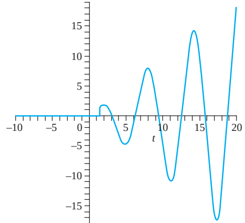
FIGURE 3.14 H(t - 3/2)t \sin(t) .
