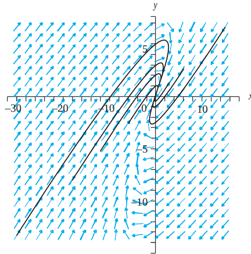
FIGURE 10.22 Improper node in Example 10.22.
