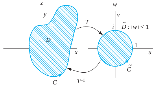
FIGURE 23.31 Solving a Dirichlet problem by a conformal mapping.
