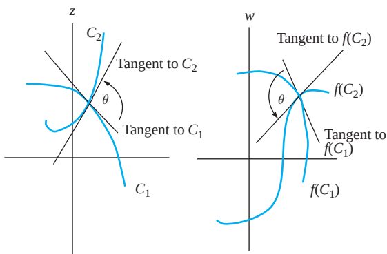
FIGURE 23.6 f preserves angles.
