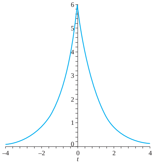
FIGURE 14.2 f(t) = 6e^{-|t|}
