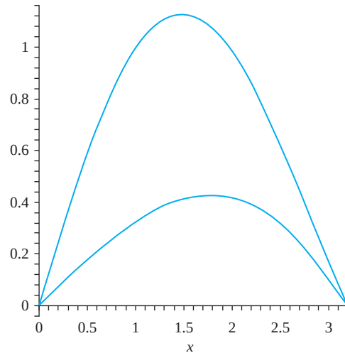
FIGURE 17.3 t = 0.8 .
