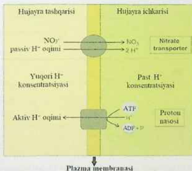
68-rasm. O'simlik hujayrasi plazma membranasi nitrat tashilishining sxematik diagrammasi. Marschner (2012).
