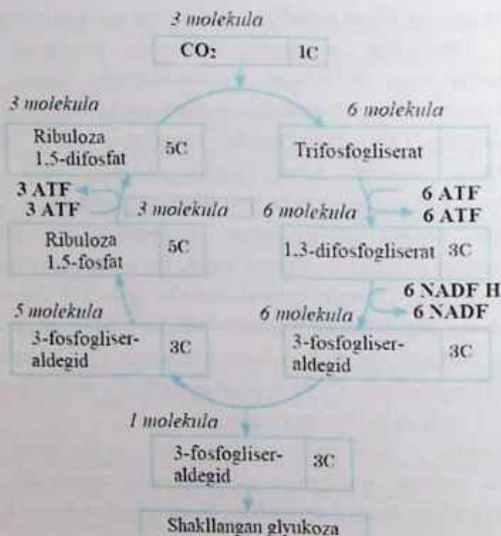
8-rasm. Calvin sikli.
