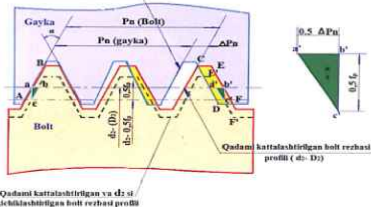
Gayka rezbasining nominal profili
