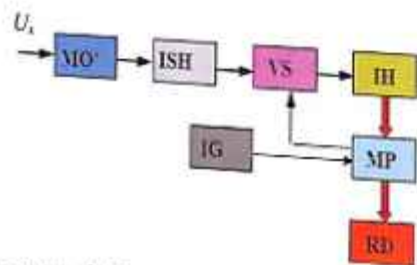
63-rasm. Mikroprotessorli chastotomer.
