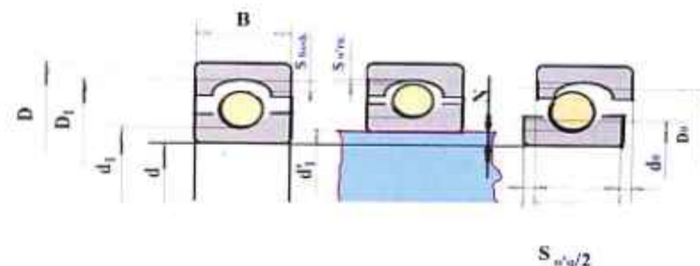
95-rasm. Dumalash podshipnidagi tirqishlar.
