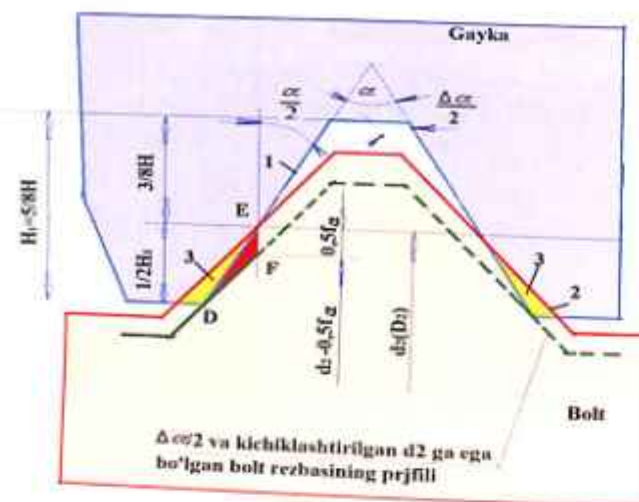
113-rasm. Profil burchagi yarmining og'ishi \frac{\Delta\alpha}{2} va diametral kompensatsiyasi f_a .
