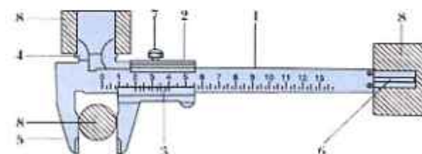
2-rasm. Shtangentsirkulning tuzilishi.
