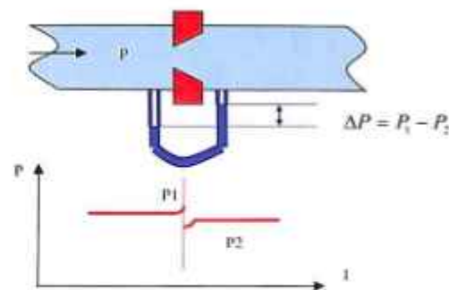
55-rasm. Bosim farqi o'zgaruvchan sarf o'lchagich
