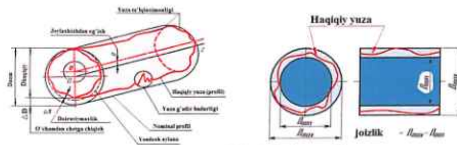
127-rasm. Silindrikdan og'ish.
