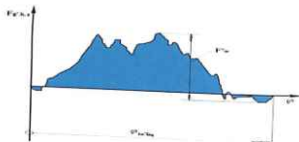
120-rasm. Tishli gildirak kinematik xatoligining egri chizig'i.
