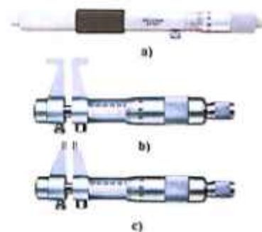
22-rasm. Mikrometrik icho'lchagichlar: a) NM 75-0.01 ISO 9002, b) NM 50-0.01 DIN 863, c) NM 30-0.01 DIN 863
