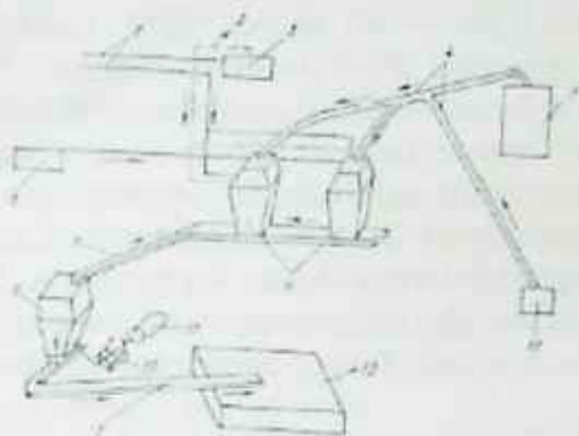
6-rasm. Trixodermin-5 biopreparati tayyorlanadigan qurilmaning texnologik sxemasi:
