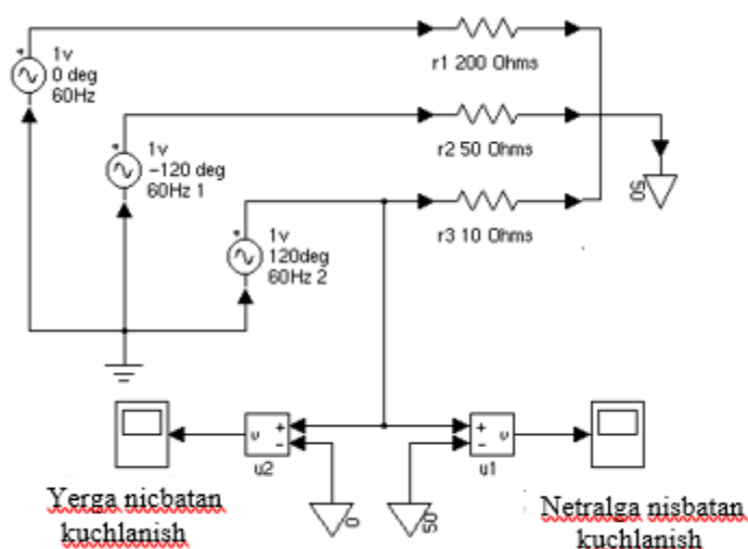
5.12-rasm. Netral blokidan foydalanishga misol
