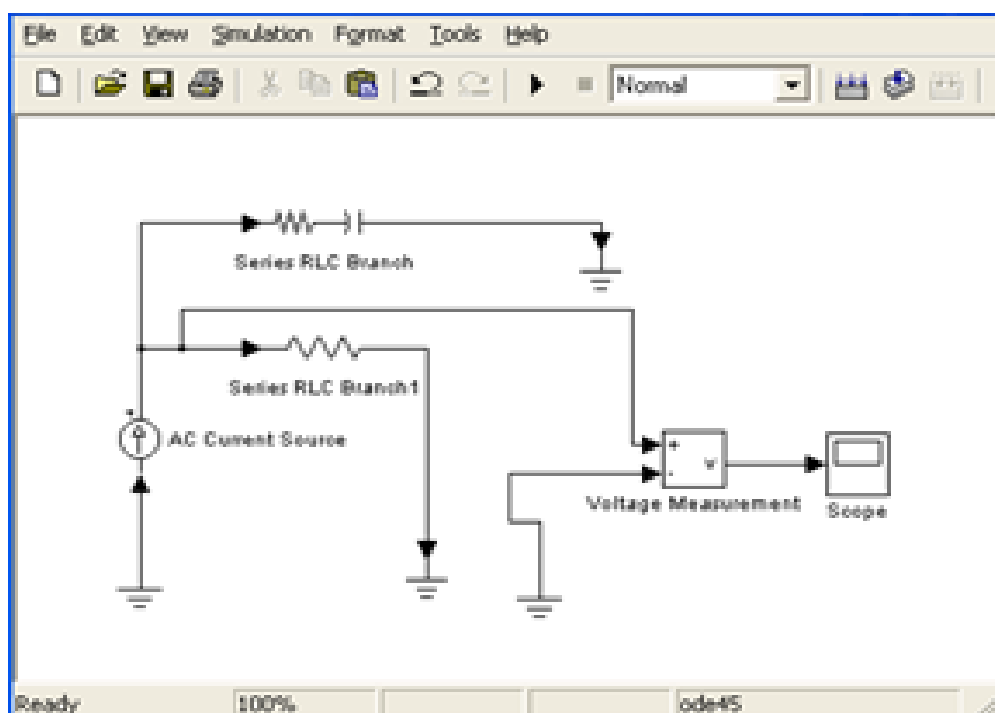
5.13-rasm. Ground blokidan foydalanishga misol
