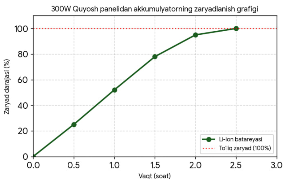
1-rasm. 300W Quyosh panelidan akkumulyatorning zaryadlanish dinamikasi
