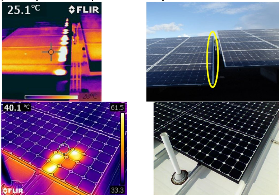
2-rasm. Kichik soylarning panel diodlariga ta‘hiri
