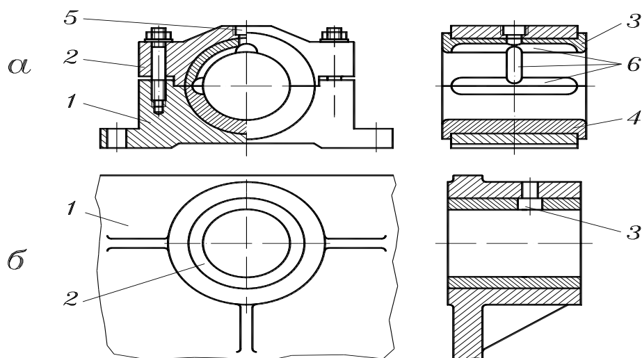
2-rasm. Sirpanish podshipniklarini tuzilishi
