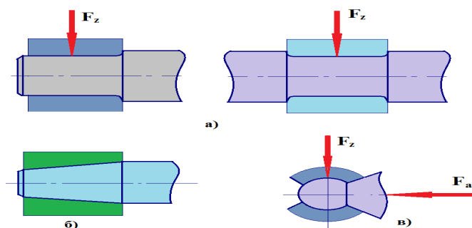
1- rasm. Sirpanish podshipnik turlari
