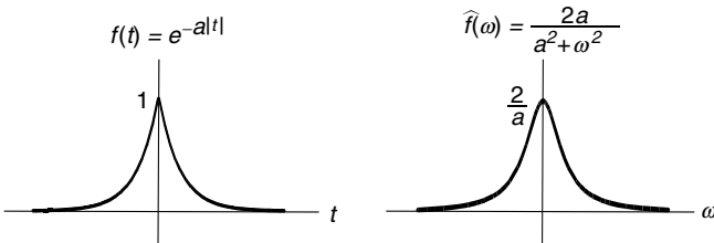
Fig. 2.6. The Fourier transform of an exponentially decaying function is Lorentz profile
