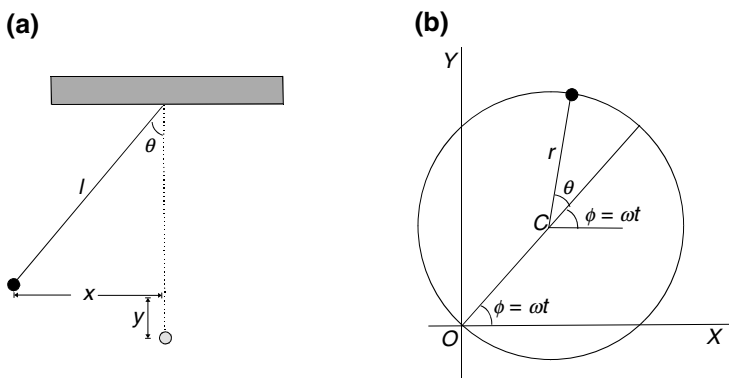
Fig. 7.14. Motions of pendulums
