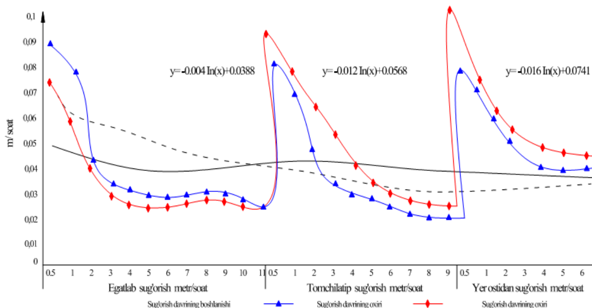
1-rasm. Egatlab va yer ostidan sug'orish usulida suvning shimilish jarayoni
