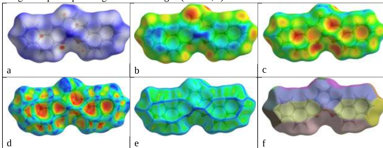
3-rasm. [\text{CuC}_{24}\text{H}_{18}\text{O}_2\text{N}_2] tarkibli kompleks birikmaning Hirshfeld yuzasi tahlilining sirt xususiyatlari tasviri: (a) d_{\text{norm}} ; (b) d_i ; (c) d_e ; (d) Shakl Indeksi; (e) Egrilik; (f) qismlarga bo'linish
