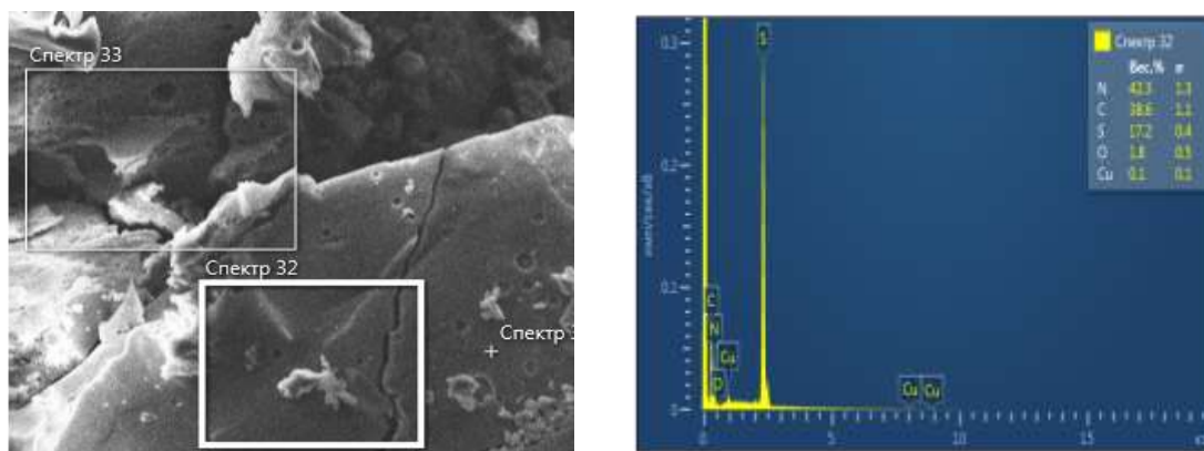
Figure 2. \text{Cu}^{2+} of DMT+M ionite ion scanning electron microscopic image of the surface of the complex compound with and the amount of elements in it, %
