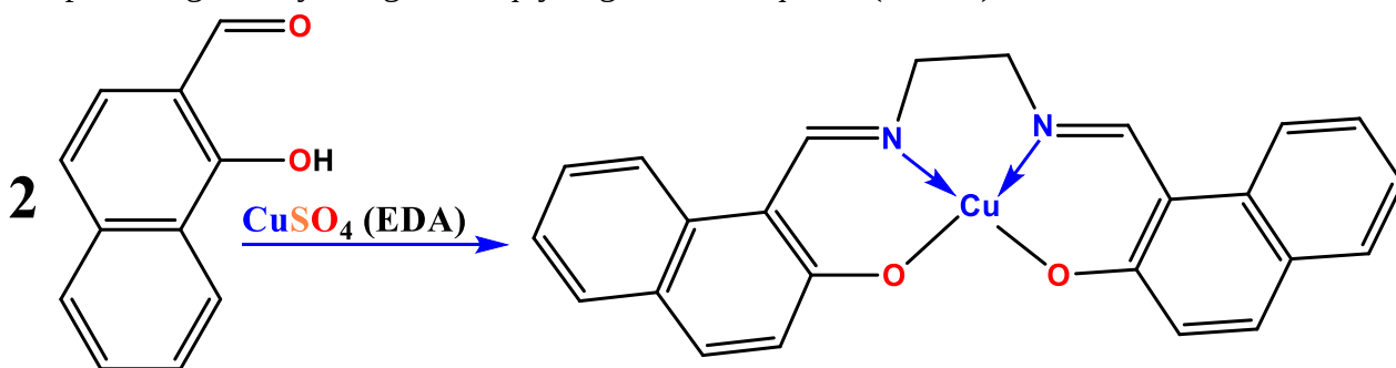
1-rasm. [\text{CuC}_{24}\text{H}_{18}\text{O}_2\text{N}_2] tarkibli kompleksining sintez sxemasi
