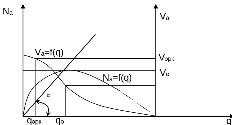
2.14-rasm. Transport oqimining asosiy diagrammasi.
