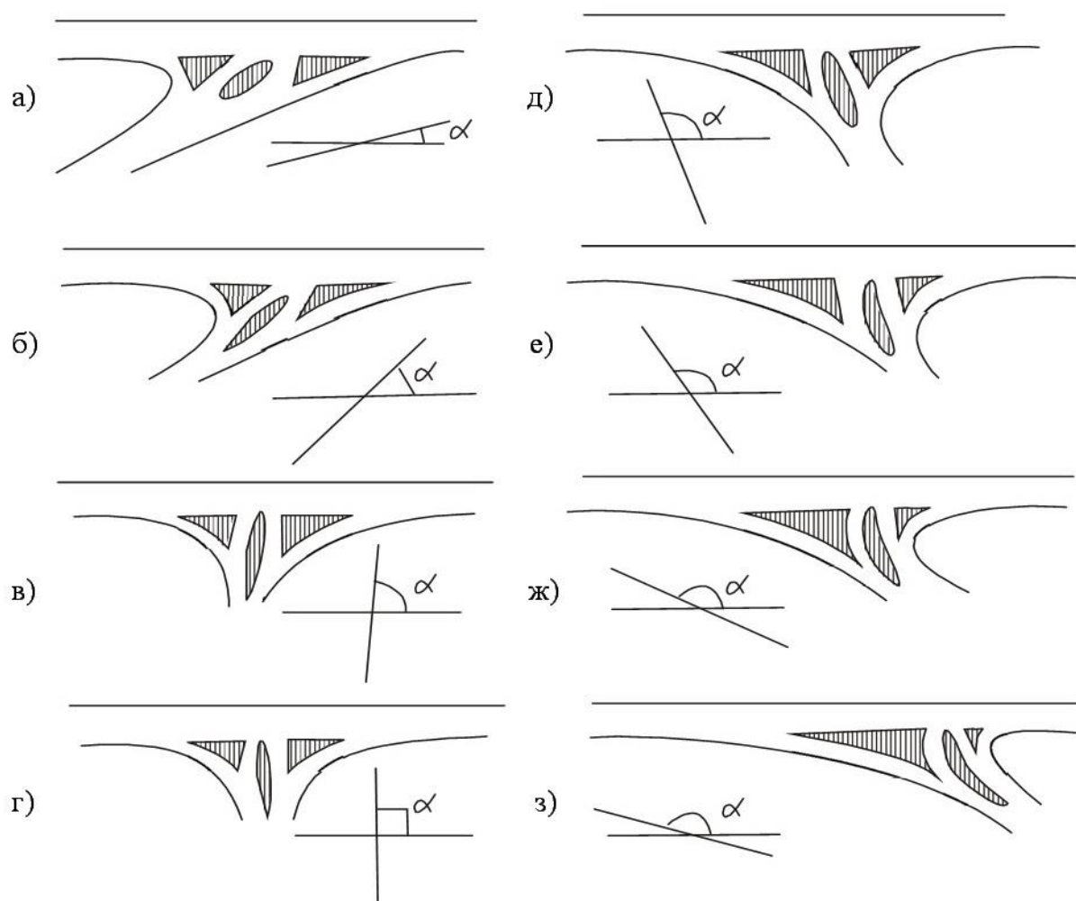
6.5-rasm. Tutashish burchagiga nisbatan planirovkaning o'zgarishi:
